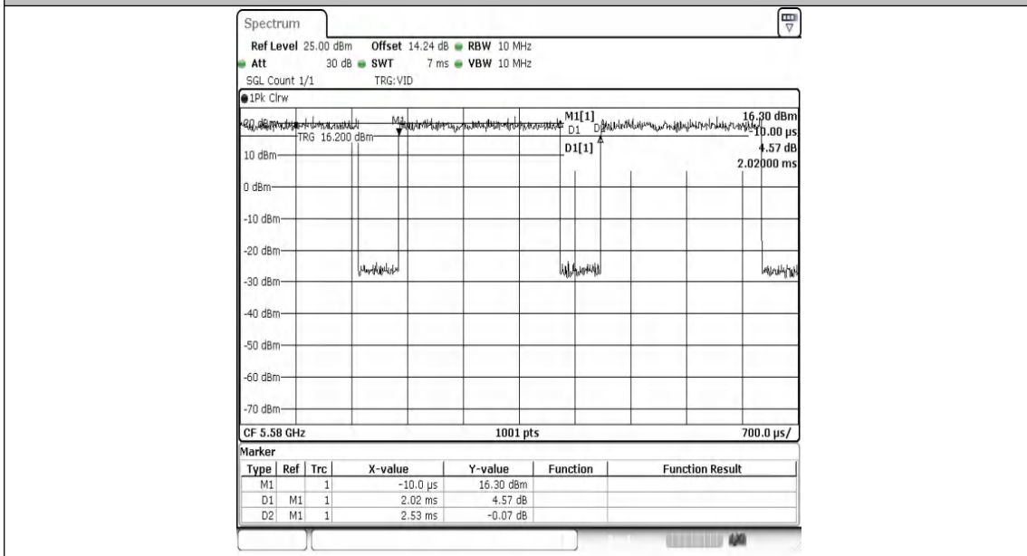
NTNV-802.11a-Ant1-5580
