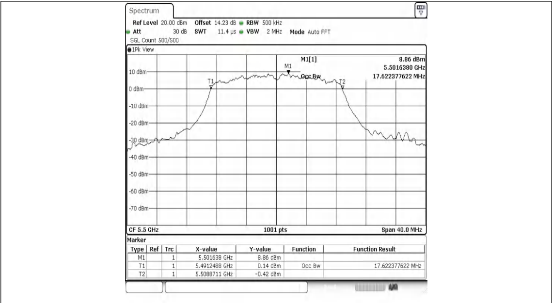
802.11n (HT20)-Ant1-5500
