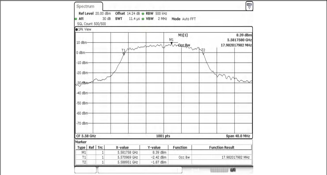
802.11n (HT20)-Ant1-5580
