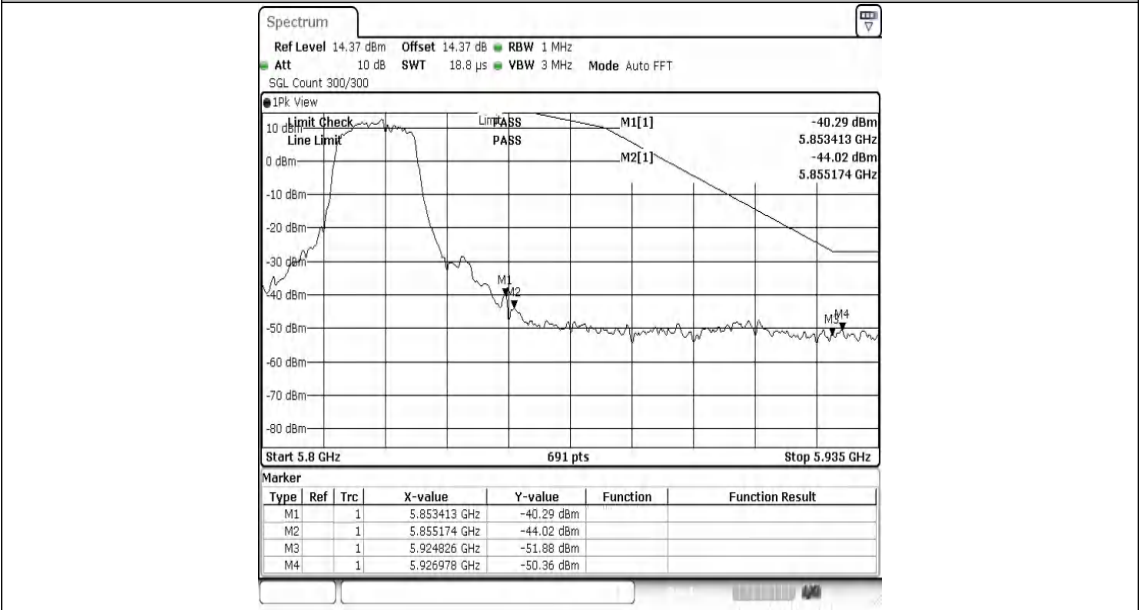
802.11n (HT20)-Ant1-5825-PASS
