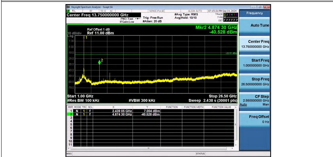
802.11b-Ant1-2437-1000~26500-PASS
