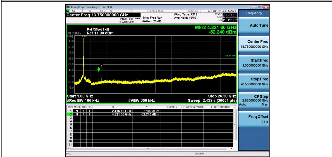
802.11g-Ant1-2412-1000~26500-PASS
