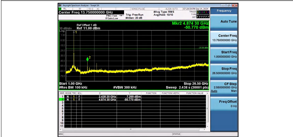
802.11g-Ant1-2437-1000~26500-PASS
