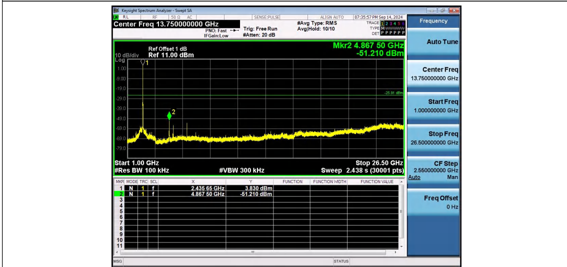
802.11n(HT20)SISO-Ant1-2437-1000~26500-PASS
