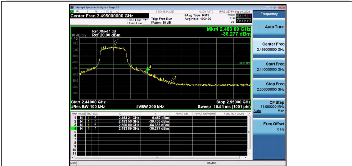
802.11g-Ant1-2462-PASS
