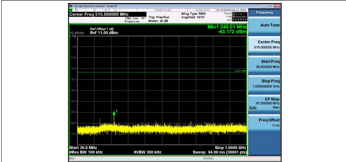
802.11b-Ant1-2437-30~1000-PASS
