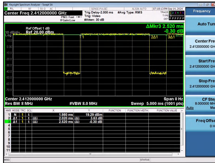
NTNV-802.11g-Ant1-2412
