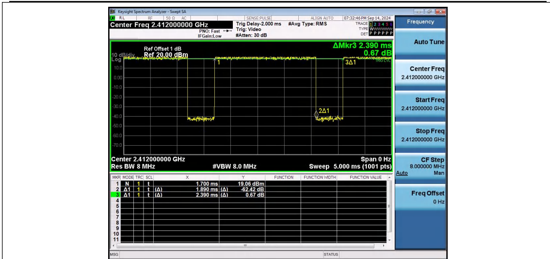
NTNV-802.11n(HT20)SISO-Ant1-2412
