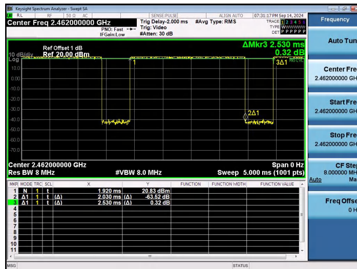
NTNV-802.11g-Ant1-2462
