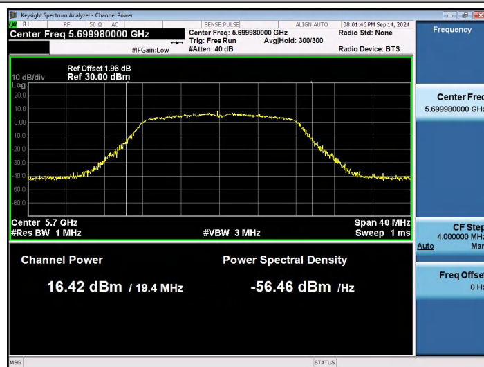
802.11a-Ant1-5700-PASS
