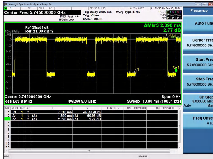
NTNV-802.11n(HT20)SISO-Ant1-5745
