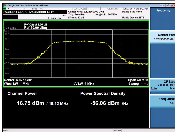
802.11a-Ant1-5825-PASS
