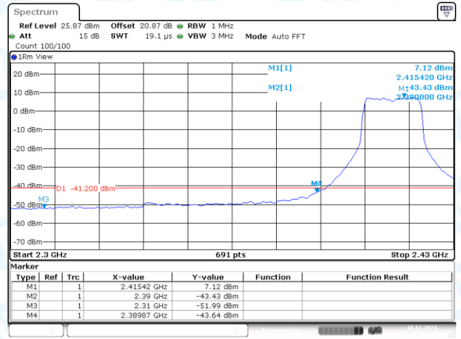
11G-Ant1-2412-PASS
