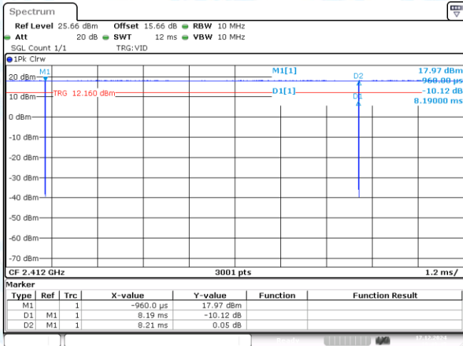
NTNV-11B-Ant1-2412
