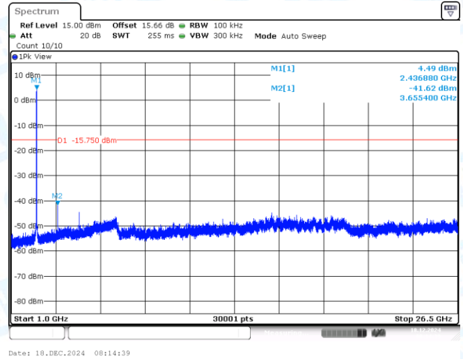
11B-Ant1-2437-1000~26500-PASS
