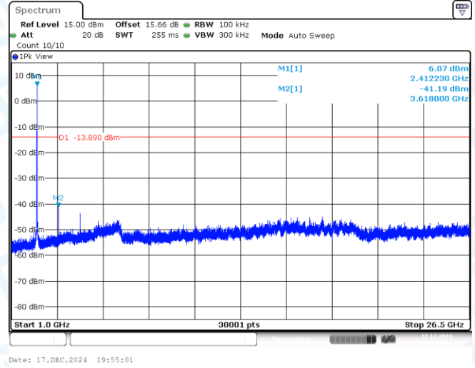
11B-Ant1-2412-1000~26500-PASS
