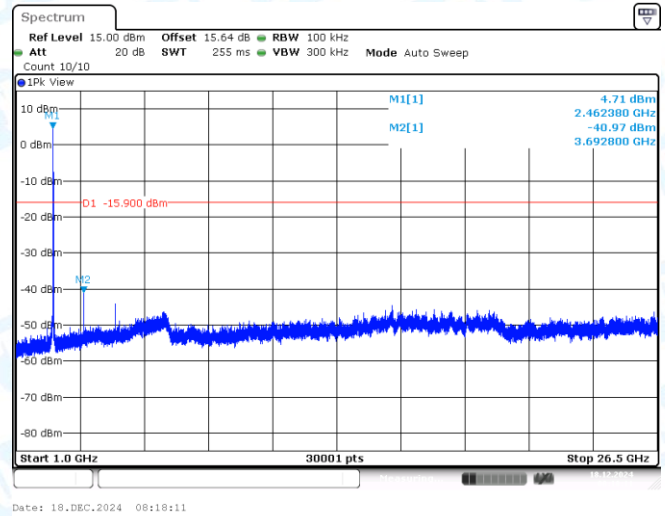
11B-Ant1-2462-1000~26500-PASS
