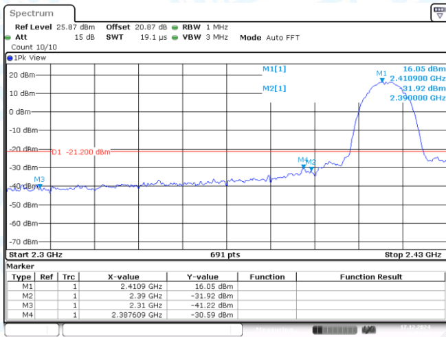
11B-Ant1-2412-PASS
