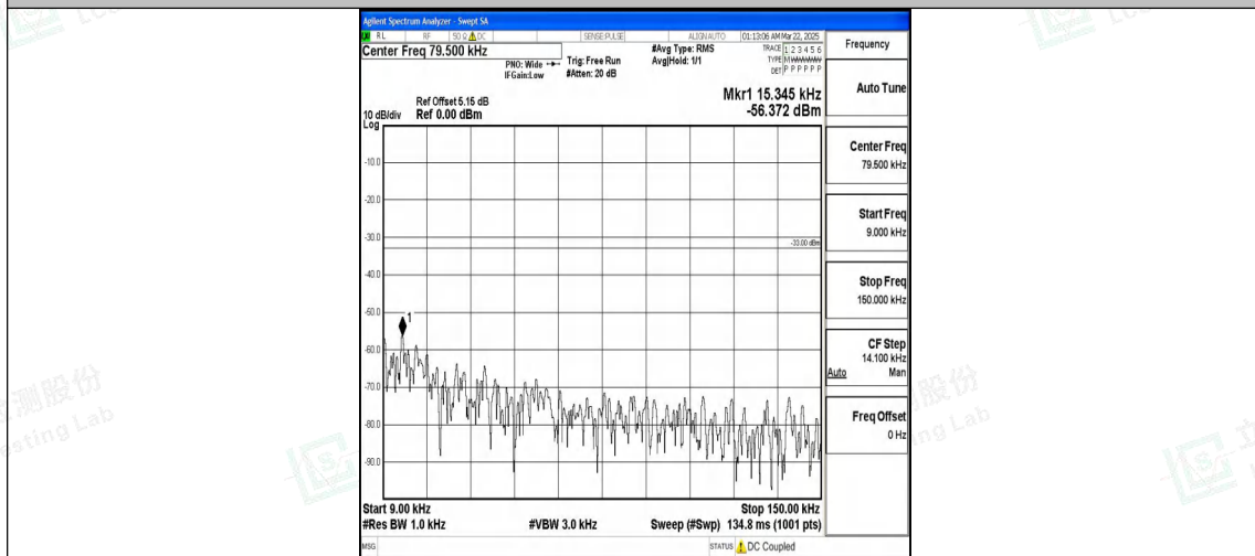
Band26_3MHz_QPSK_26740_1RB#0_0.009~0.15_0.009~0.15
