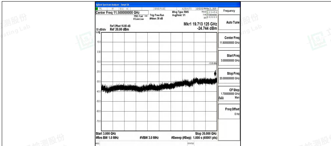
Band25_20MHz_QPSK_26365_1RB#0_3000~20000_3000~20000
