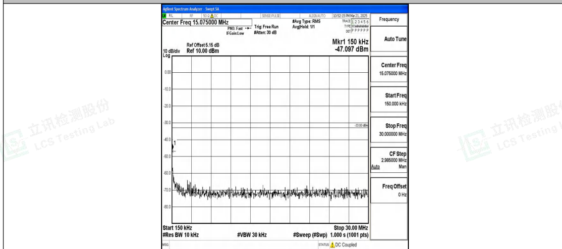
Band25_20MHz_16QAM_26365_1RB#0_0.15~30_0.15~30
