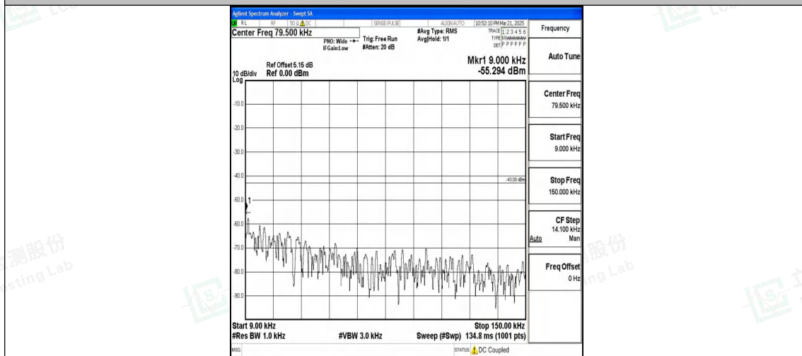
Band25_20MHz_16QAM_26365_1RB#0_0.009~0.15_0.009~0.15
