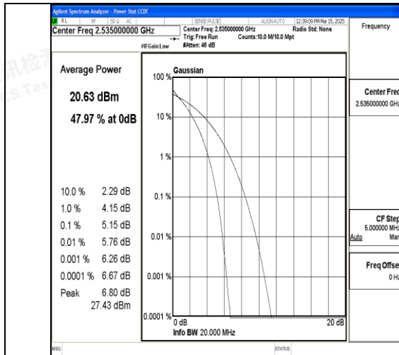
Band7-20MHz-QPSK-21100-100RB#0-PASS
