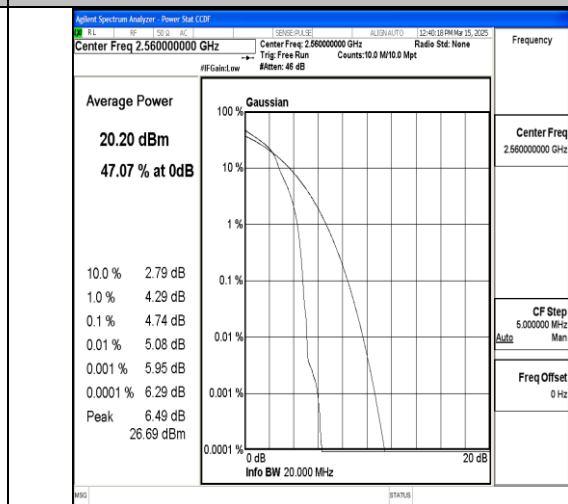
Band7-20MHz-16QAM-21350-1RB#0-PASS
