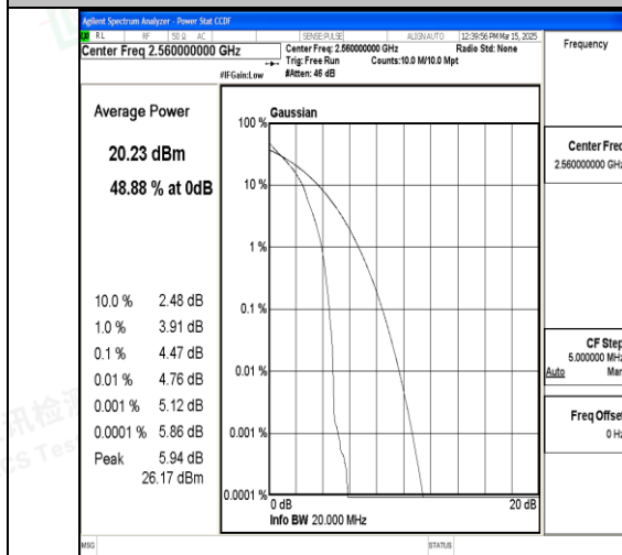
Band7-20MHz-QPSK-21350-1RB#0-PASS
