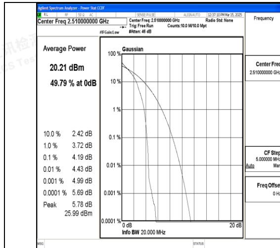
Band7-20MHz-QPSK-20850-1RB#0-PASS
