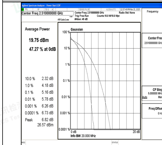
Band7-20MHz-QPSK-20850-100RB#0-PASS
