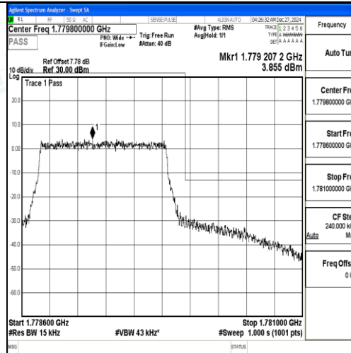
Band66_1.4MHz_16QAM_132665_6RB#0
