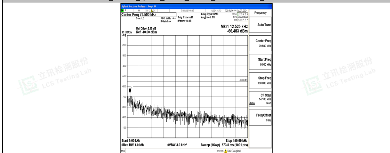
Band41_10MHz_16QAM_39700_1RB#0_0.009~0.15_0.009~0.15
