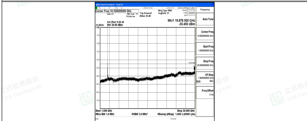
Band41_15MHz_QPSK_39725_1RB#0_1000~20000_1000~20000
