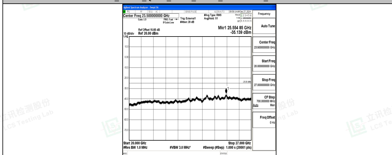
Band41_10MHz_QPSK_41540_1RB#0_20000~27000_20000~27000
