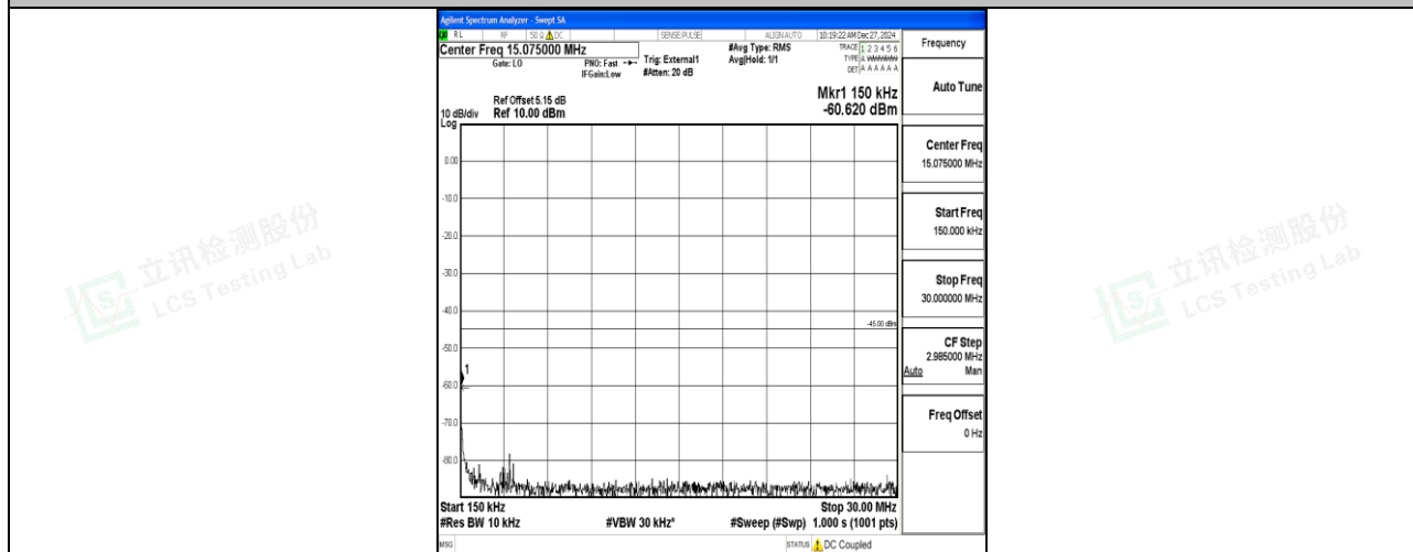
Band41_15MHz_QPSK_39725_1RB#0_0.15~30_0.15~30
