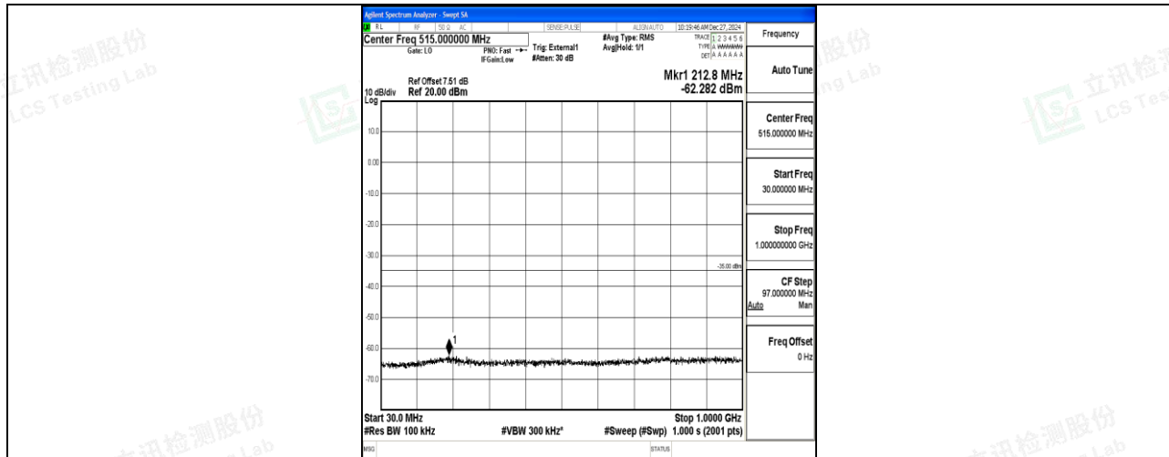
Band41_15MHz_QPSK_39725_1RB#0_30~1000_30~1000
