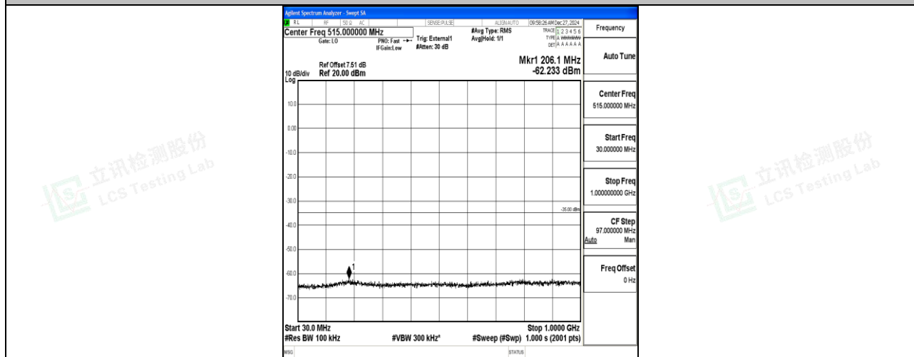
Band41_10MHz_QPSK_41540_1RB#0_30~1000_30~1000
