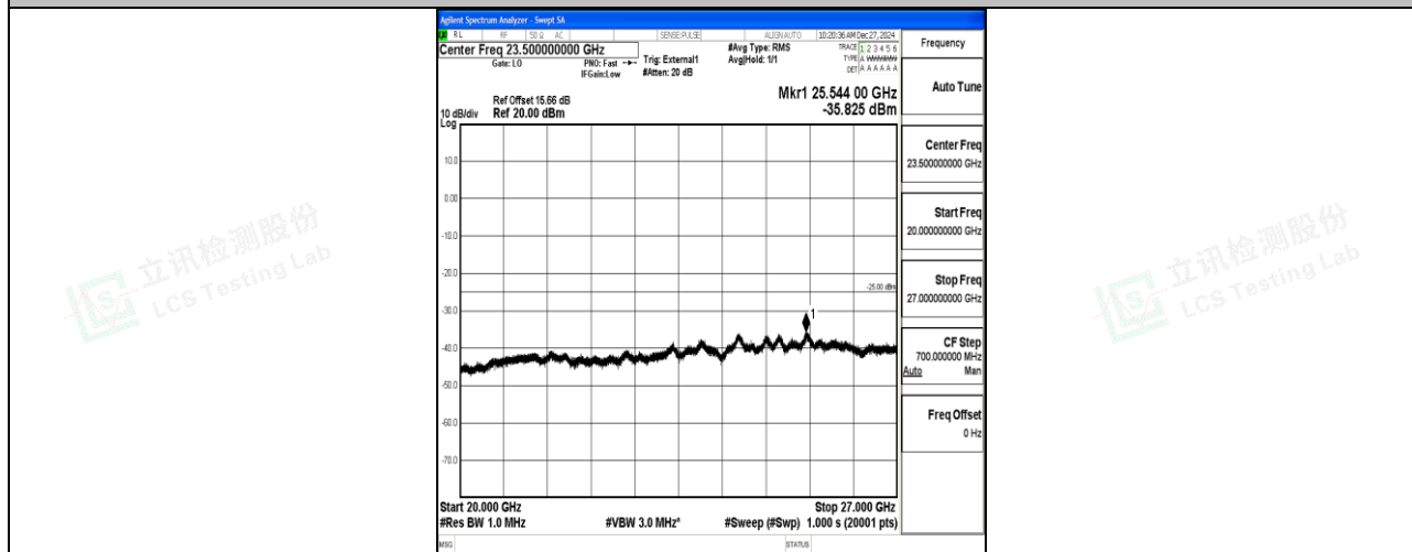
Band41_15MHz_QPSK_39725_1RB#0_20000~27000_20000~27000
