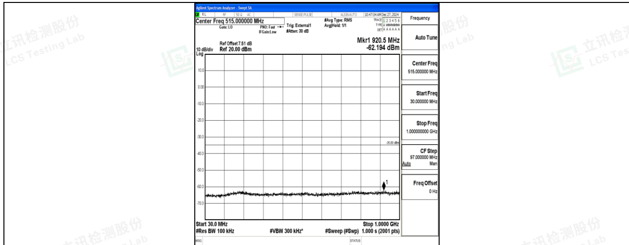
Band41_20MHz_QPSK_39750_1RB#0_30~1000_30~1000
