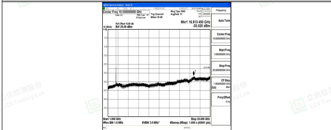
Band41_20MHz_QPSK_39750_1RB#0_1000~20000_1000~20000
