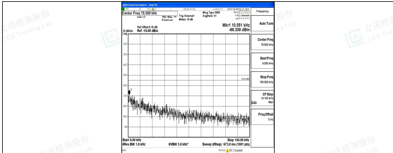
Band41_10MHz_QPSK_41540_1RB#0_0.009~0.15_0.009~0.15
