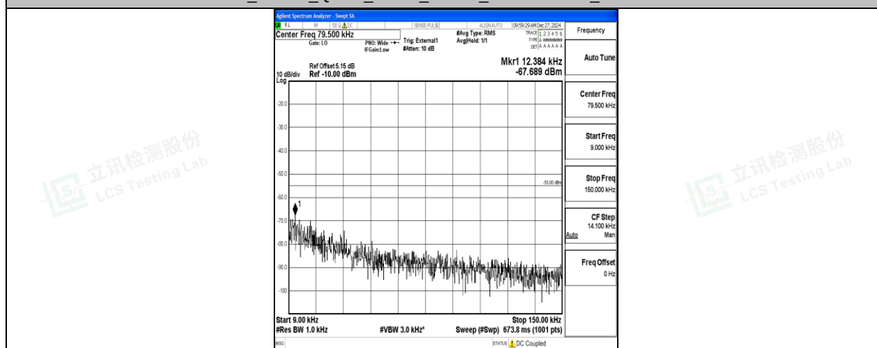
Band41_10MHz_16QAM_41540_1RB#0_0.009~0.15_0.009~0.15
