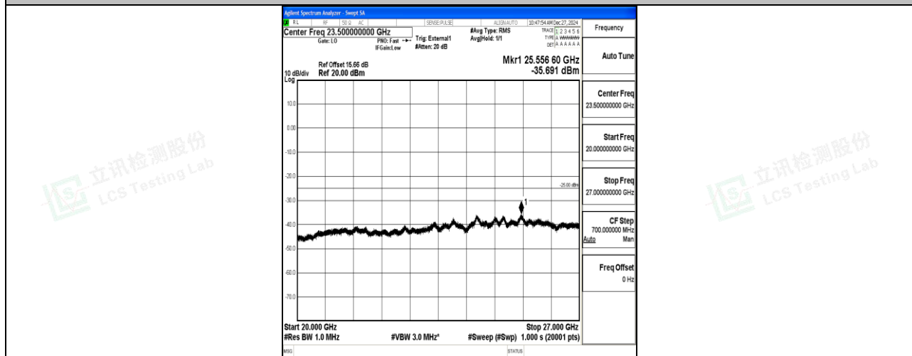
Band41_20MHz_QPSK_39750_1RB#0_20000~27000_20000~27000
