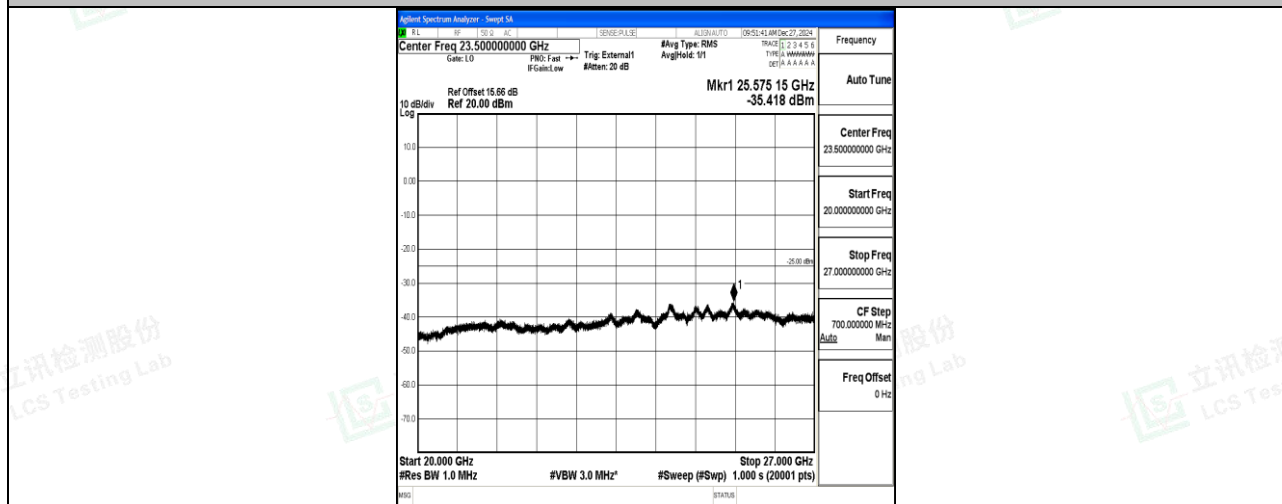
Band41_10MHz_QPSK_39700_1RB#0_20000~27000_20000~27000
