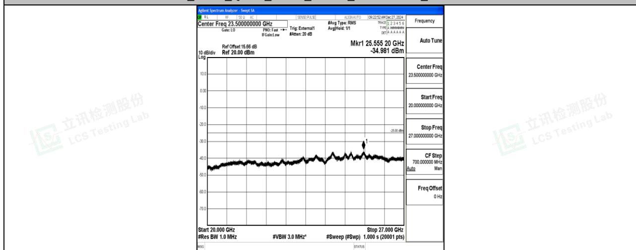
Band41_5MHz_QPSK_40620_1RB#0_20000~27000_20000~27000
