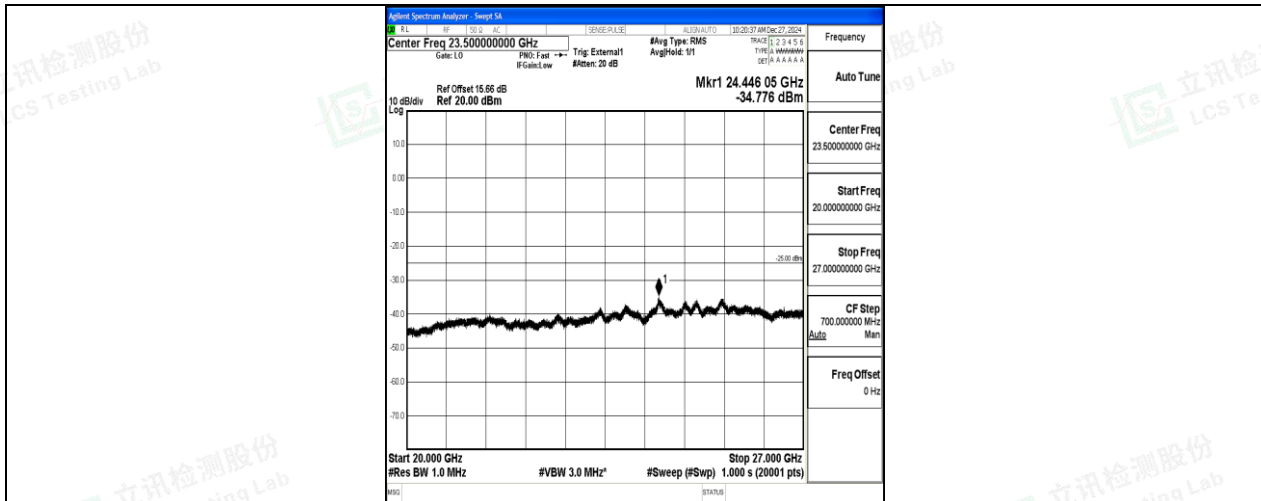
Band38_20MHz_16QAM_37850_1RB#0_20000~27000_20000~27000
