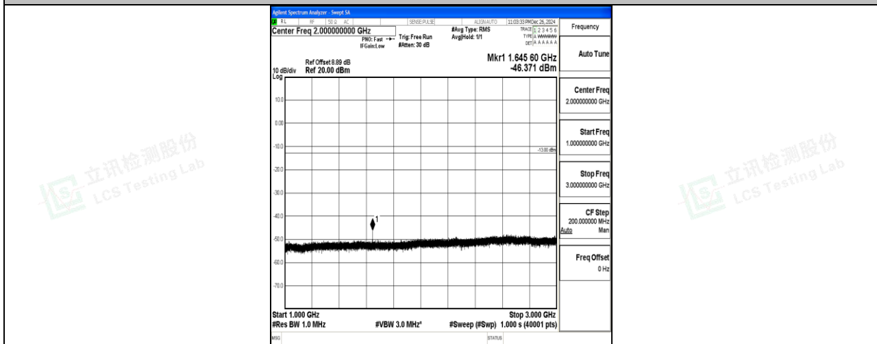
Band26_1.4MHz_16QAM_26783_1RB#0_1000~3000_1000~3000
