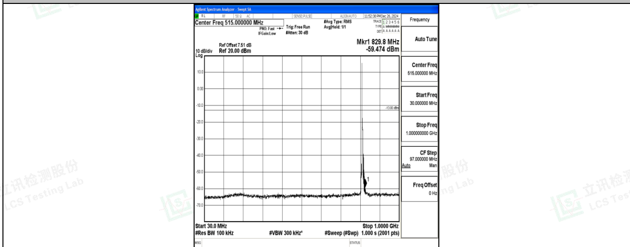
Band26_5MHz_QPSK_26715_1RB#0_30~1000_30~1000
