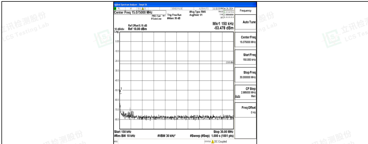
Band26_3MHz_16QAM_26775_1RB#0_0.15~30_0.15~30
