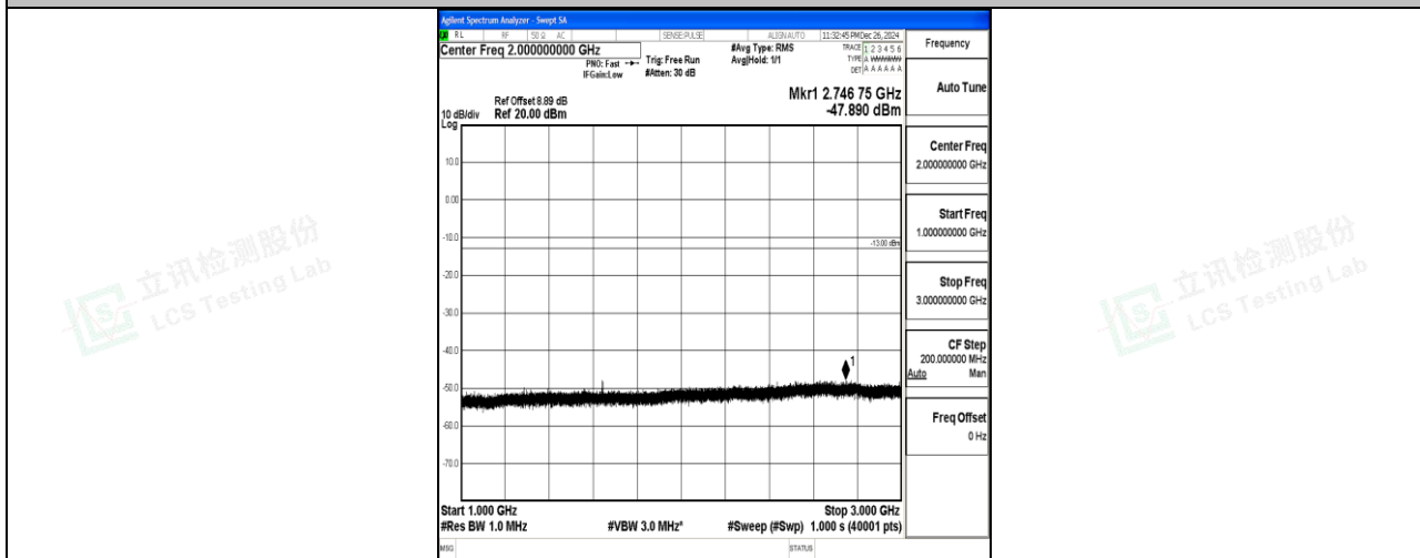
Band26_3MHz_16QAM_26775_1RB#0_1000~3000_1000~3000
