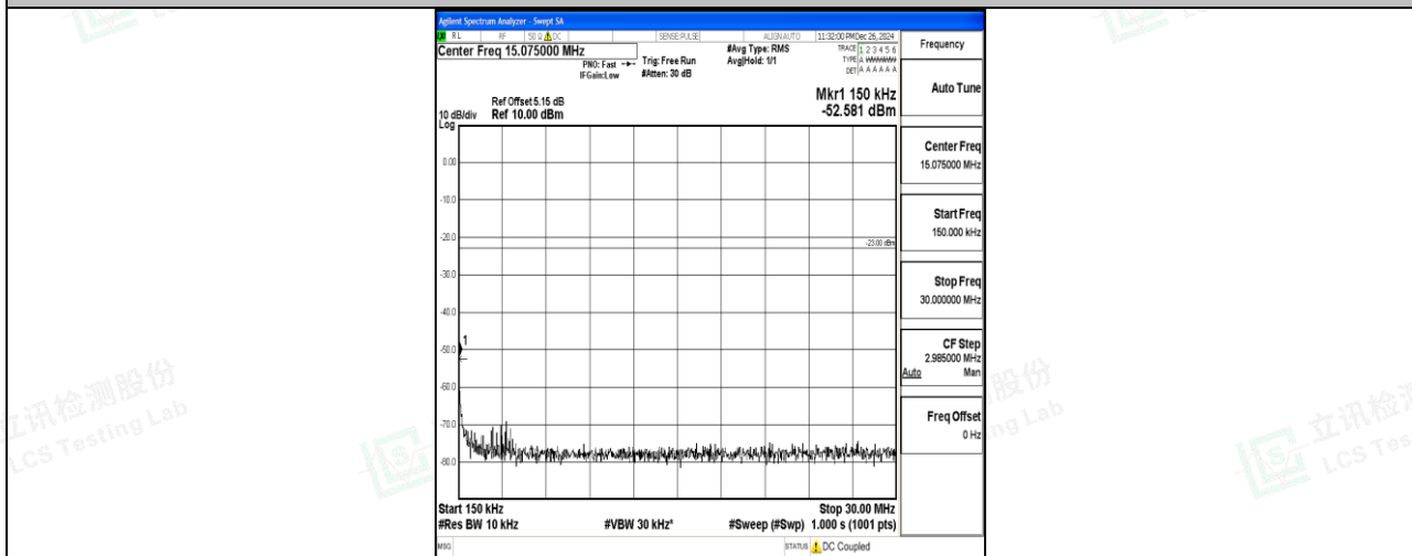
Band26_3MHz_QPSK_26775_1RB#0_0.15~30_0.15~30
