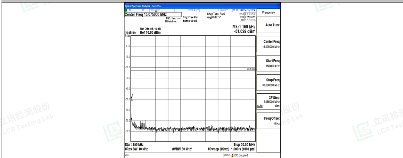
Band26_3MHz_16QAM_26705_1RB#0_0.15~30_0.15~30
