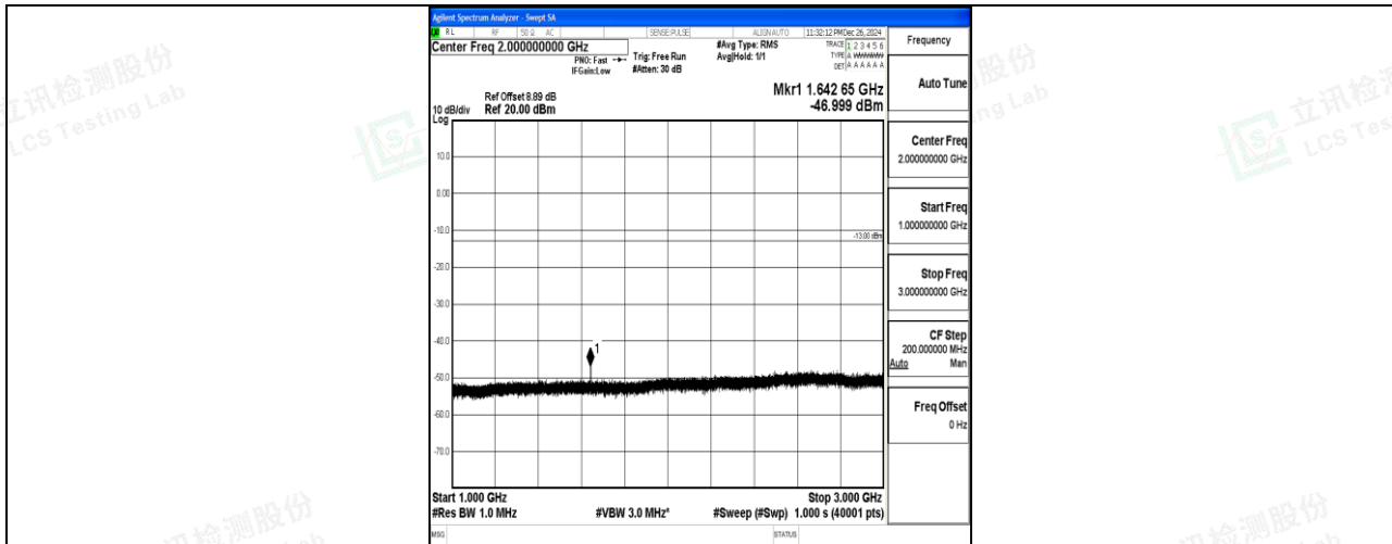
Band26_3MHz_QPSK_26775_1RB#0_1000~3000_1000~3000
