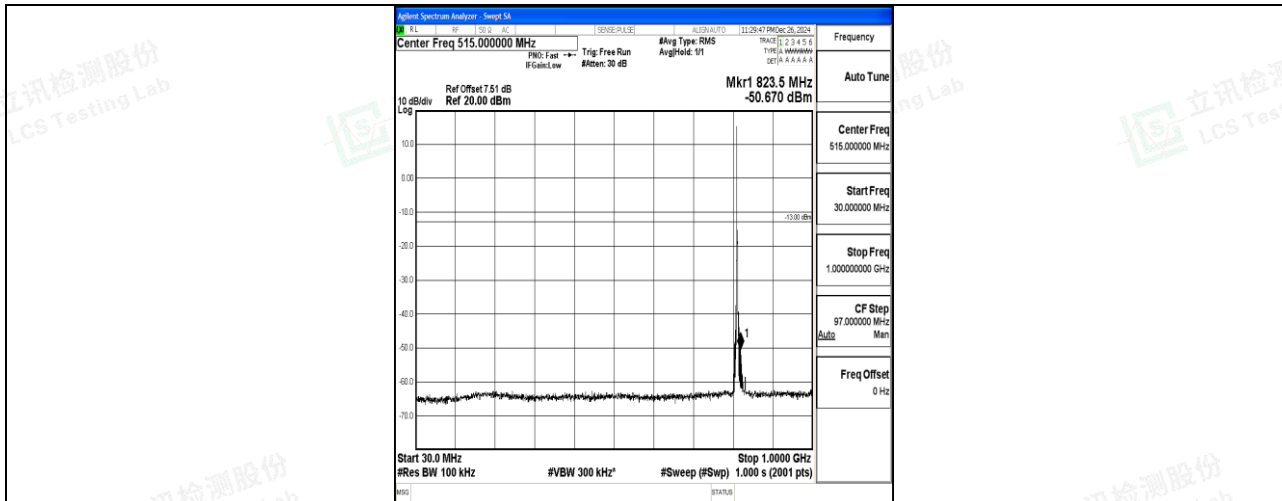
Band26_3MHz_QPSK_26705_1RB#0_30~1000_30~1000
