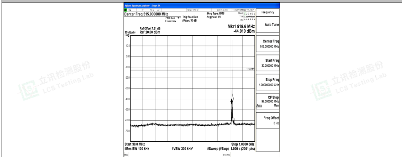
Band26_1.4MHz_QPSK_26783_1RB#0_30~1000_30~1000
