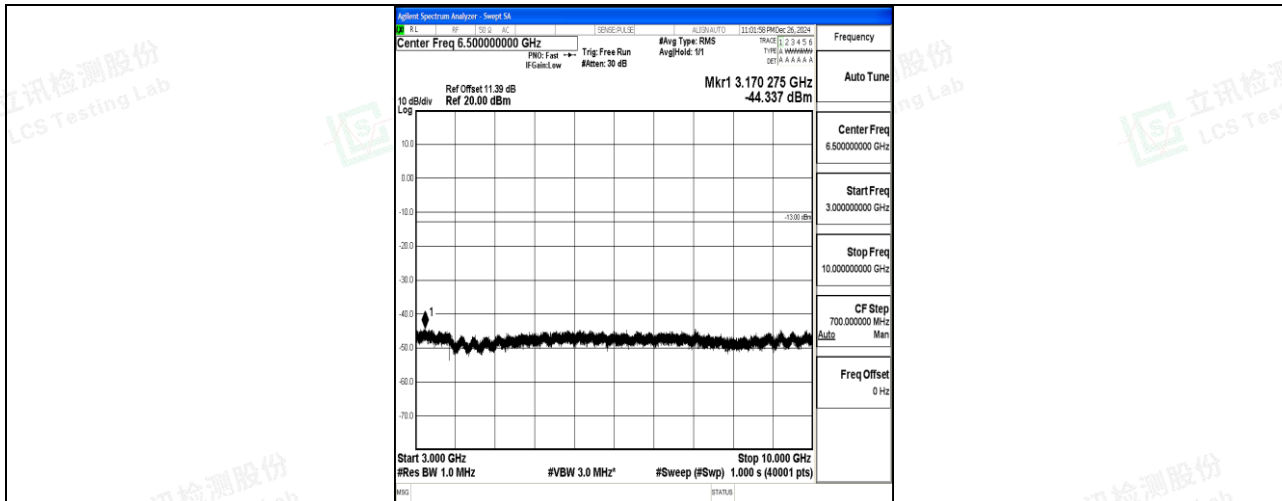
Band26_1.4MHz_QPSK_26740_1RB#0_3000~10000_3000~10000
