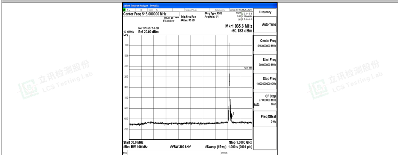
Band26_5MHz_16QAM_26765_1RB#0_30~1000_30~1000
