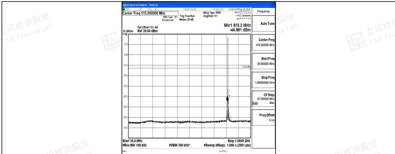
Band26_1.4MHz_16QAM_26740_1RB#0_30~1000_30~1000
