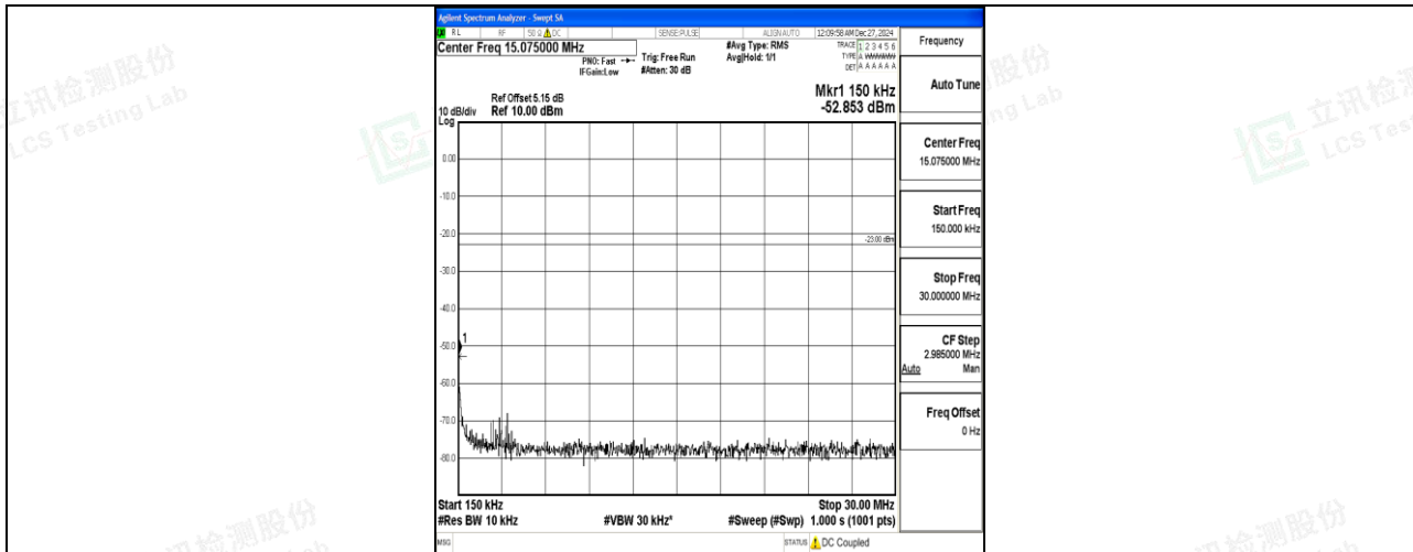
Band26_10MHz_QPSK_26740_1RB#0_0.15~30_0.15~30
