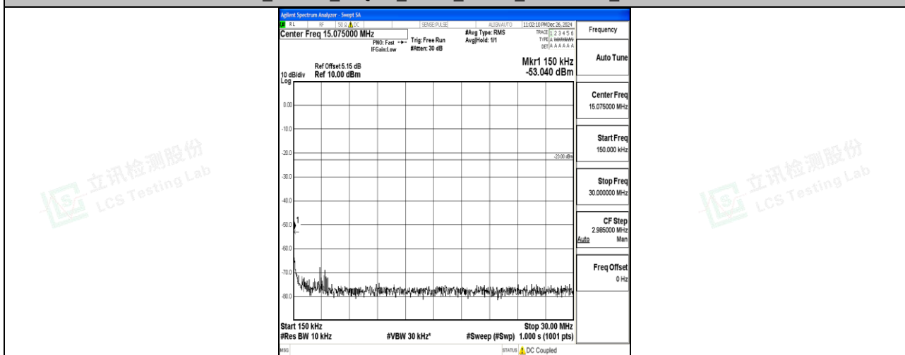
Band26_1.4MHz_16QAM_26740_1RB#0_0.15~30_0.15~30
