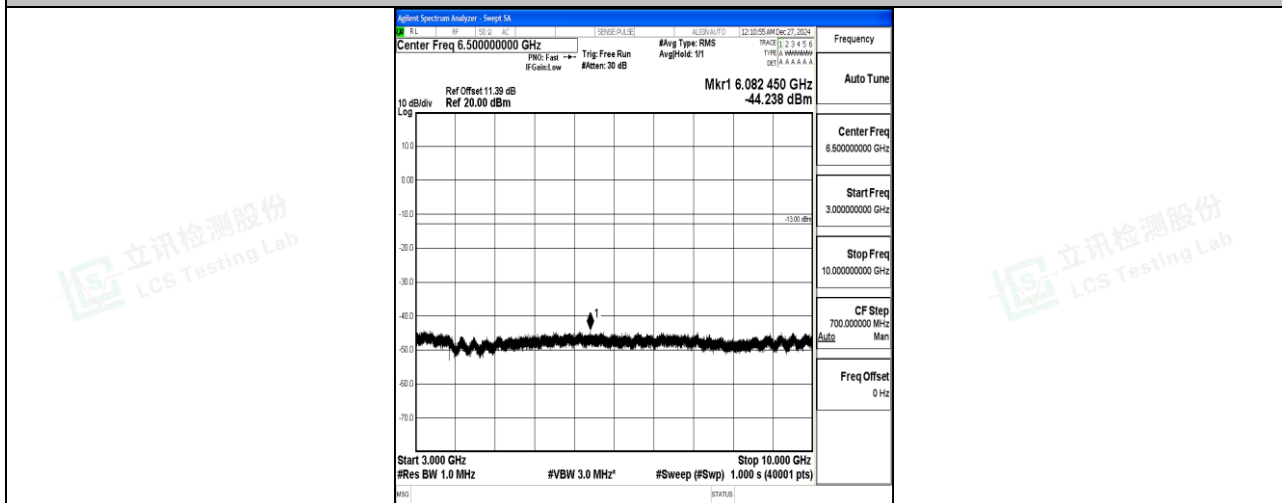
Band26_10MHz_16QAM_26740_1RB#0_3000~10000_3000~10000
