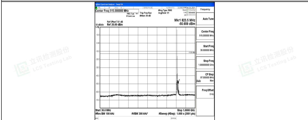
Band26_3MHz_16QAM_26705_1RB#0_30~1000_30~1000
