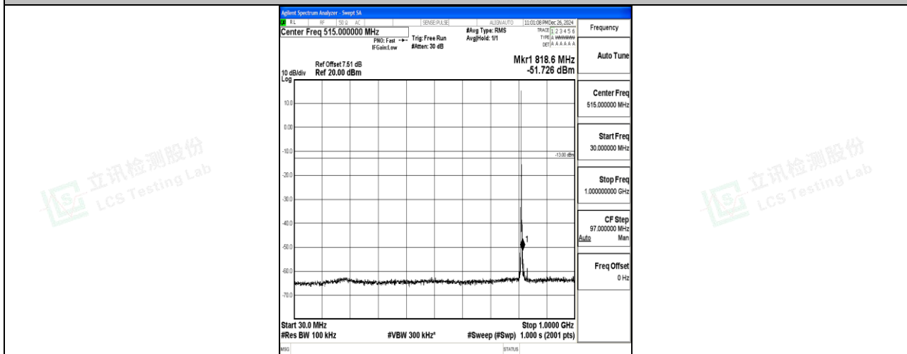
Band26_1.4MHz_16QAM_26697_1RB#0_30~1000_30~1000
