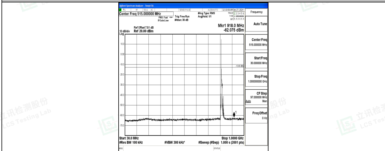
Band26_10MHz_QPSK_26740_1RB#0_30~1000_30~1000
