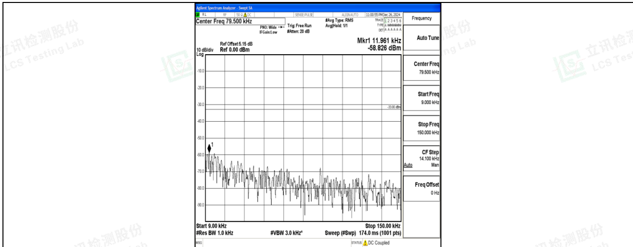
Band26_1.4MHz_16QAM_26697_1RB#0_0.009~0.15_0.009~0.15
