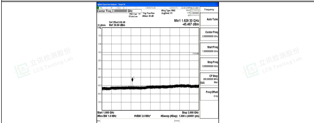
Band26_10MHz_QPSK_26740_1RB#0_1000~3000_1000~3000
