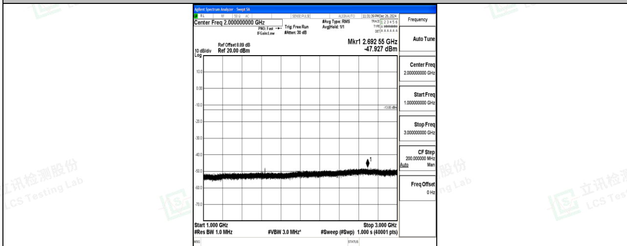
Band26_3MHz_16QAM_26740_1RB#0_1000~3000_1000~3000
