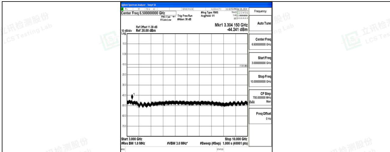
Band26_3MHz_16QAM_26775_1RB#0_3000~10000_3000~10000
