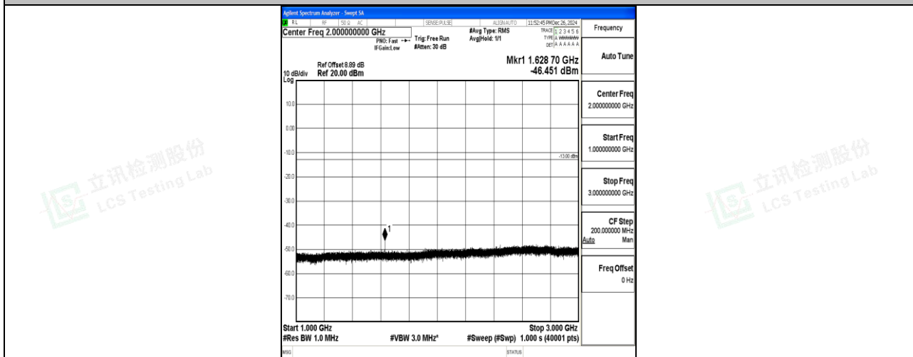
Band26_5MHz_QPSK_26715_1RB#0_1000~3000_1000~3000
