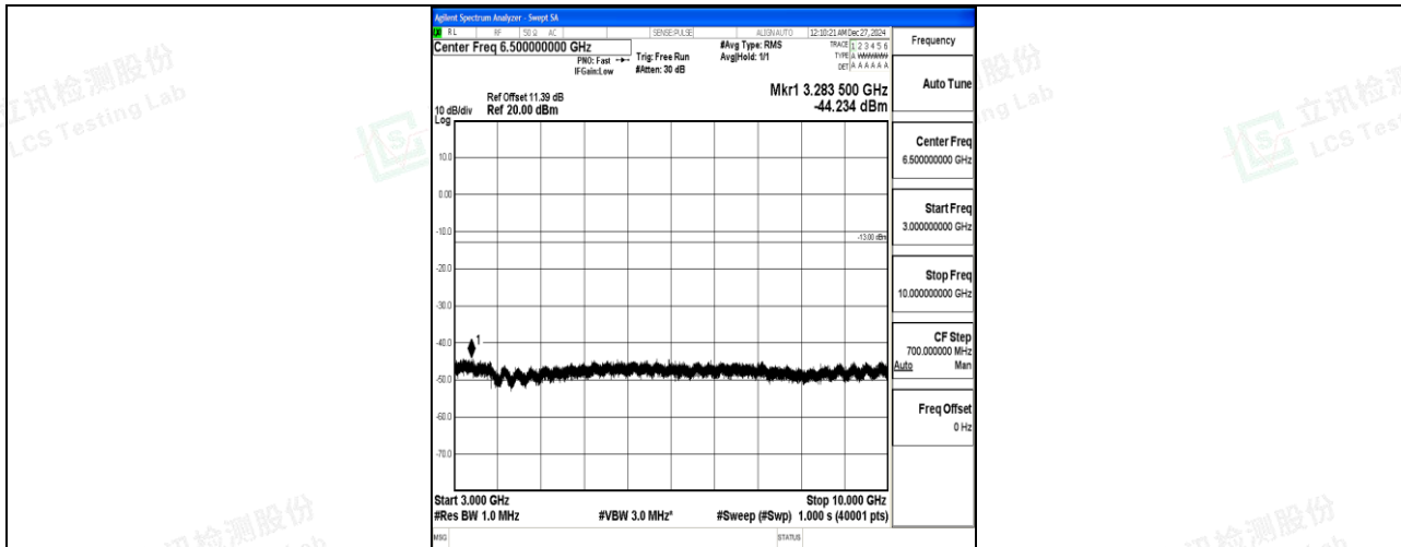
Band26_10MHz_QPSK_26740_1RB#0_3000~10000_3000~10000
