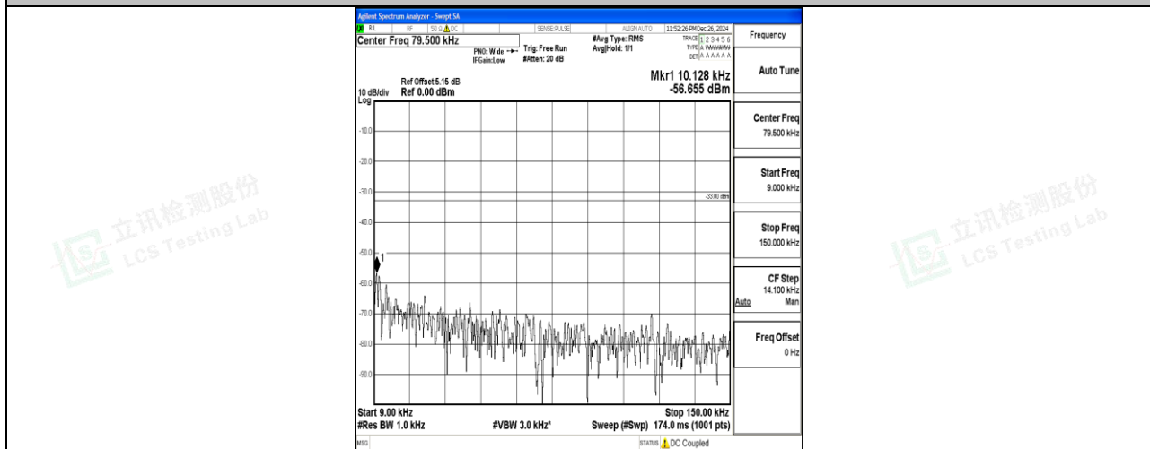
Band26_5MHz_QPSK_26715_1RB#0_0.009~0.15_0.009~0.15
