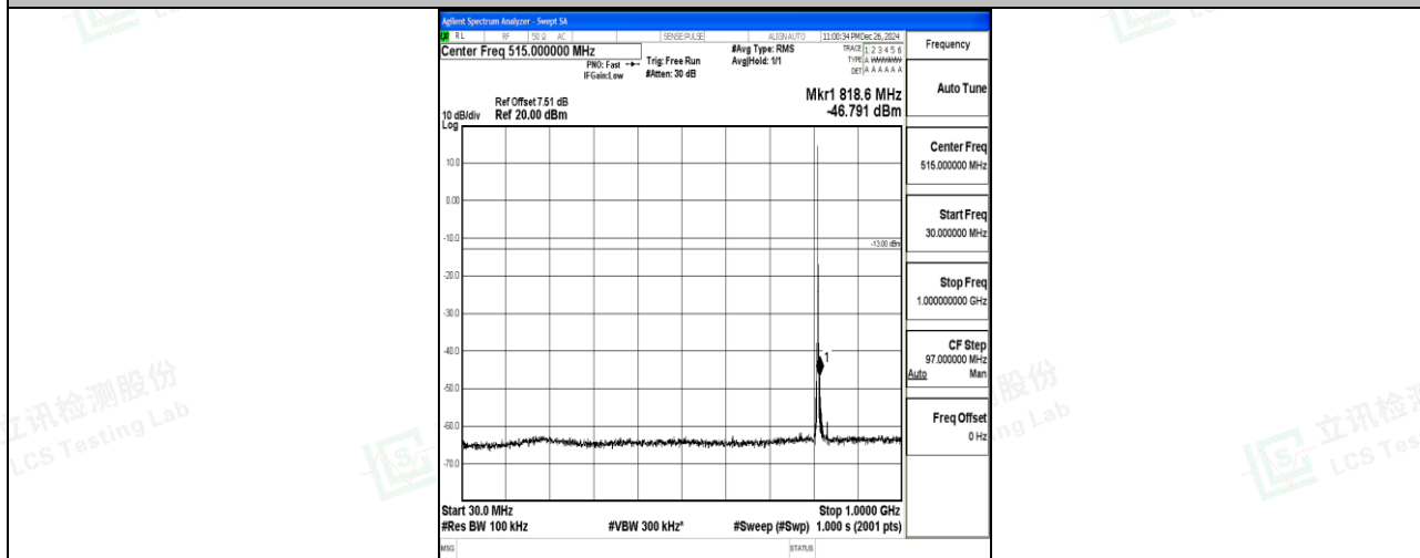
Band26_1.4MHz_QPSK_26697_1RB#0_30~1000_30~1000
