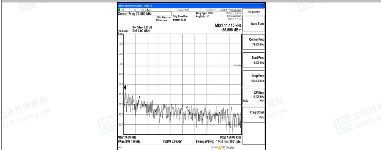
Band26_1.4MHz_16QAM_26740_1RB#0_0.009~0.15_0.009~0.15
