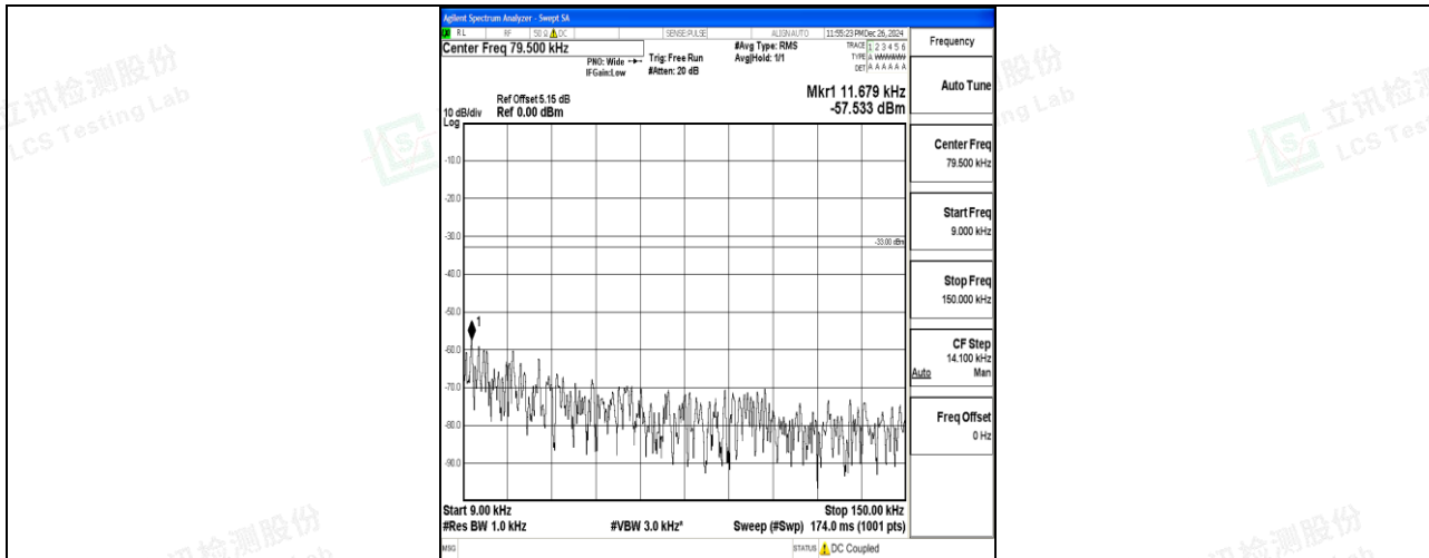
Band26_5MHz_16QAM_26765_1RB#0_0.009~0.15_0.009~0.15
