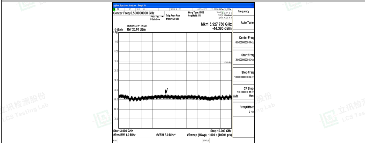
Band26_1.4MHz_QPSK_26783_1RB#0_3000~10000_3000~10000
