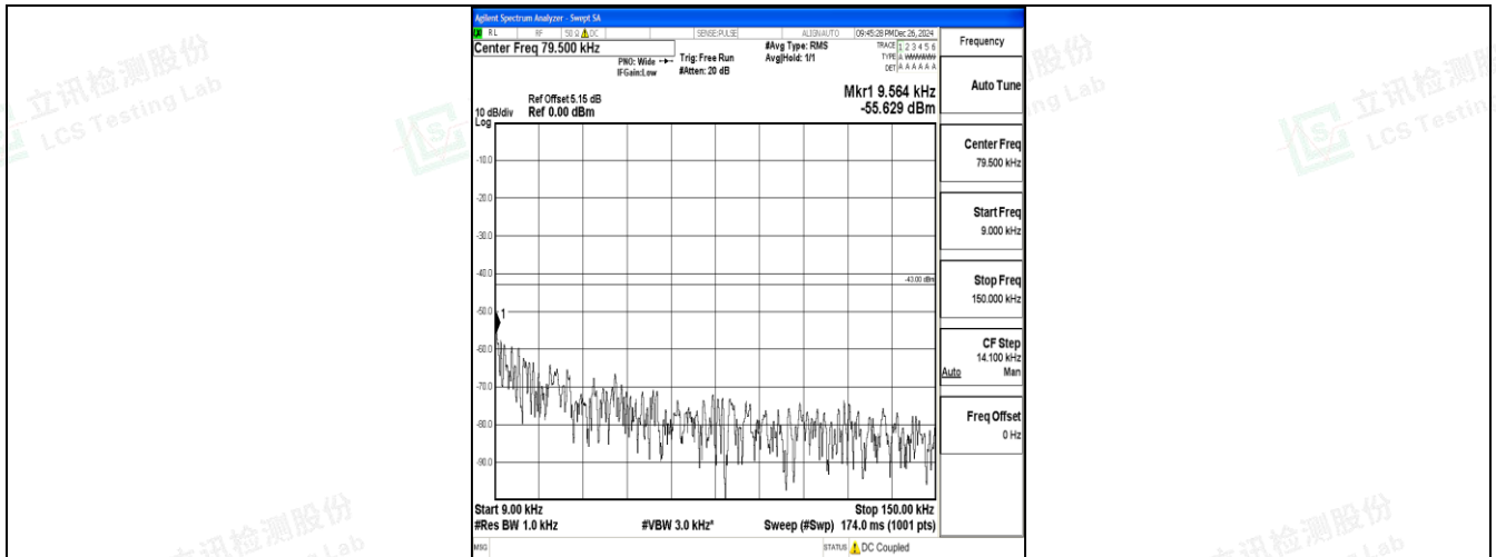
Band25_5MHz_QPSK_26365_1RB#0_0.009~0.15_0.009~0.15
