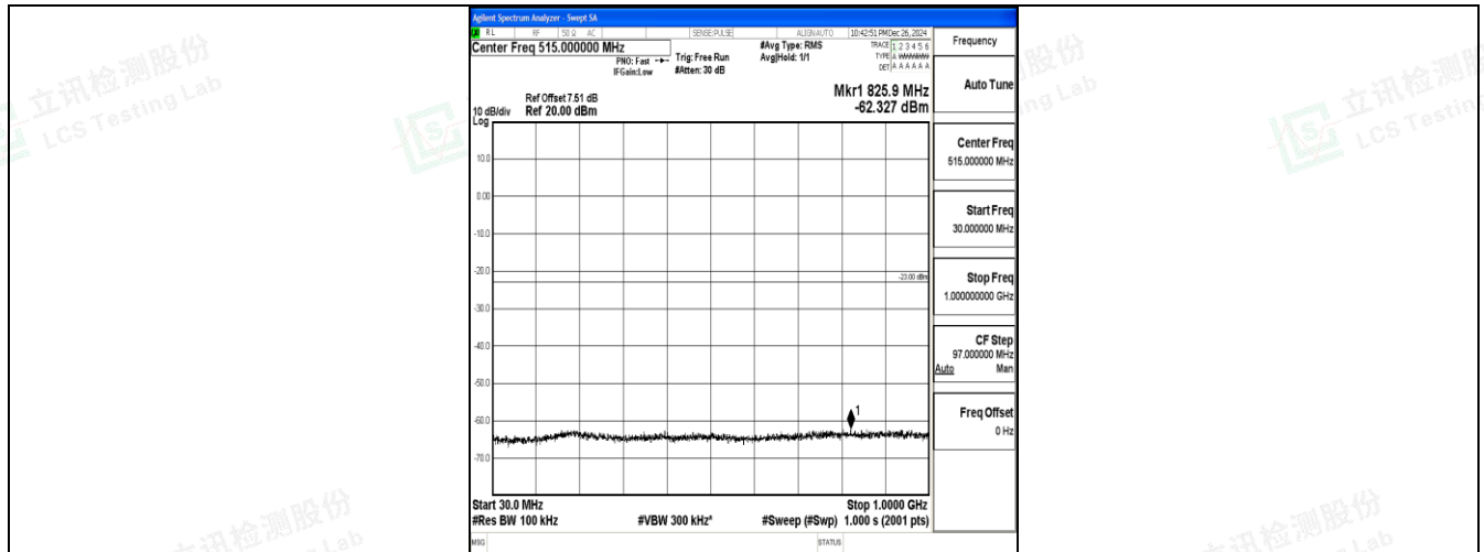
Band25_20MHz_16QAM_26140_1RB#0_30~1000_30~1000
