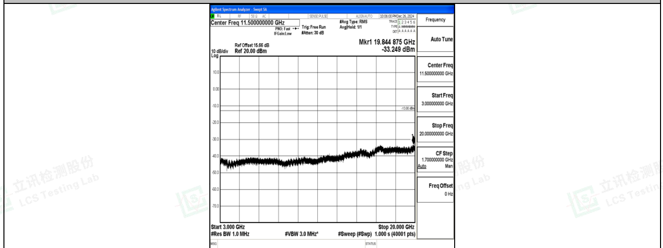
Band25_10MHz_QPSK_26365_1RB#0_3000~20000_3000~20000
