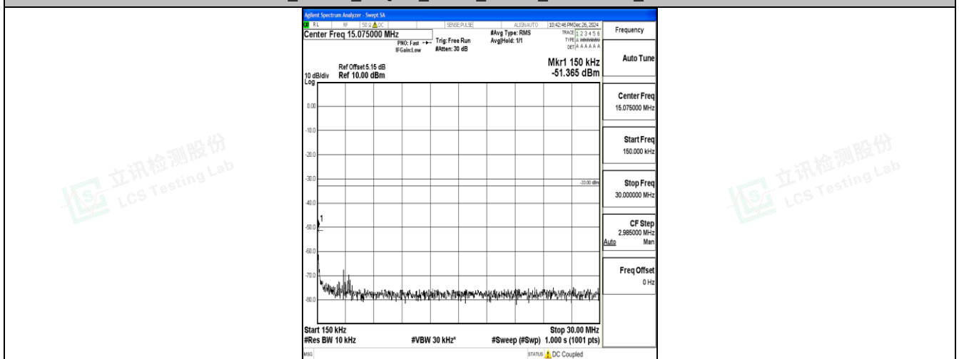
Band25_20MHz_16QAM_26140_1RB#0_0.15~30_0.15~30
