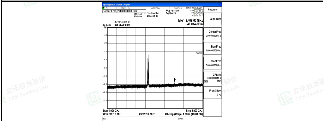
Band25_10MHz_16QAM_26090_1RB#0_1000~3000_1000~3000
