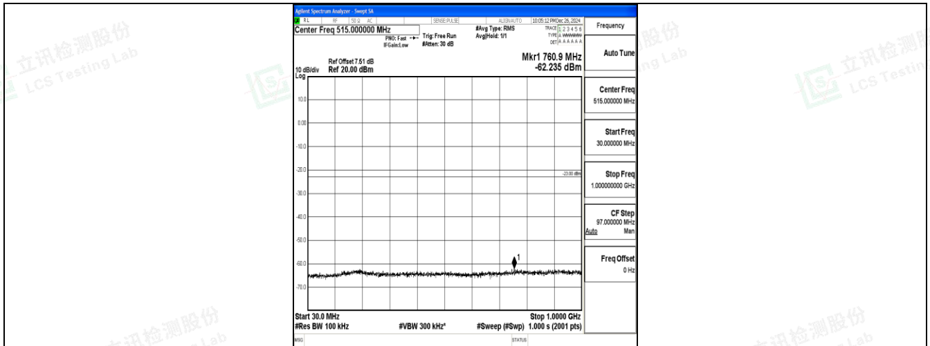
Band25_10MHz_16QAM_26090_1RB#0_30~1000_30~1000
