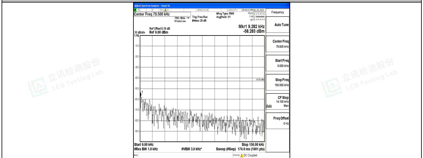
Band25_5MHz_16QAM_26365_1RB#0_0.009~0.15_0.009~0.15
