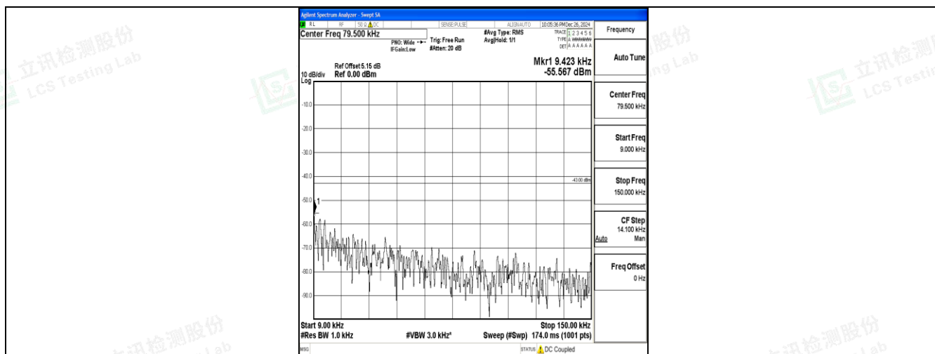
Band25_10MHz_QPSK_26365_1RB#0_0.009~0.15_0.009~0.15
