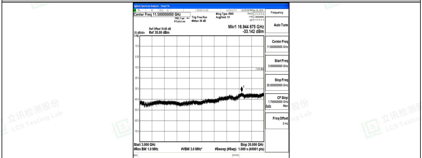
Band25_15MHz_QPSK_26365_1RB#0_3000~20000_3000~20000
