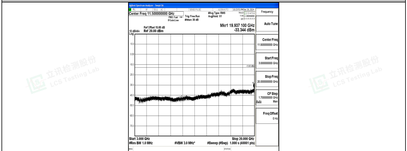
Band25_15MHz_QPSK_26115_1RB#0_3000~20000_3000~20000
