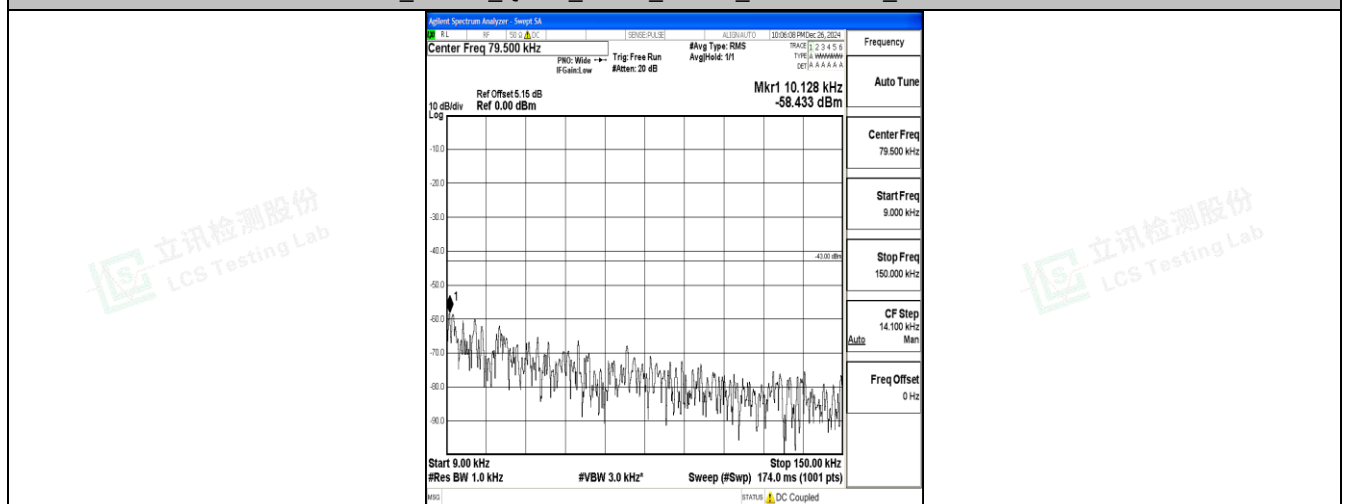
Band25_10MHz_16QAM_26365_1RB#0_0.009~0.15_0.009~0.15
