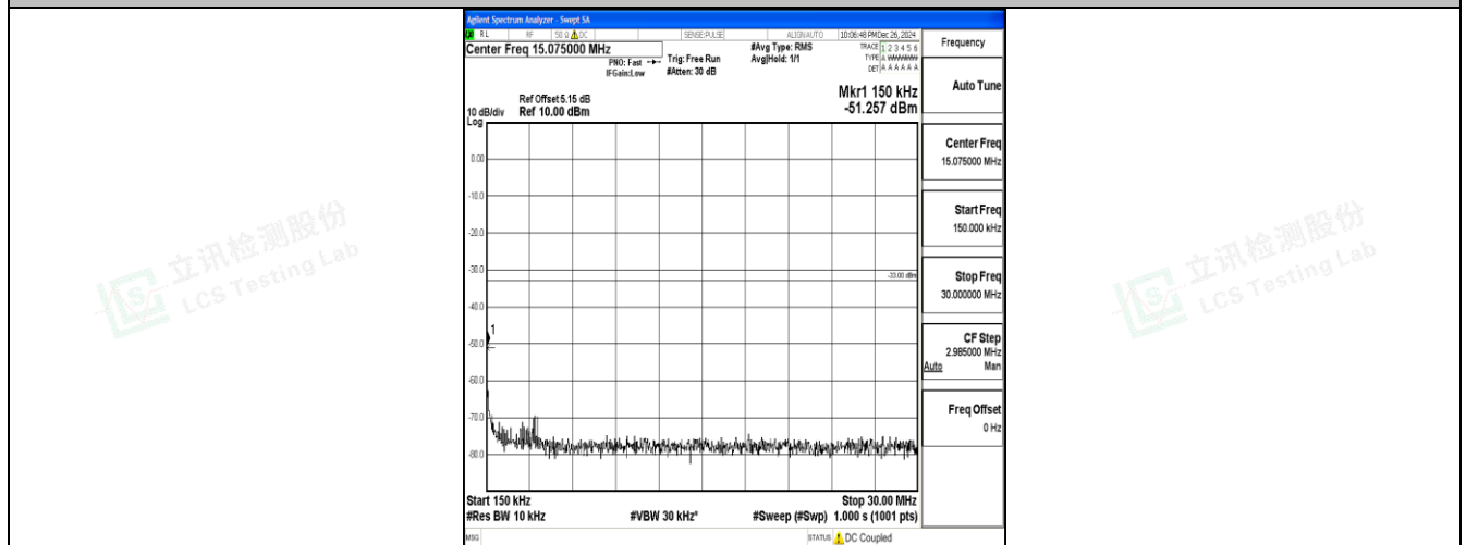
Band25_10MHz_QPSK_26640_1RB#0_0.15~30_0.15~30
