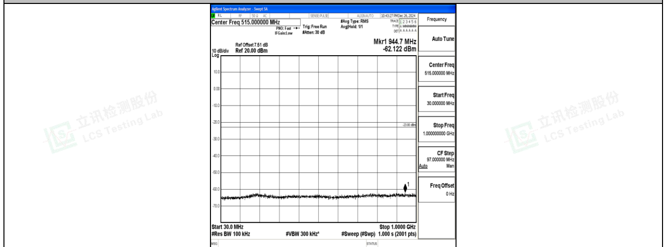
Band25_20MHz_QPSK_26365_1RB#0_30~1000_30~1000
