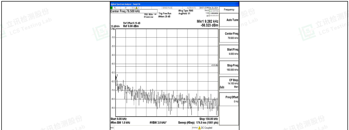
Band25_1.4MHz_16QAM_26365_1RB#0_0.009~0.15_0.009~0.15
