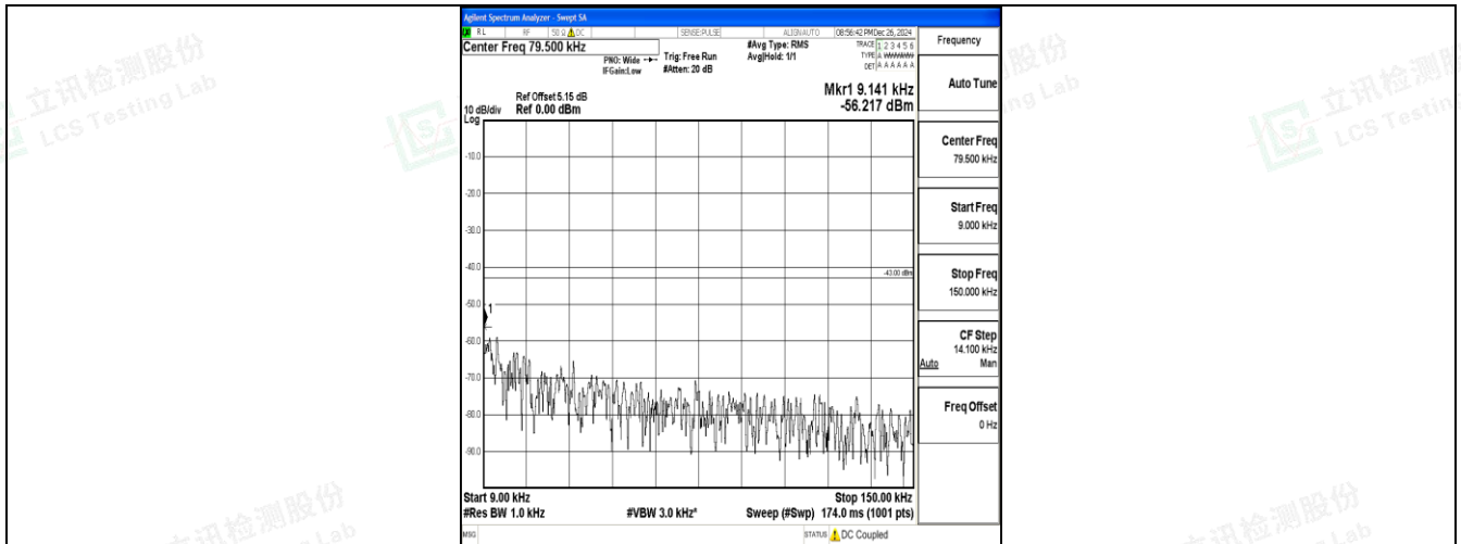
Band25_1.4MHz_QPSK_26365_1RB#0_0.009~0.15_0.009~0.15
