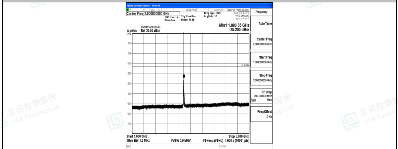
Band25_1.4MHz_QPSK_26365_1RB#0_1000~3000_1000~3000
