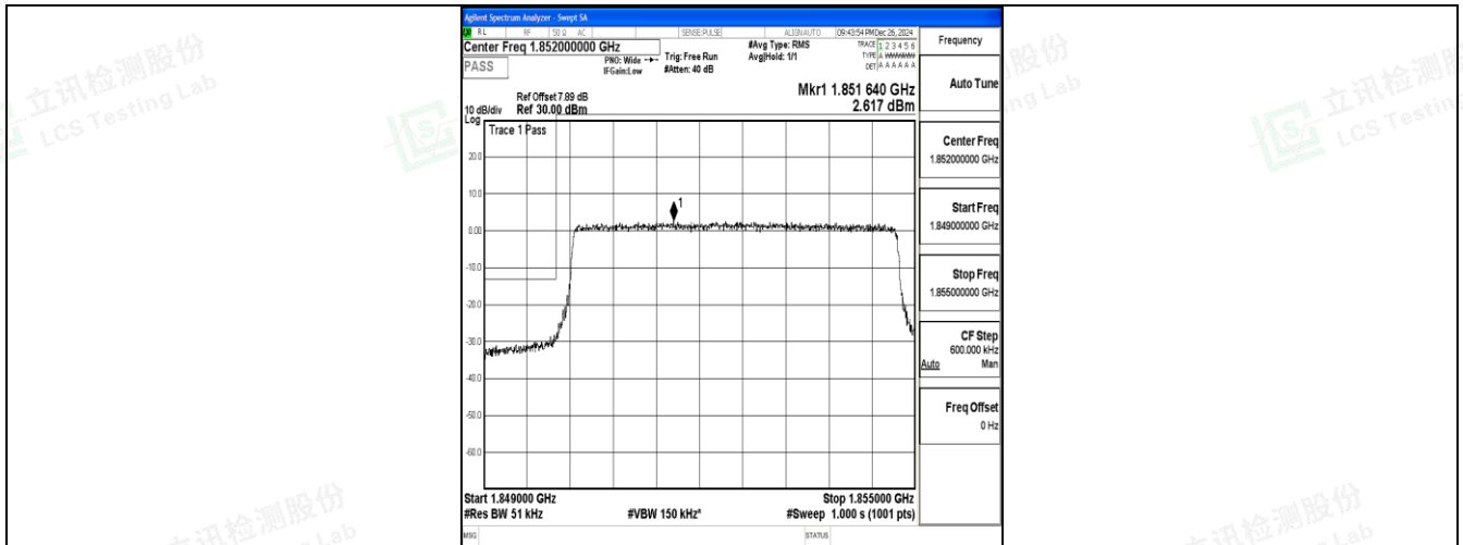
Band25_5MHz_16QAM_26065_25RB#0
