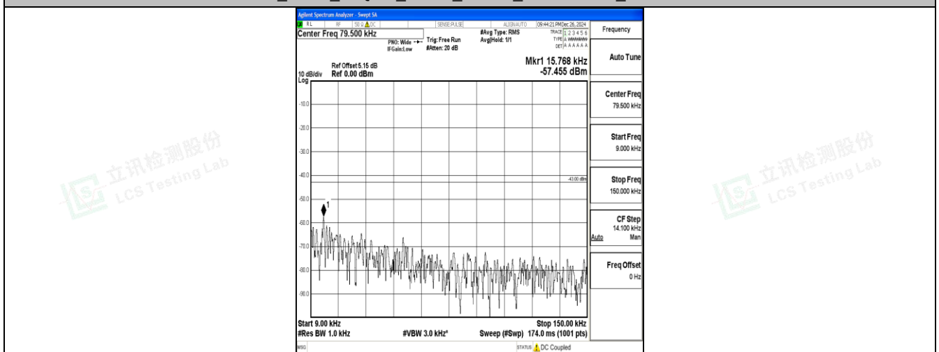
Band25_5MHz_QPSK_26065_1RB#0_0.009~0.15_0.009~0.15
