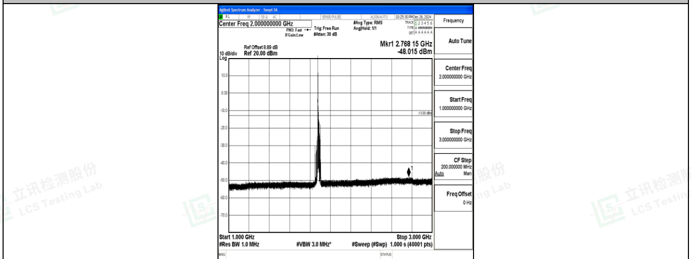
Band25_15MHz_16QAM_26365_1RB#0_1000~3000_1000~3000
