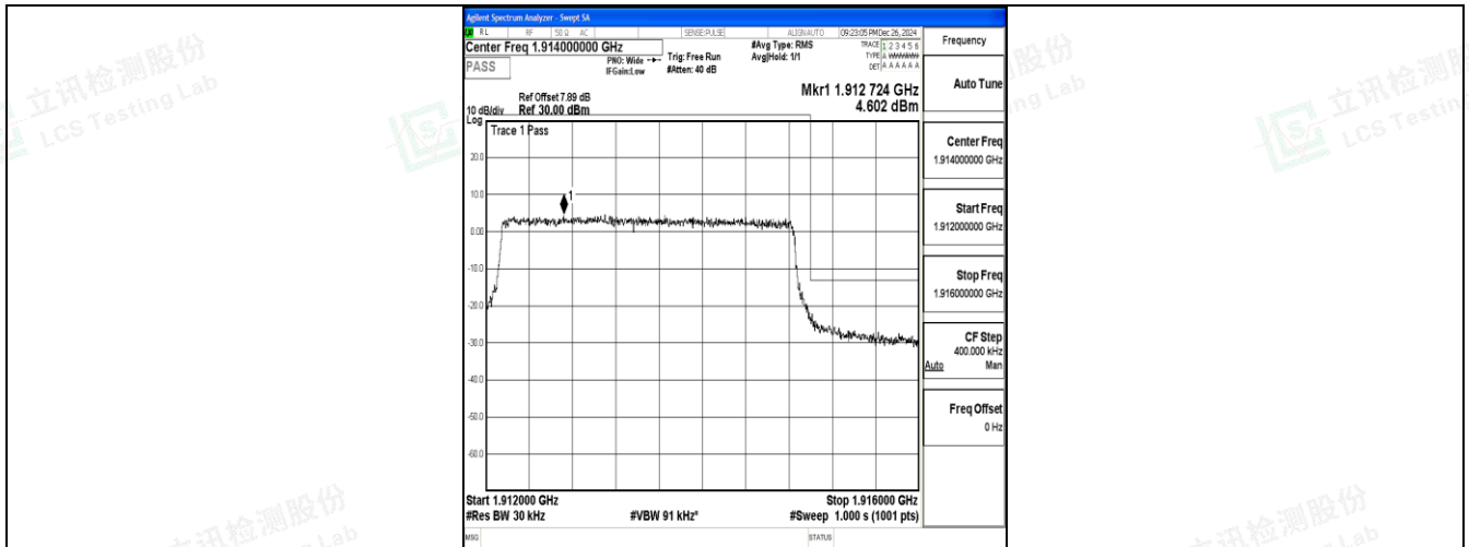
Band25_3MHz_QPSK_26675_15RB#0
