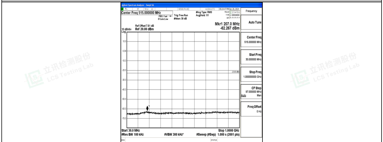
Band25_3MHz_QPSK_26365_1RB#0_30~1000_30~1000
