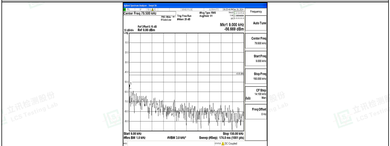
Band25_3MHz_QPSK_26675_1RB#0_0.009~0.15_0.009~0.15
