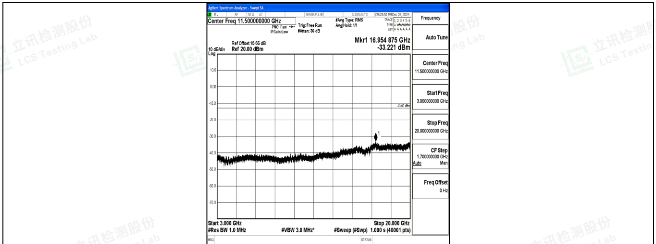
Band25_3MHz_QPSK_26055_1RB#0_3000~20000_3000~20000
