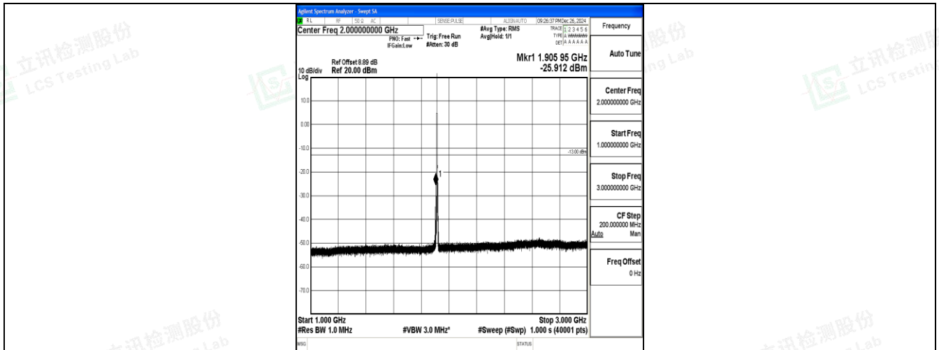
Band25_3MHz_16QAM_26675_1RB#0_1000~3000_1000~3000
