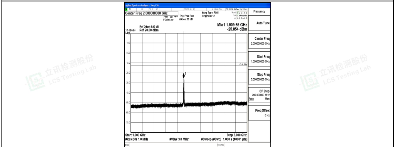
Band25_1.4MHz_QPSK_26683_1RB#0_1000~3000_1000~3000
