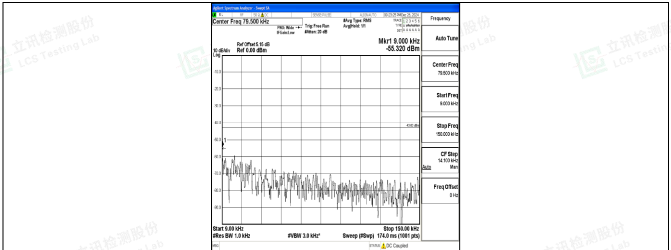
Band25_3MHz_QPSK_26055_1RB#0_0.009~0.15_0.009~0.15
