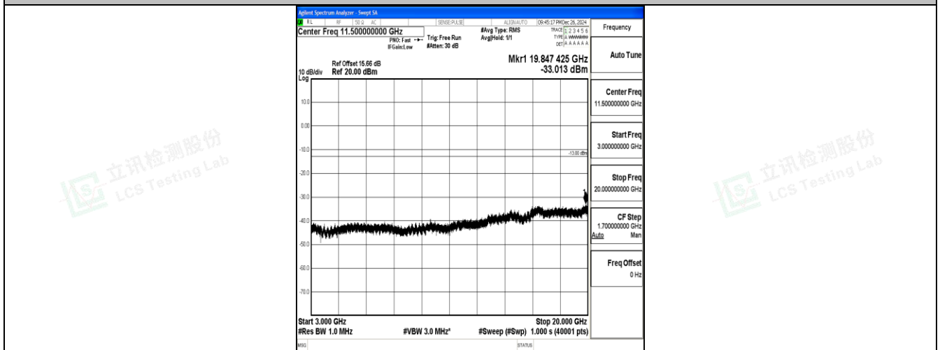
Band25_5MHz_16QAM_26065_1RB#0_3000~20000_3000~20000
