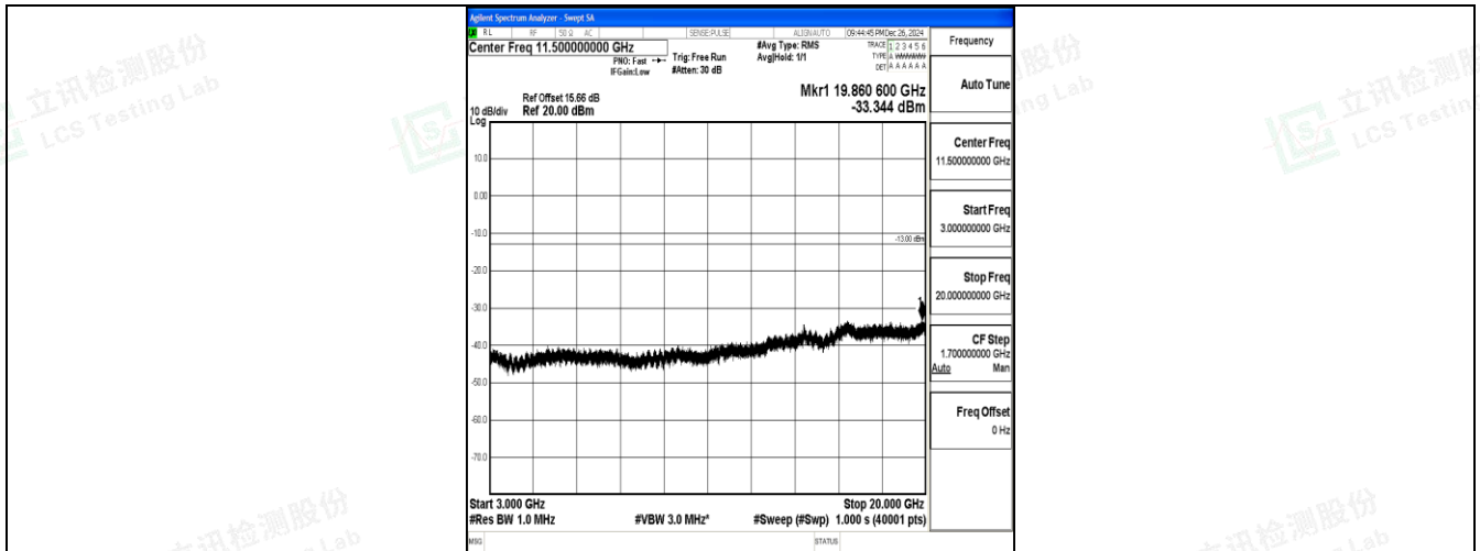
Band25_5MHz_QPSK_26065_1RB#0_3000~20000_3000~20000
