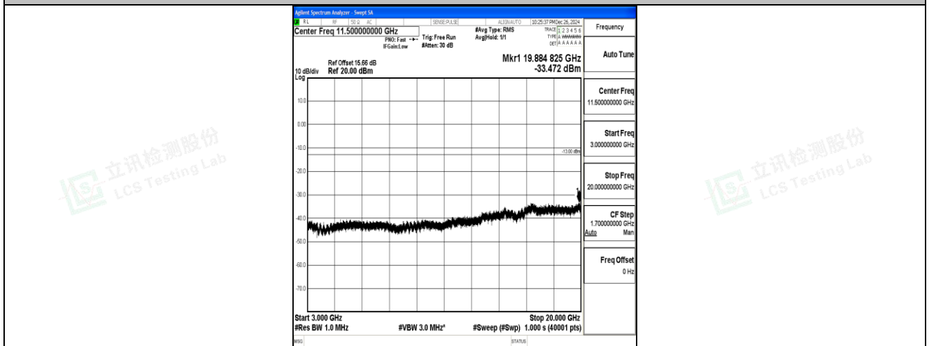
Band25_15MHz_16QAM_26365_1RB#0_3000~20000_3000~20000
