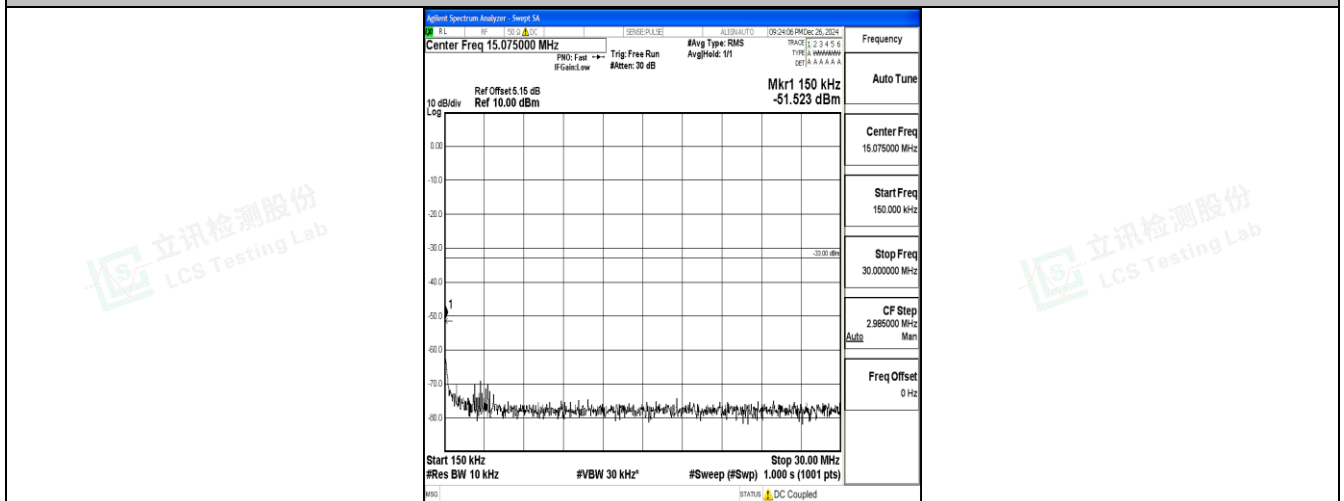
Band25_3MHz_16QAM_26055_1RB#0_0.15~30_0.15~30
