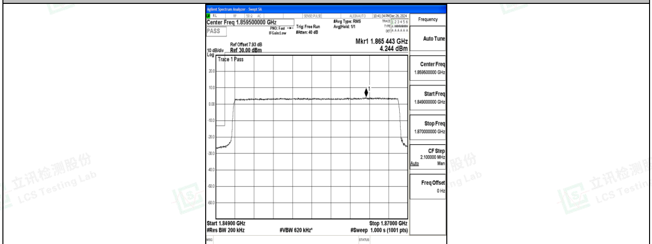
Band25_20MHz_16QAM_26140_100RB#0
