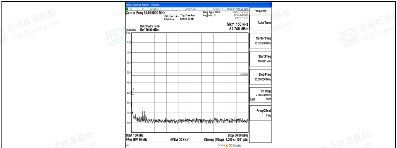
Band25_3MHz_16QAM_26365_1RB#0_0.15~30_0.15~30
