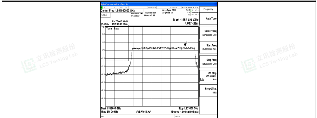
Band25_3MHz_16QAM_26055_15RB#0
