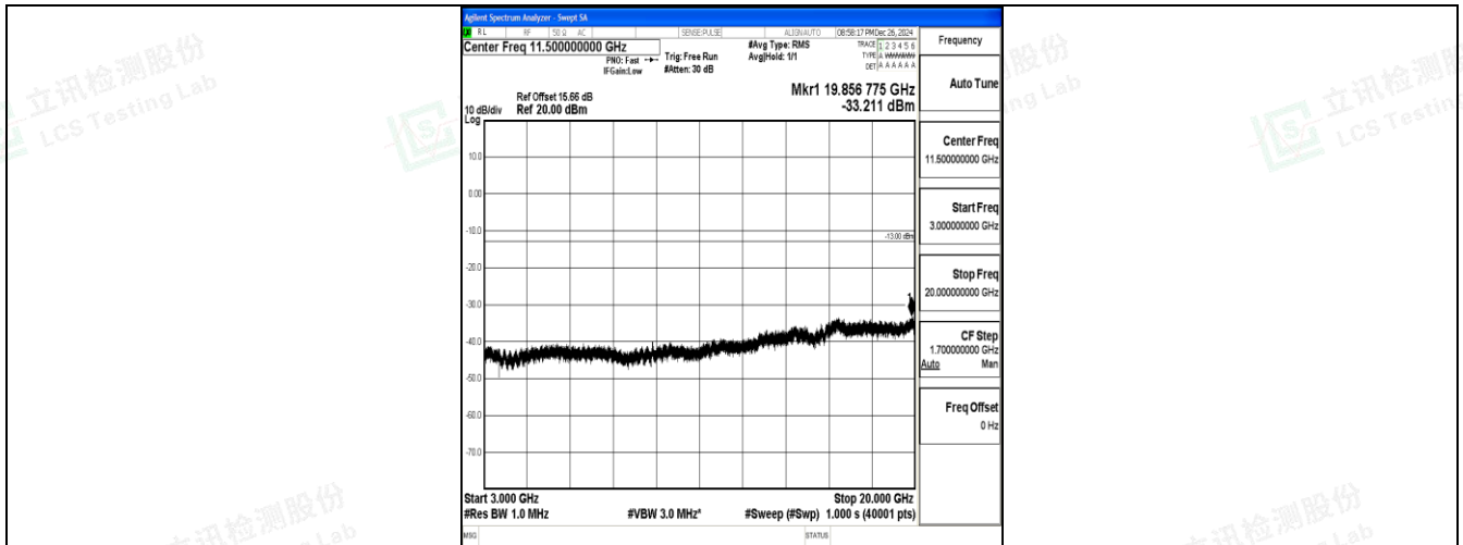
Band25_1.4MHz_QPSK_26683_1RB#0_3000~20000_3000~20000
