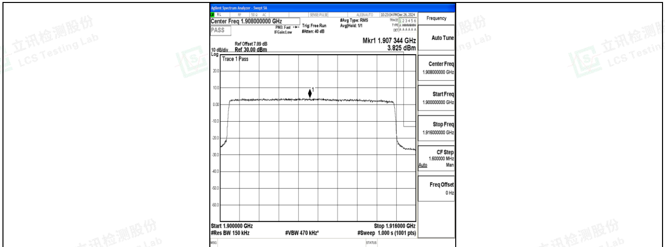
Band25_15MHz_QPSK_26615_75RB#0
