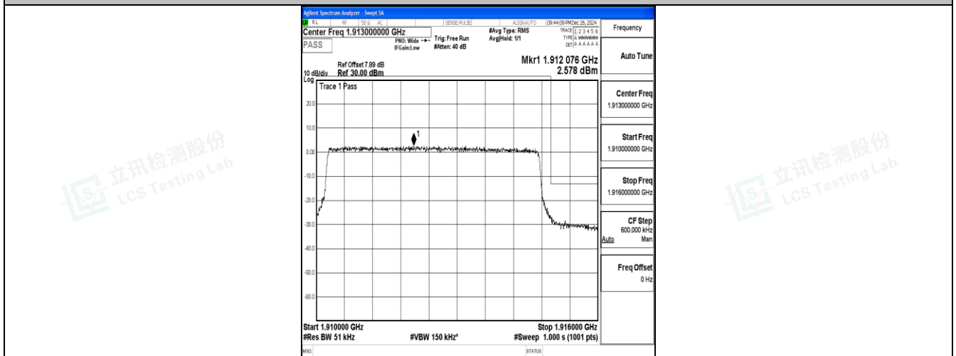
Band25_5MHz_16QAM_26665_25RB#0
