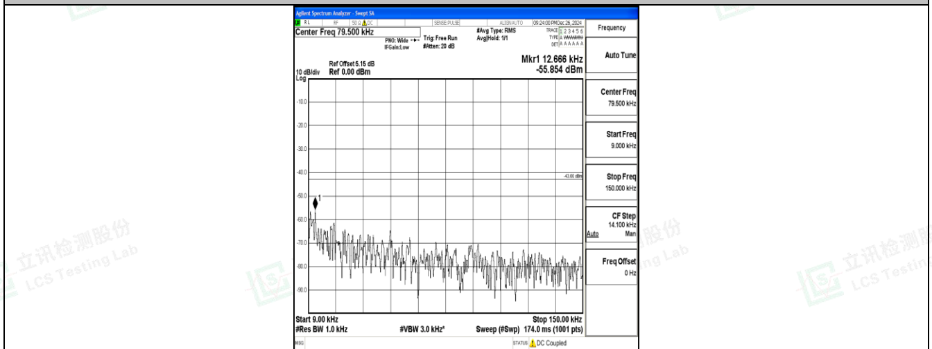
Band25_3MHz_16QAM_26055_1RB#0_0.009~0.15_0.009~0.15
