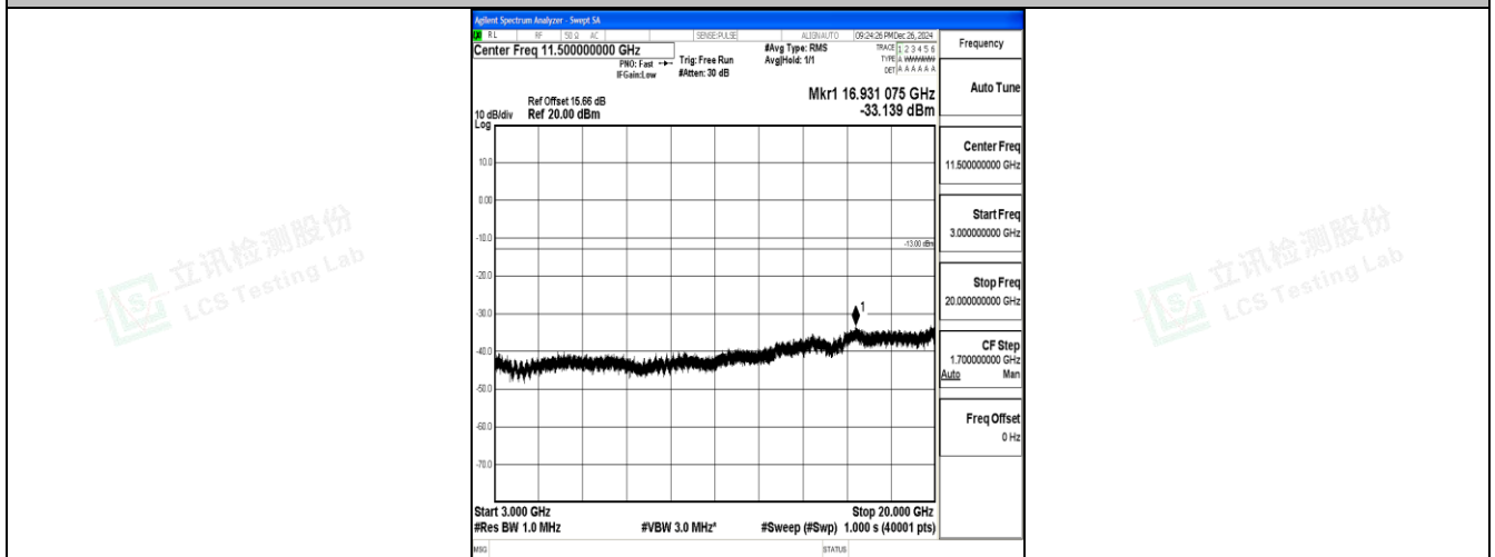
Band25_3MHz_16QAM_26055_1RB#0_3000~20000_3000~20000
