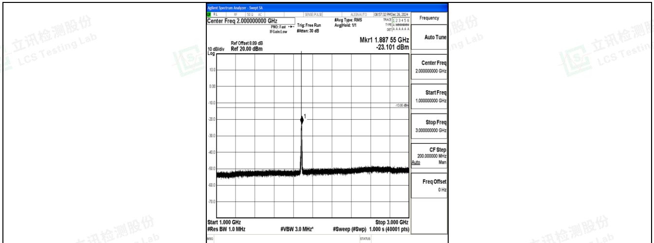
Band25_1.4MHz_16QAM_26365_1RB#0_1000~3000_1000~3000
