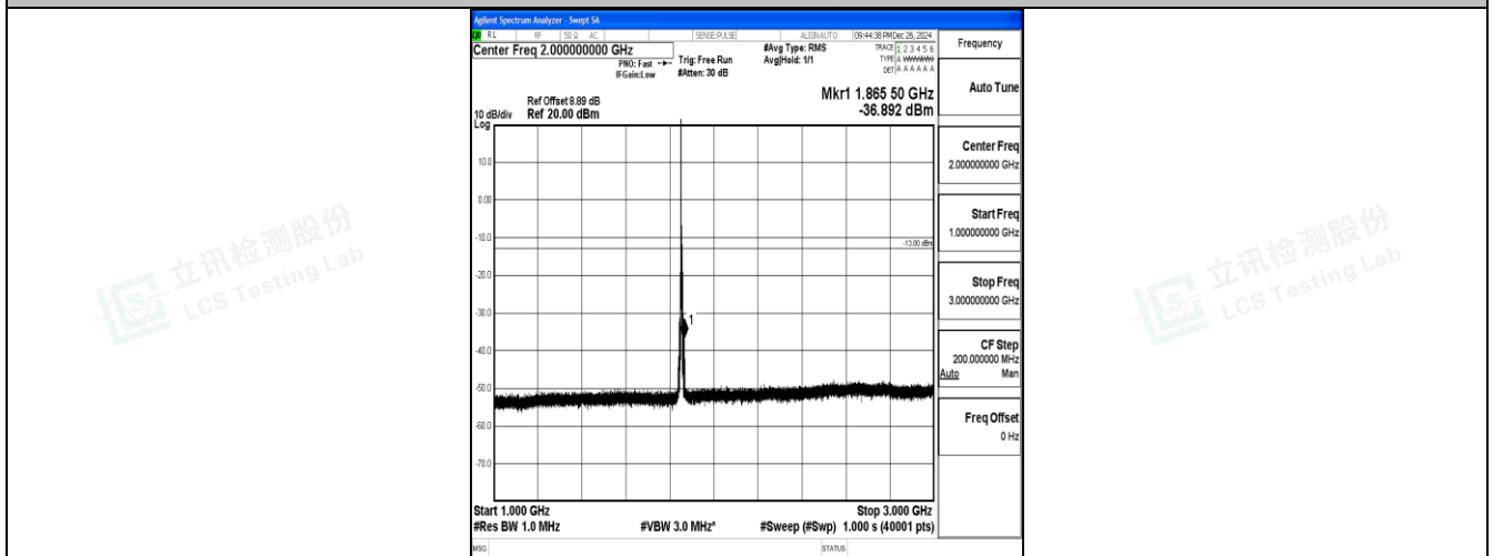
Band25_5MHz_QPSK_26065_1RB#0_1000~3000_1000~3000
