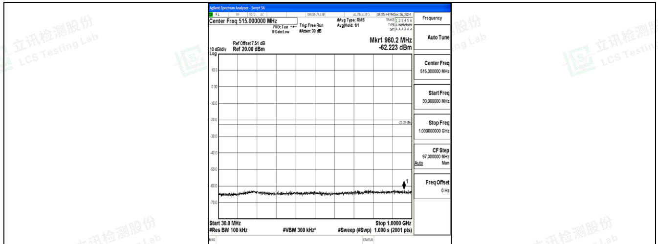
Band25_1.4MHz_QPSK_26047_1RB#0_30~1000_30~1000
