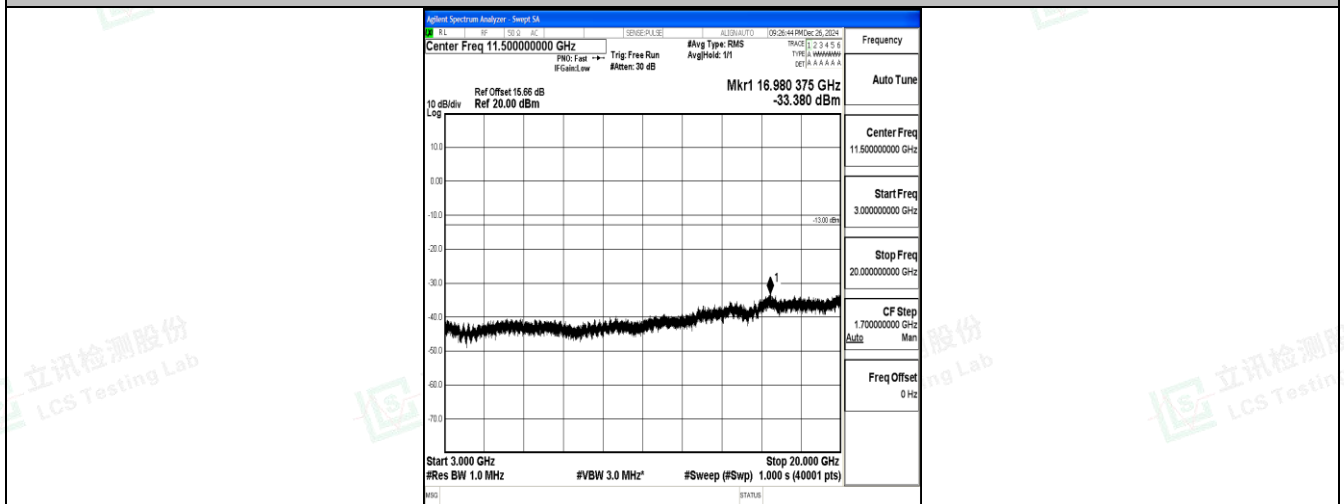
Band25_3MHz_16QAM_26675_1RB#0_3000~20000_3000~20000
