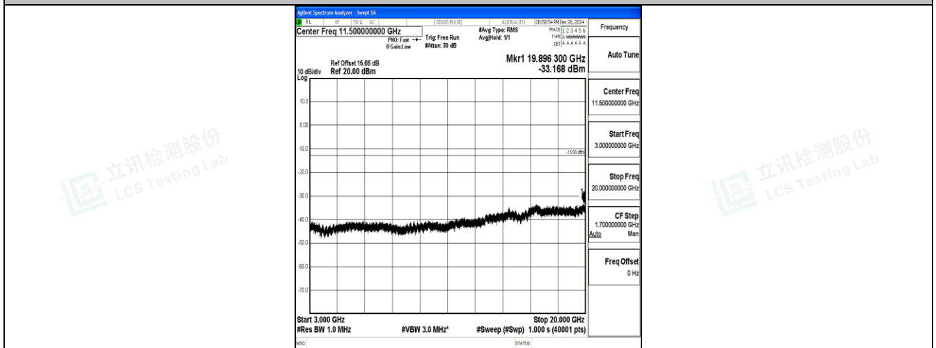
Band25_1.4MHz_16QAM_26683_1RB#0_3000~20000_3000~20000
