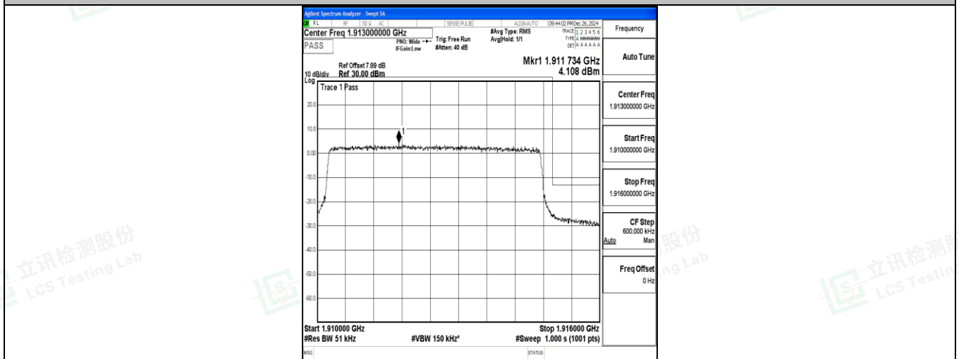
Band25_5MHz_QPSK_26665_25RB#0
