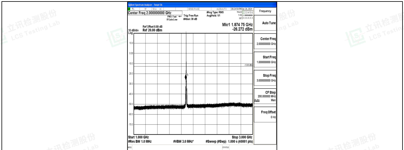
Band25_3MHz_QPSK_26365_1RB#0_1000~3000_1000~3000
