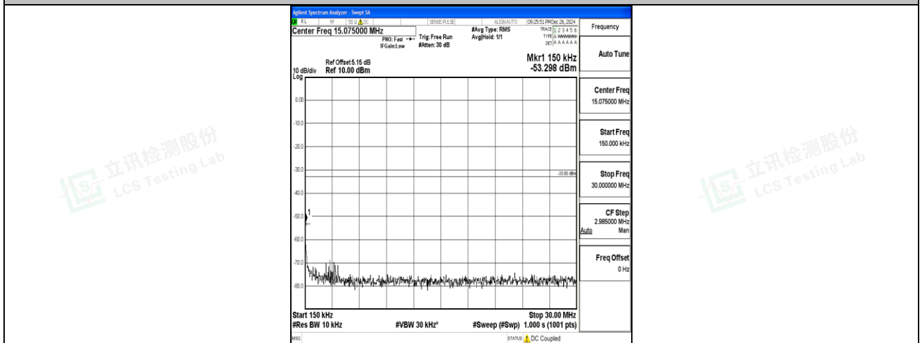
Band25_3MHz_QPSK_26675_1RB#0_0.15~30_0.15~30
