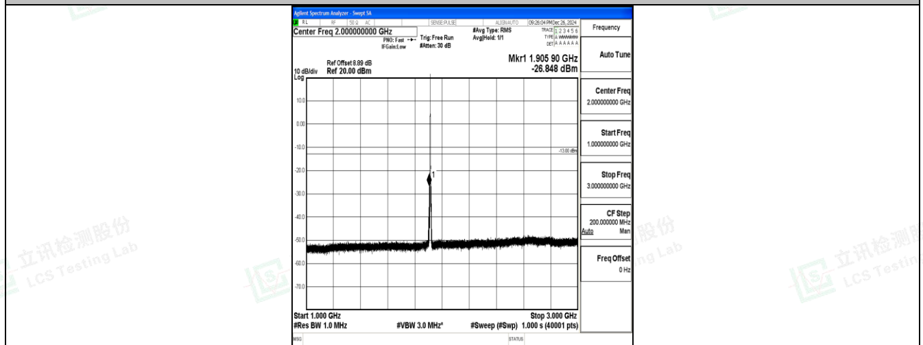
Band25_3MHz_QPSK_26675_1RB#0_1000~3000_1000~3000
