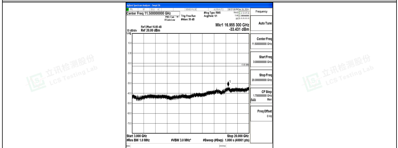
Band25_1.4MHz_QPSK_26365_1RB#0_3000~20000_3000~20000
