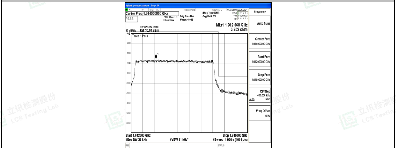
Band25_3MHz_16QAM_26675_15RB#0
