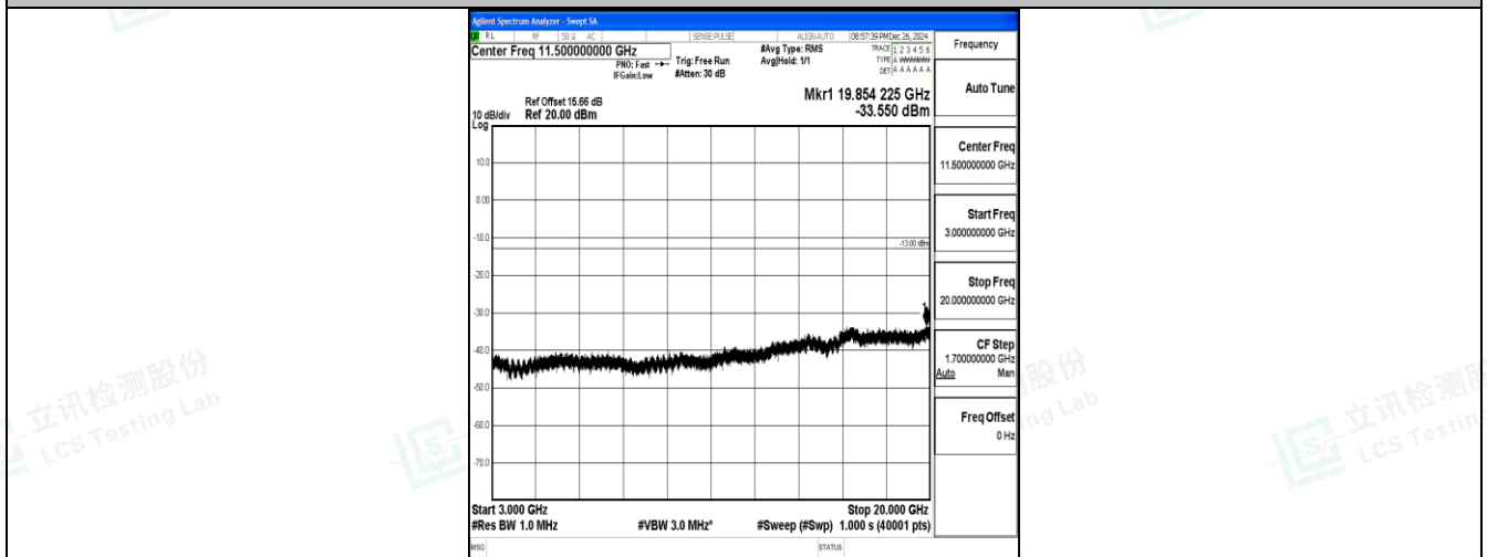
Band25_1.4MHz_16QAM_26365_1RB#0_3000~20000_3000~20000
