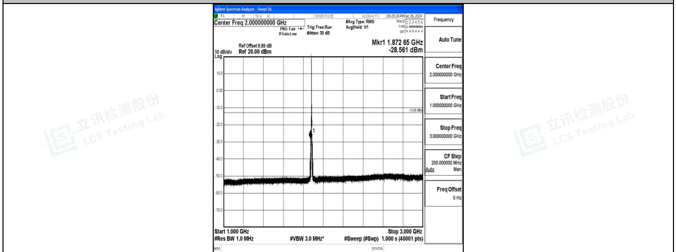
Band25_3MHz_16QAM_26365_1RB#0_1000~3000_1000~3000
