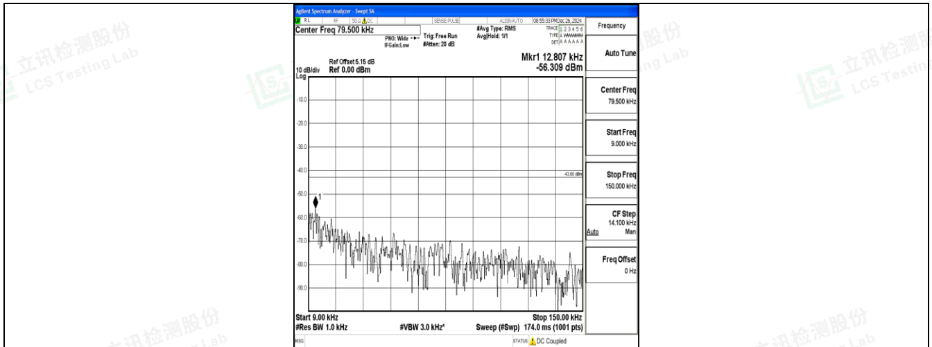
Band25_1.4MHz_QPSK_26047_1RB#0_0.009~0.15_0.009~0.15
