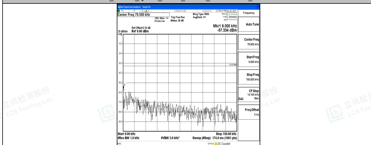
Band12 10MHz 16QAM 23130 1RB#0 0.009~0.15 0.009~0.15
