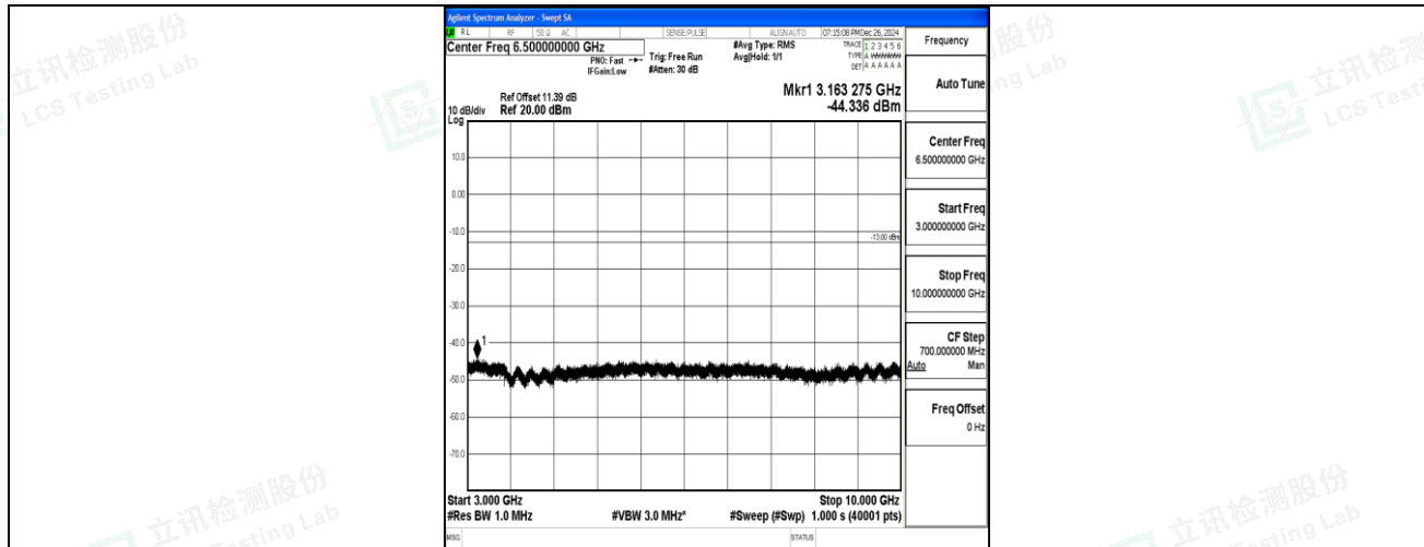
Band12_3MHz_16QAM_23025_1RB#0_3000~10000_3000~10000
