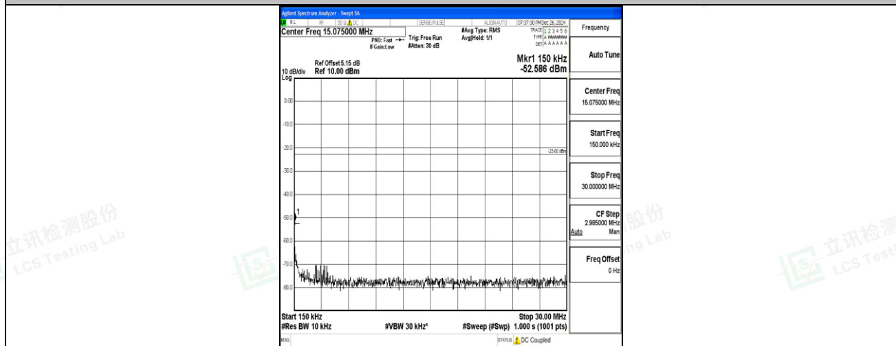
Band12_5MHz_16QAM_23095_1RB#0_0.15~30_0.15~30
