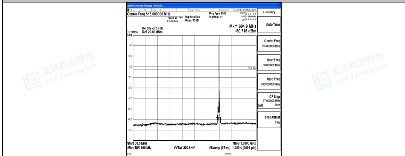
Band12_5MHz_16QAM_23095_1RB#0_30~1000_30~1000
