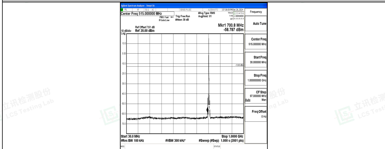
Band12_5MHz_QPSK_23155_1RB#0_30~1000_30~1000
