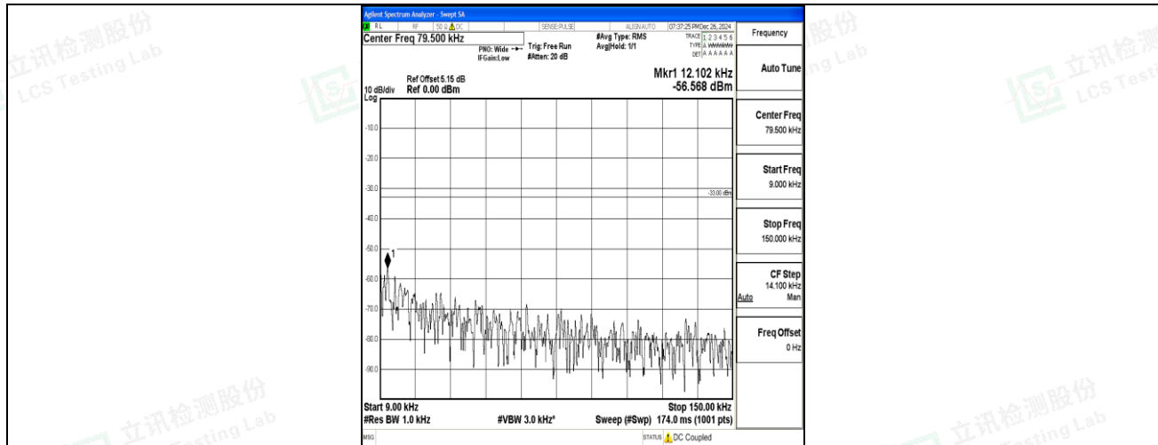
Band12_5MHz_16QAM_23095_1RB#0_0.009~0.15_0.009~0.15
