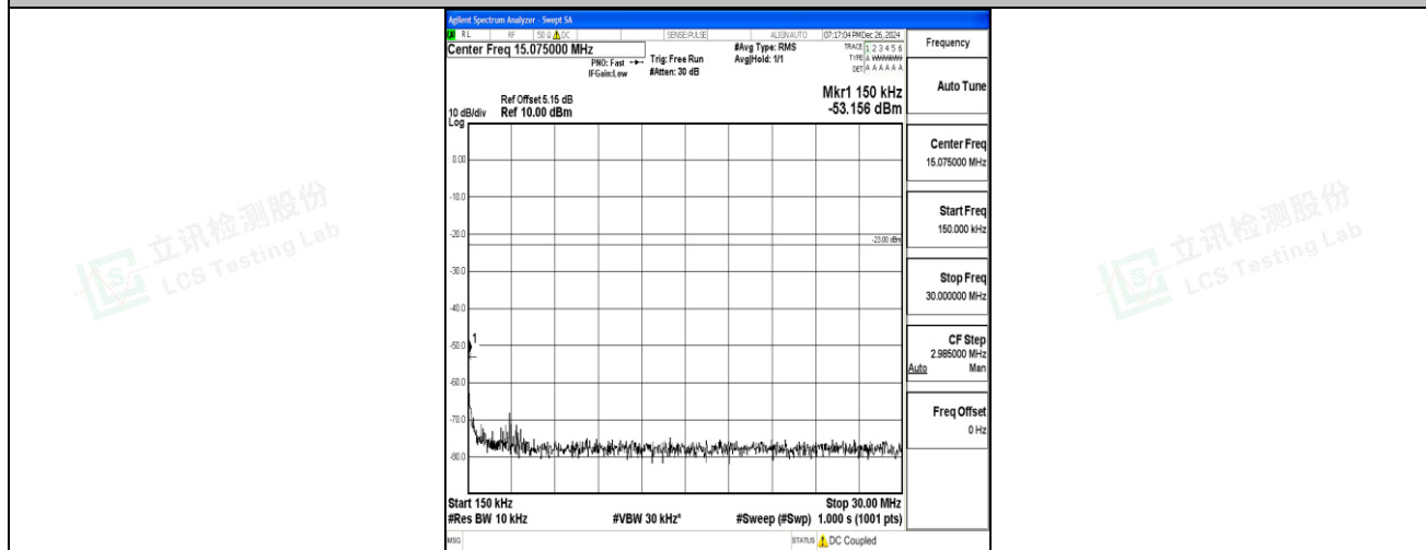
Band12_3MHz_16QAM_23165_1RB#0_0.15~30_0.15~30
