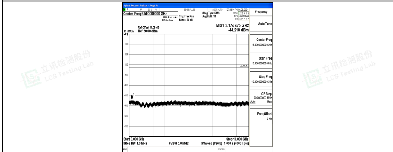
Band12_5MHz_16QAM_23155_1RB#0_3000~10000_3000~10000
