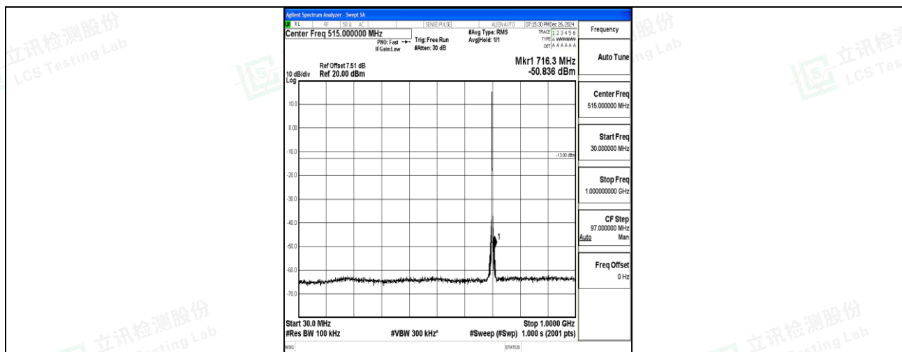
Band12_3MHz_QPSK_23095_1RB#0_30~1000_30~1000
