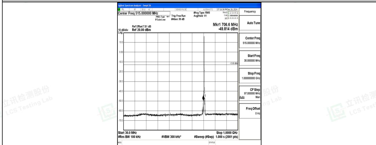
Band12_3MHz_QPSK_23165_1RB#0_30~1000_30~1000
