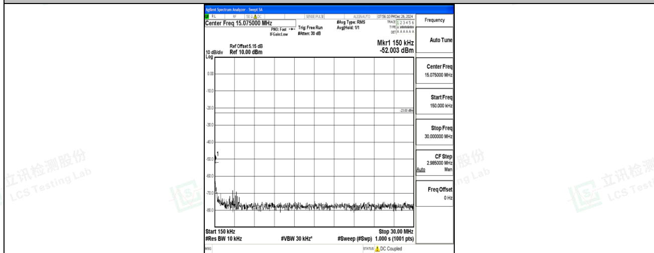
Band12_10MHz_QPSK_23060_1RB#0_0.15~30_0.15~30
