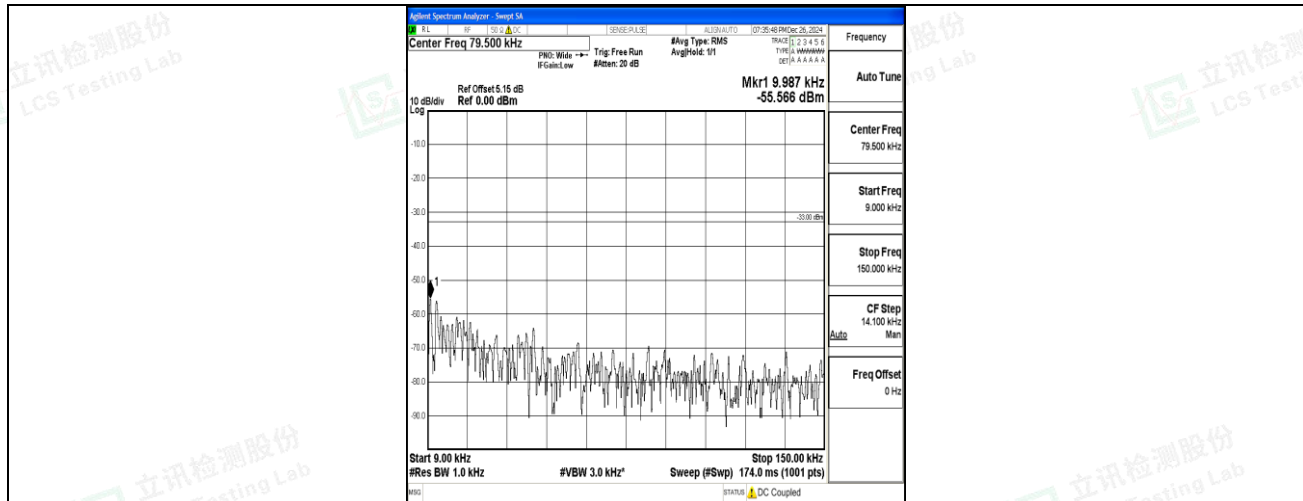
Band12_5MHz_QPSK_23035_1RB#0_0.009~0.15_0.009~0.15
