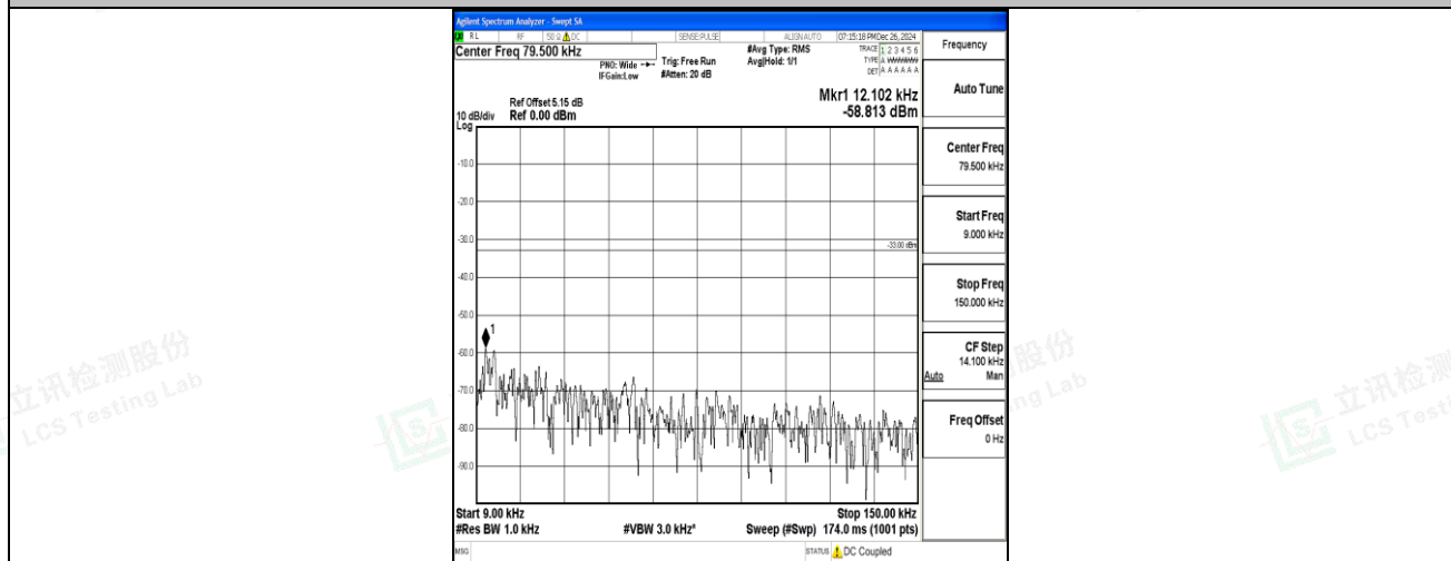
Band12_3MHz_QPSK_23095_1RB#0_0.009~0.15_0.009~0.15
