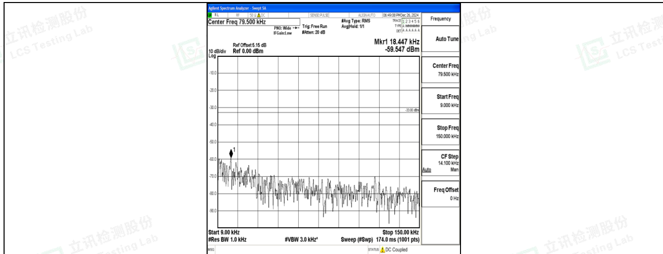
Band12_1.4MHz_QPSK_23173_1RB#0_0.009~0.15_0.009~0.15
