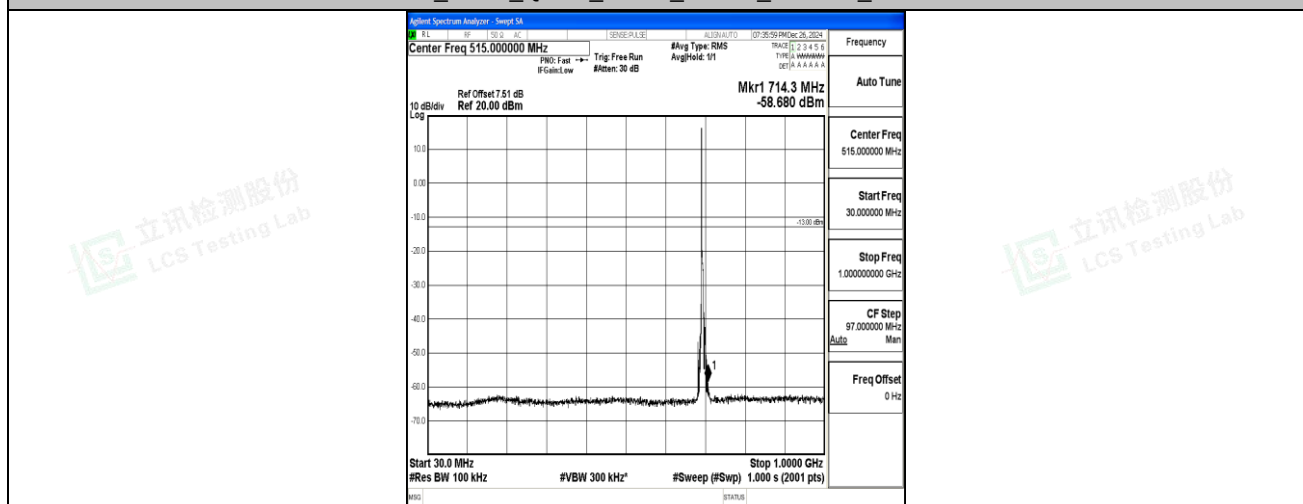
Band12_5MHz_QPSK_23035_1RB#0_30~1000_30~1000
