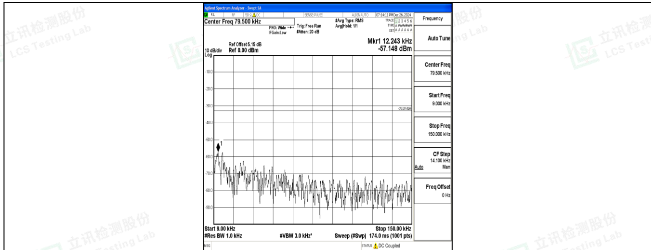
Band12_3MHz_QPSK_23025_1RB#0_0.009~0.15_0.009~0.15
