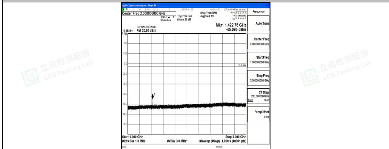
Band12_5MHz_QPSK_23155_1RB#0_1000~3000_1000~3000
