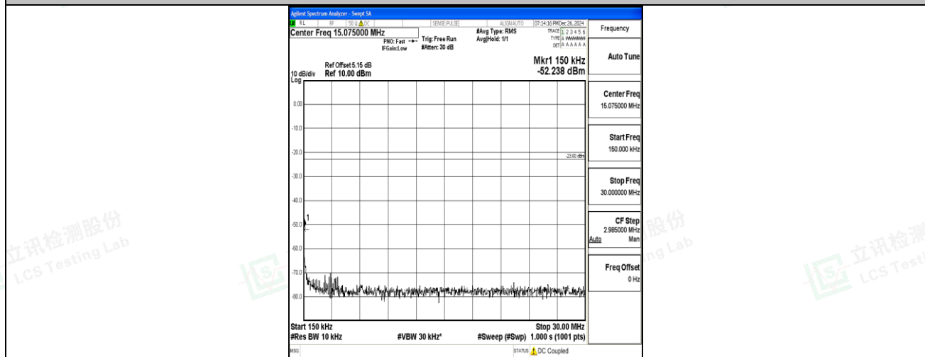
Band12_3MHz_QPSK_23025_1RB#0_0.15~30_0.15~30
