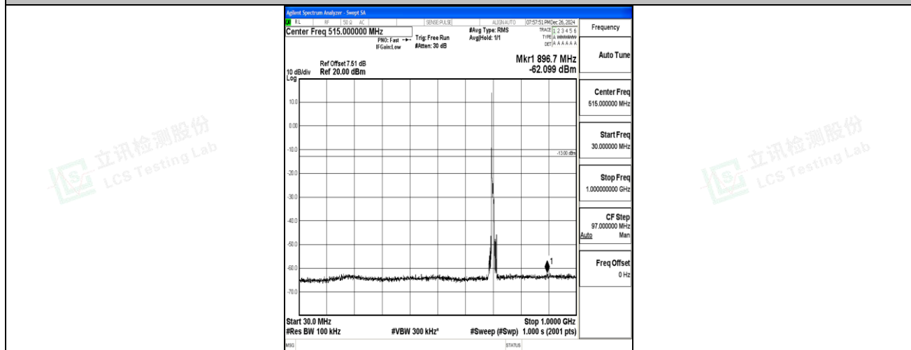
Band12_10MHz_16QAM_23095_1RB#0_30~1000_30~1000
