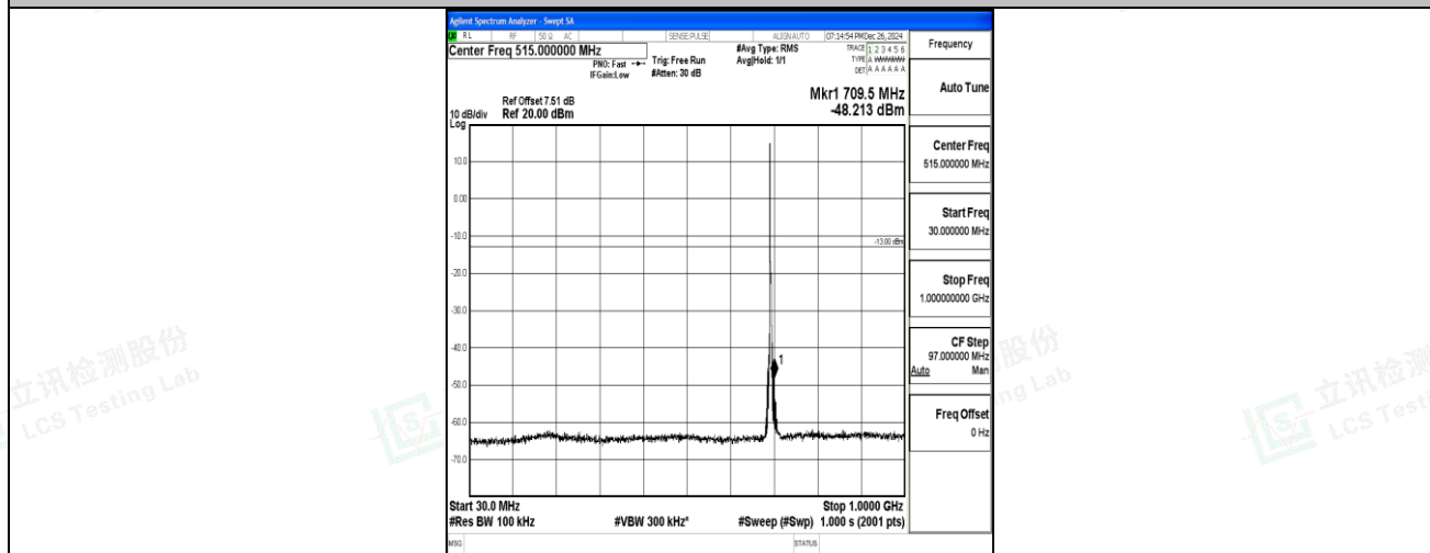
Band12_3MHz_16QAM_23025_1RB#0_30~1000_30~1000
