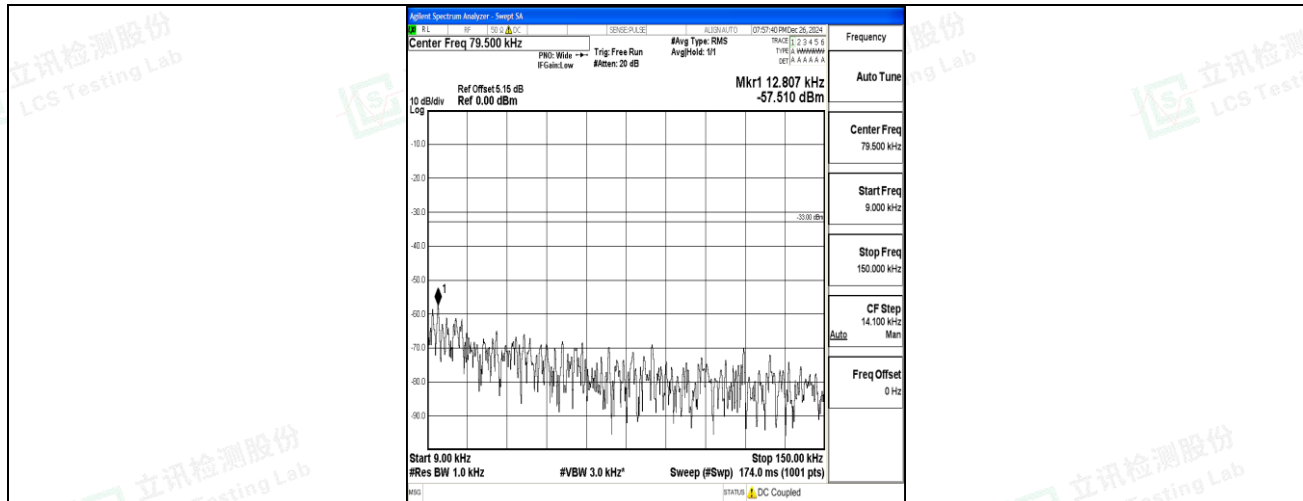
Band12_10MHz_16QAM_23095_1RB#0_0.009~0.15_0.009~0.15
