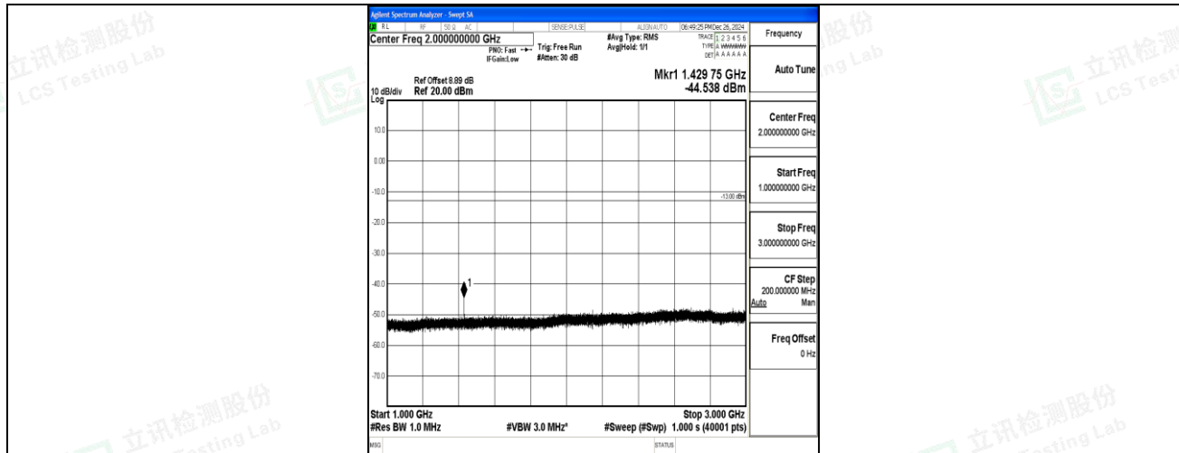
Band12_1.4MHz_QPSK_23173_1RB#0_1000~3000_1000~3000
