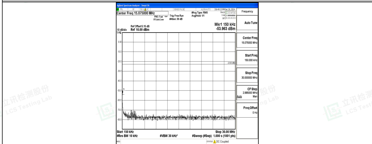
Band12_1.4MHz_QPSK_23173_1RB#0_0.15~30_0.15~30
