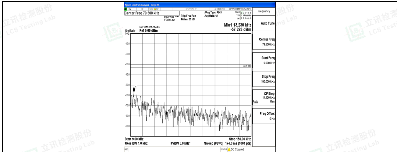
Band12_3MHz_16QAM_23095_1RB#0_0.009~0.15_0.009~0.15
