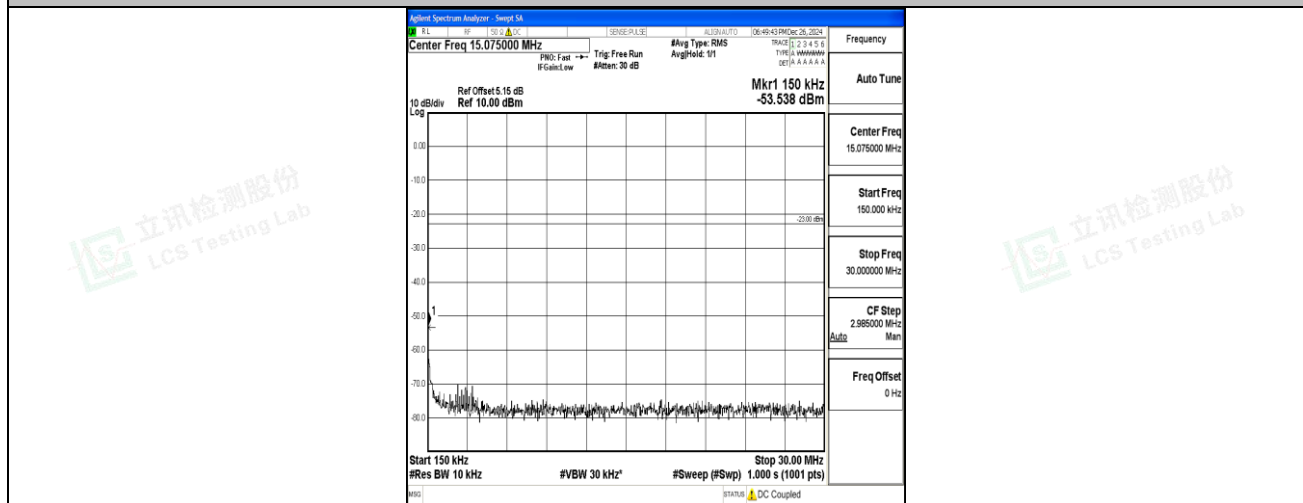
Band12_1.4MHz_16QAM_23173_1RB#0_0.15~30_0.15~30
