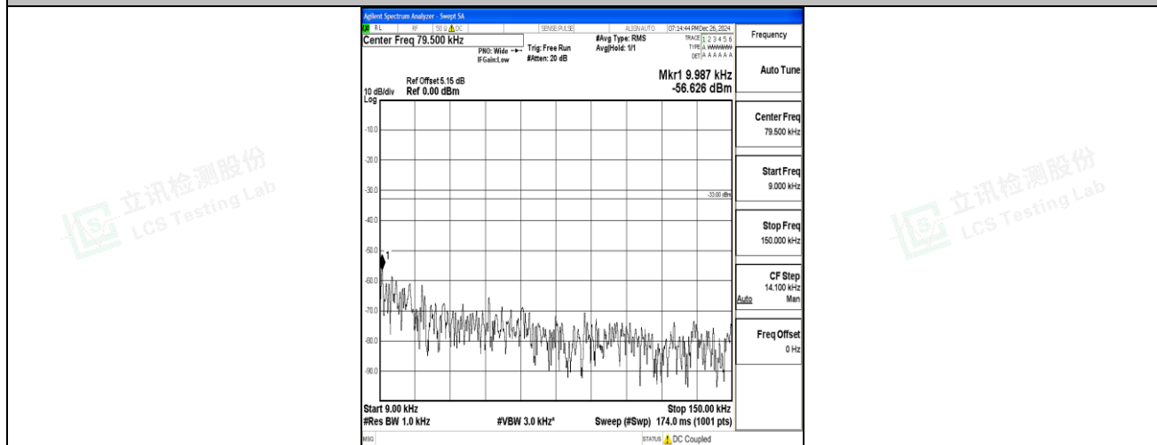
Band12_3MHz_16QAM_23025_1RB#0_0.009~0.15_0.009~0.15
