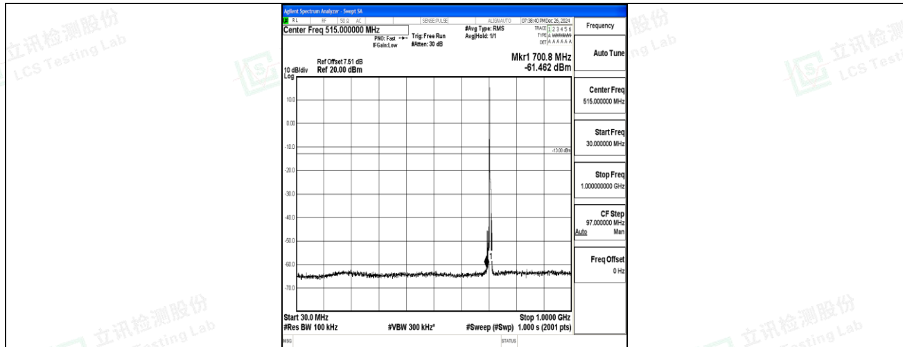
Band12_5MHz_16QAM_23155_1RB#0_30~1000_30~1000
