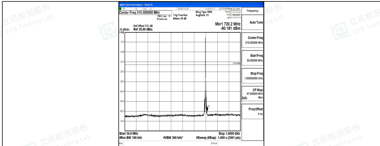
Band12_5MHz_QPSK_23095_1RB#0_30~1000_30~1000
