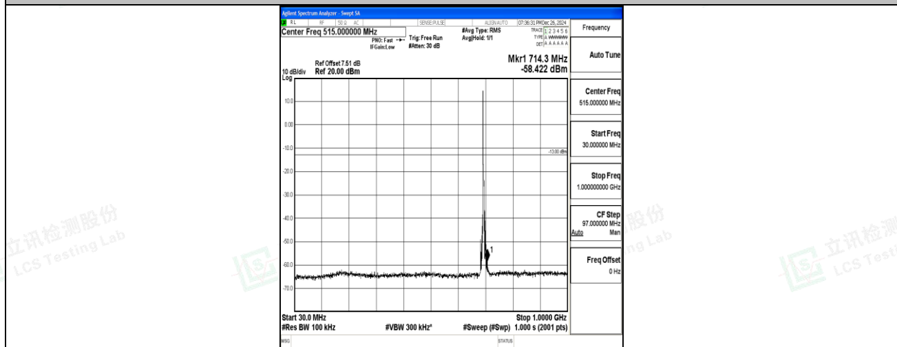
Band12_5MHz_16QAM_23035_1RB#0_30~1000_30~1000
