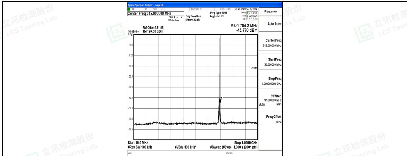
Band12_1.4MHz_QPSK_23017_1RB#0_30-1000_30-1000
