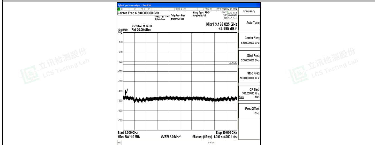
Band12_3MHz_16QAM_23165_1RB#0_3000~10000_3000~10000
