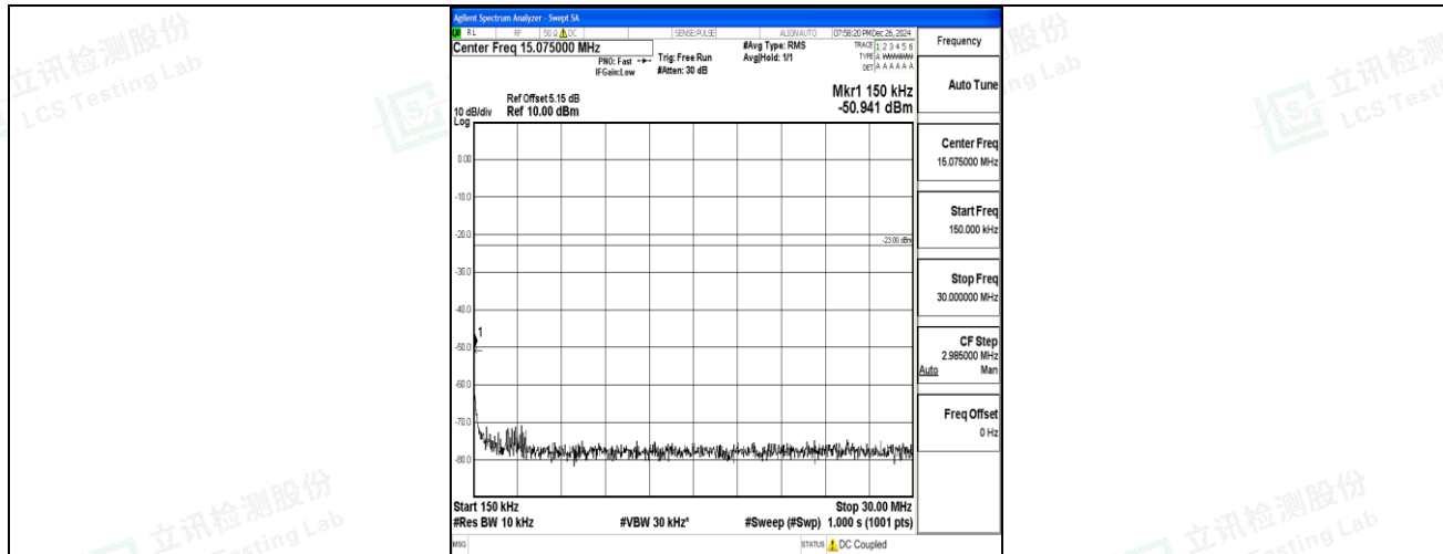
Band12_10MHz_QPSK_23130_1RB#0_0.15~30_0.15~30
