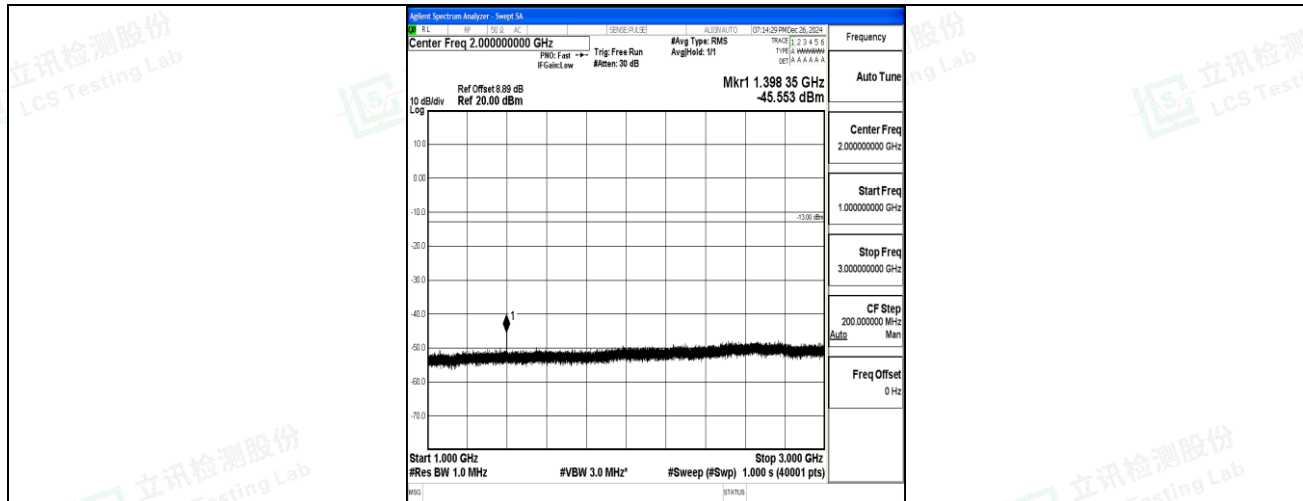
Band12_3MHz_QPSK_23025_1RB#0_1000~3000_1000~3000
