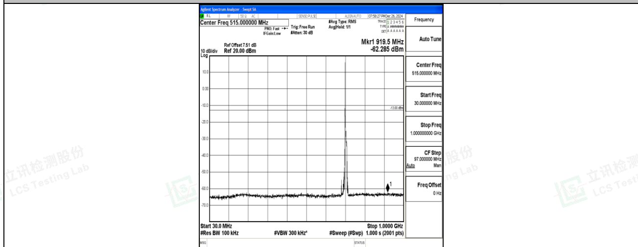
Band12_10MHz_QPSK_23130_1RB#0_30~1000_30~1000
