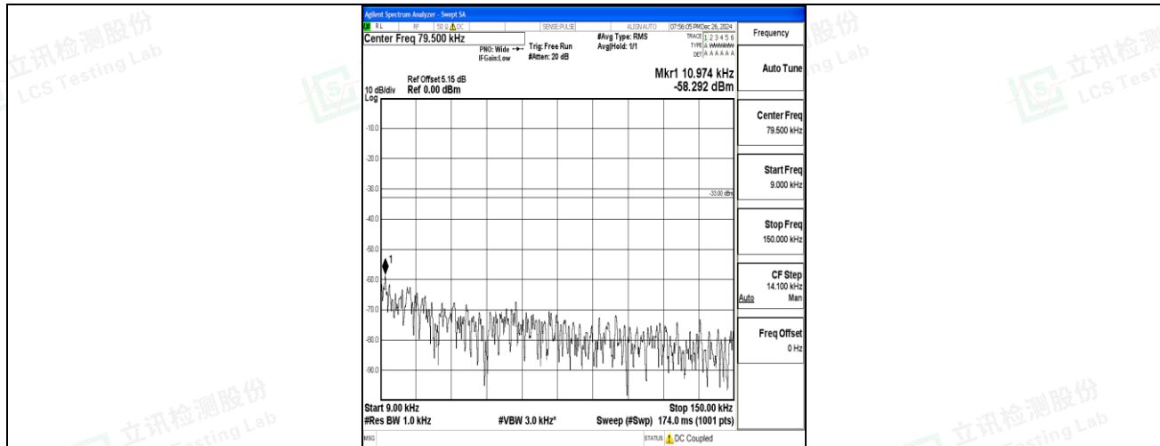
Band12_10MHz_QPSK_23060_1RB#0_0.009~0.15_0.009~0.15
