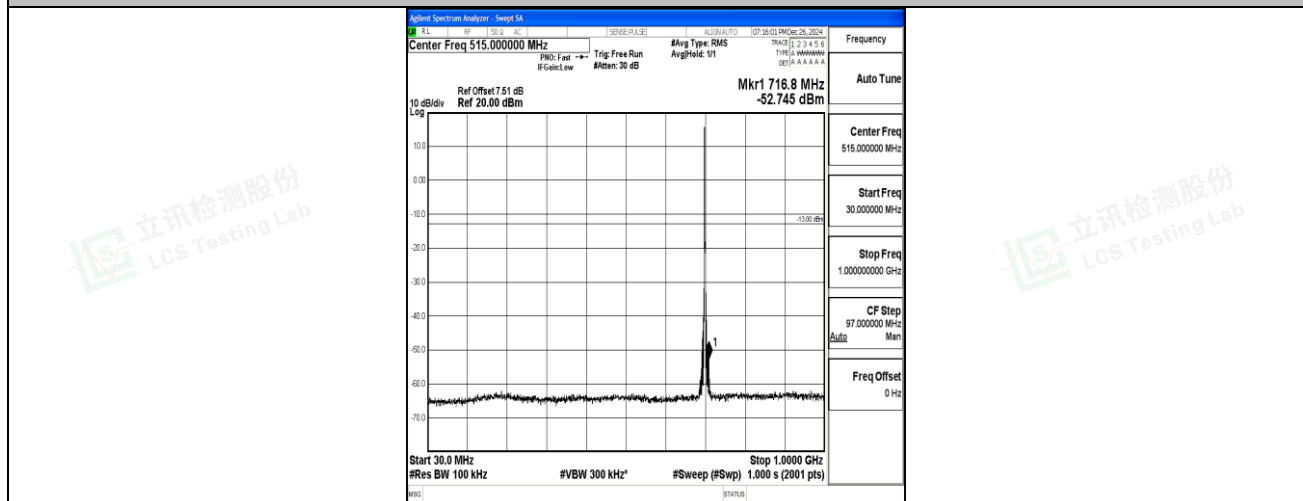
Band12_3MHz_16QAM_23095_1RB#0_30~1000_30~1000
