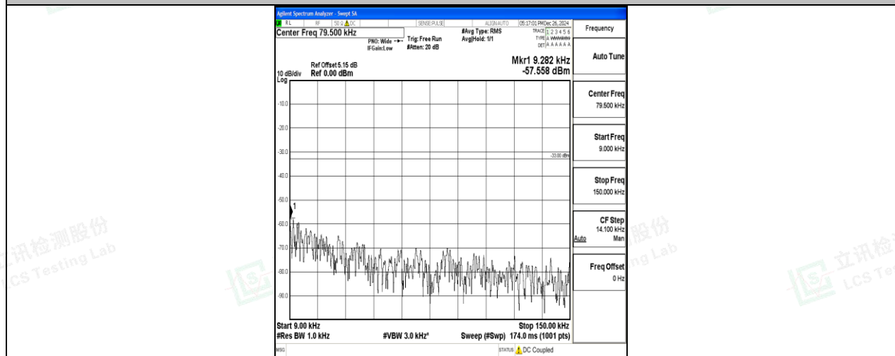
Band5_10MHz_16QAM_20600_1RB#0_0.009~0.15_0.009~0.15
