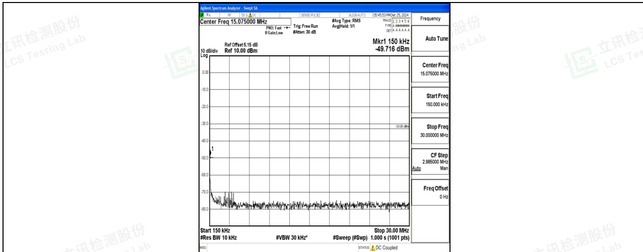
Band4_15MHz_16QAM_20175_1RB#0_0.15~30_0.15~30
