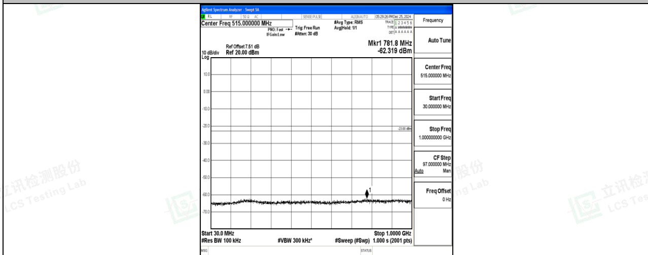
Band4_10MHz_16QAM_20175_1RB#0_30~1000_30~1000
