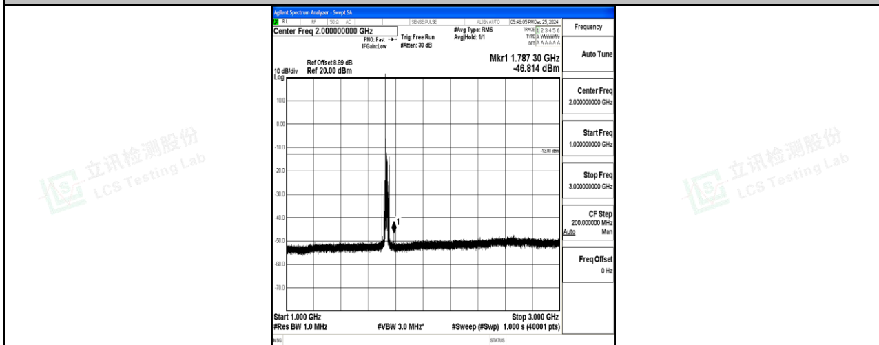
Band4_15MHz_16QAM_20175_1RB#0_1000~3000_1000~3000
