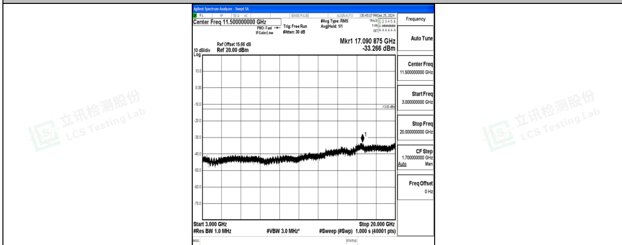
Band4_15MHz_16QAM_20025_1RB#0_3000-20000_3000-20000
