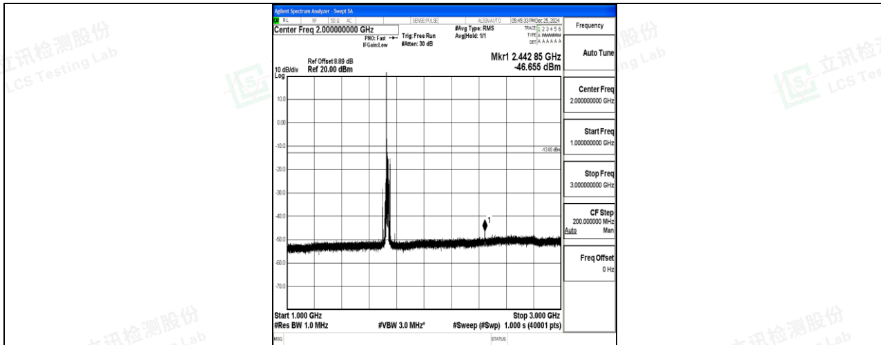
Band4_15MHz_QPSK_20175_1RB#0_1000~3000_1000~3000
