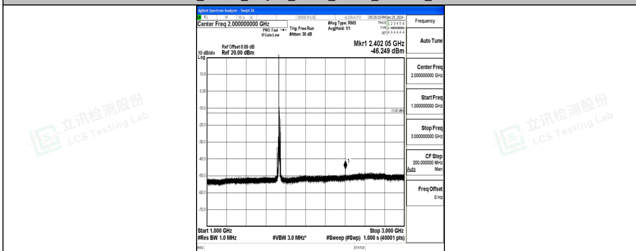
Band4_10MHz_16QAM_20175_1RB#0_1000~3000_1000~3000
