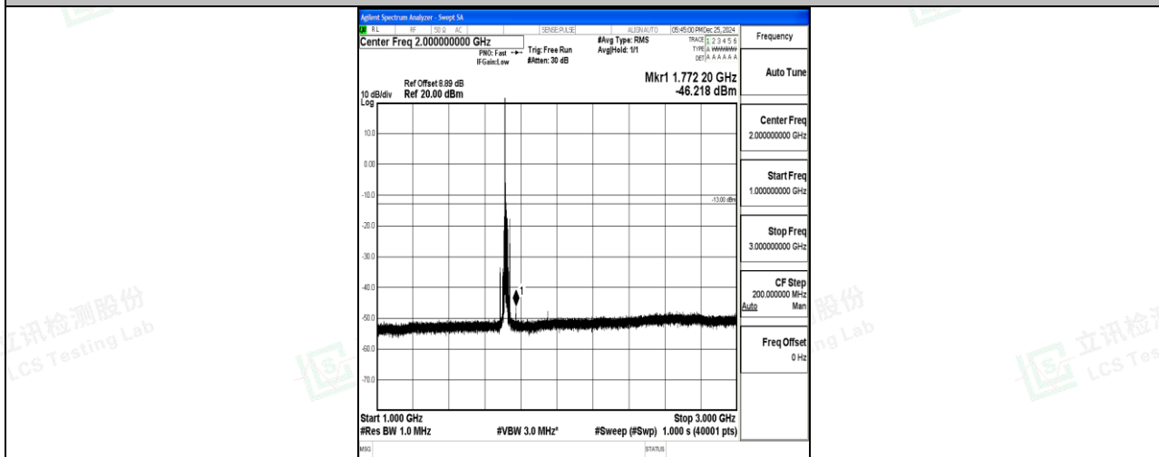
Band4_15MHz_16QAM_20025_1RB#0_1000-3000_1000-3000
