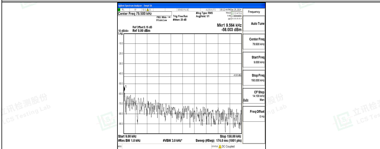
Band4_5MHz_QPSK_20375_1RB#0_0.009~0.15_0.009~0.15
