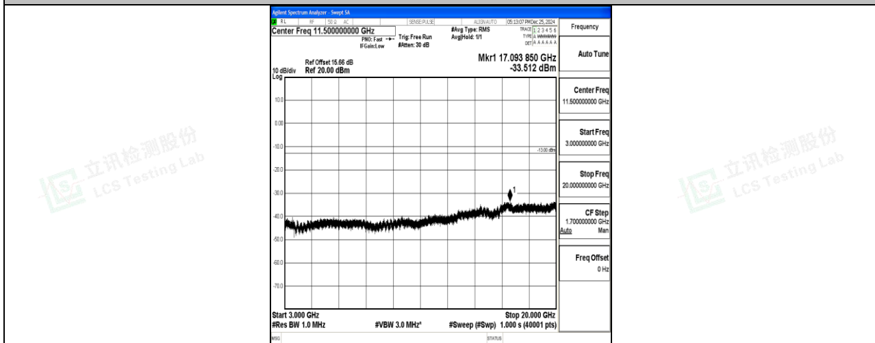
Band4_5MHz_QPSK_20375_1RB#0_3000~20000_3000~20000
