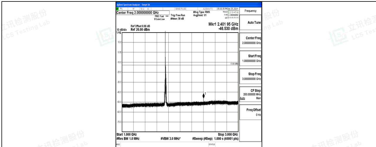
Band4_10MHz_16QAM_20350_1RB#0_1000~3000_1000~3000
