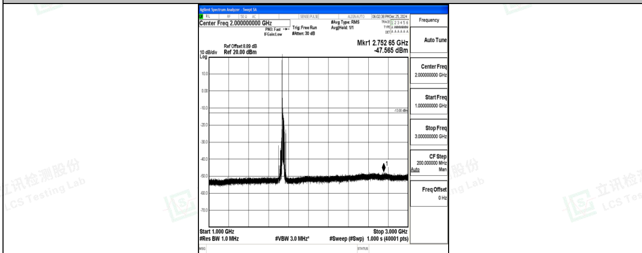
Band4_20MHz_QPSK_20300_1RB#0_1000~3000_1000~3000
