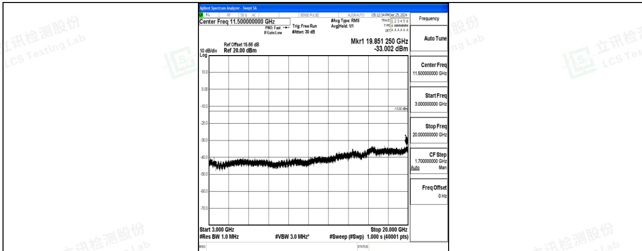
Band4_5MHz_16QAM_20175_1RB#0_3000~20000_3000~20000
