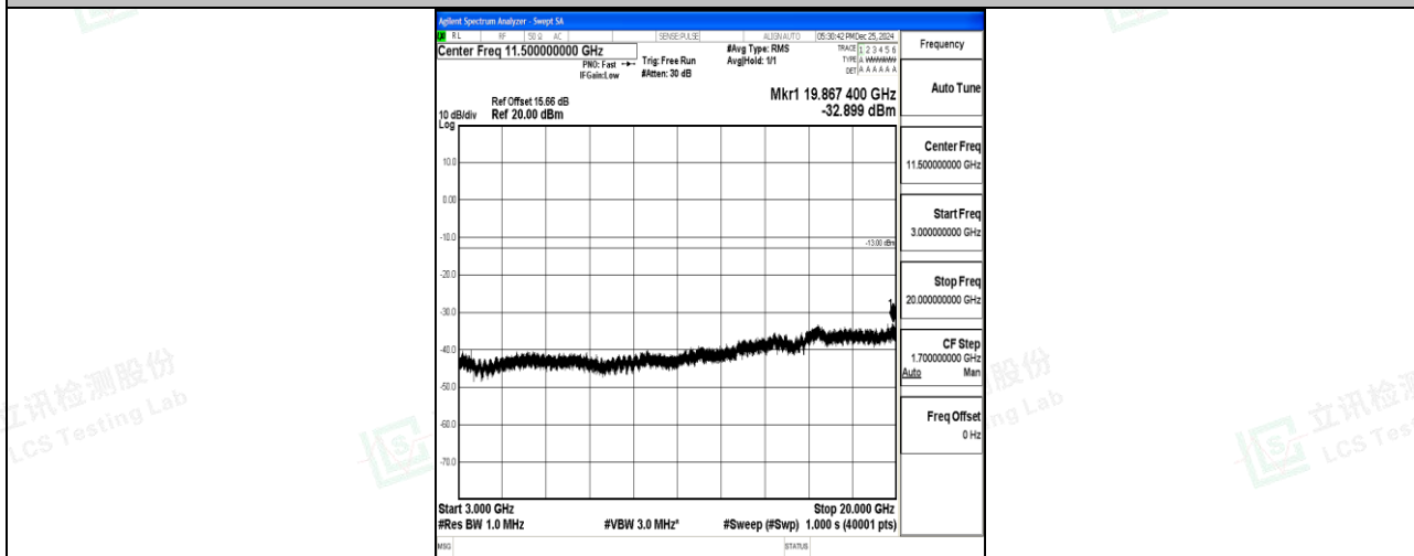
Band4_10MHz_16QAM_20350_1RB#0_3000~20000_3000~20000
