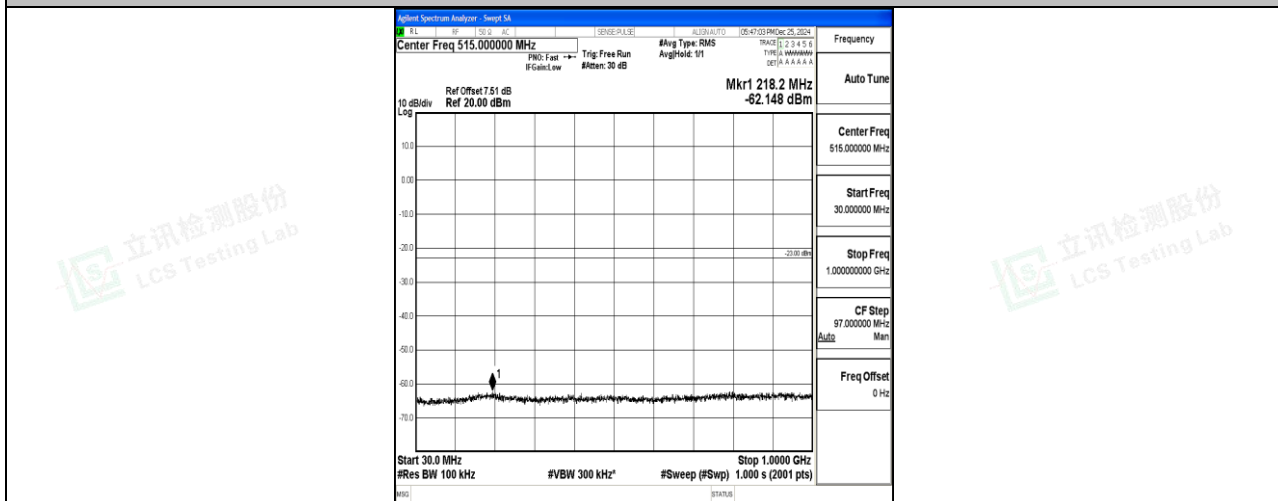
Band4_15MHz_16QAM_20325_1RB#0_30~1000_30~1000
