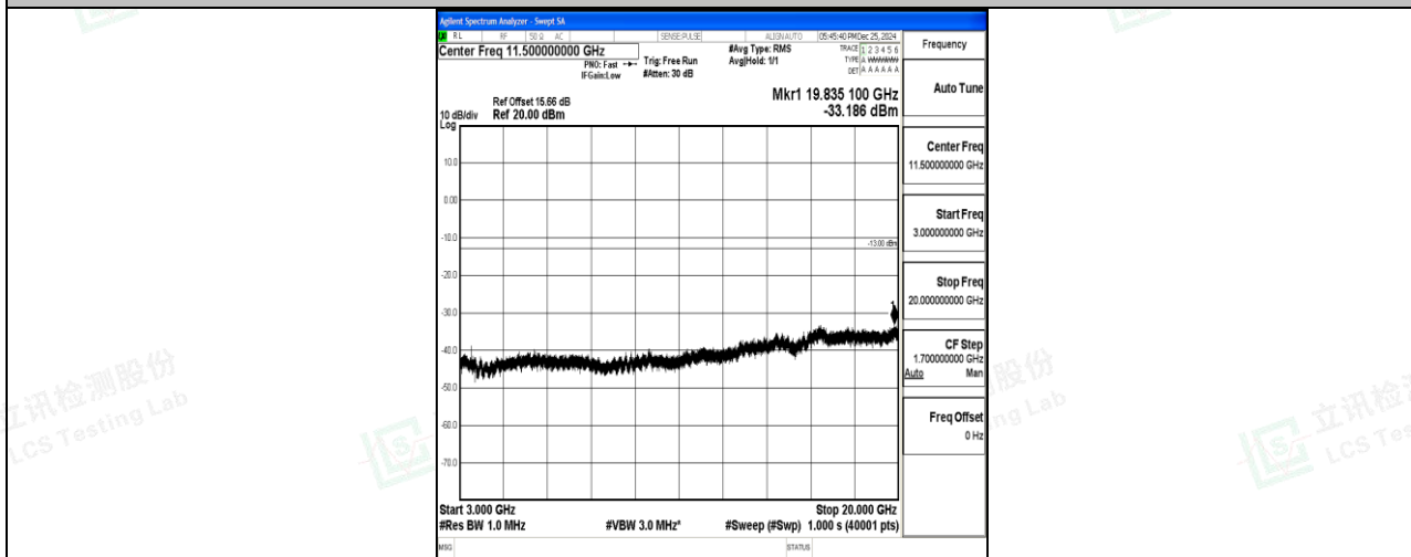
Band4_15MHz_QPSK_20175_1RB#0_3000~20000_3000~20000
