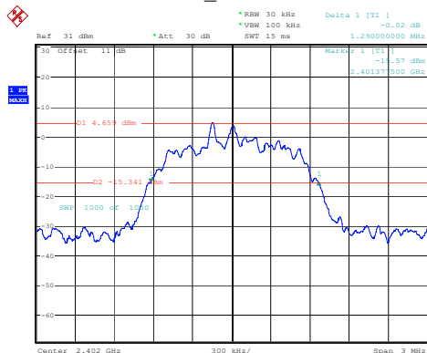
2DH1_Low 1.290MHz
