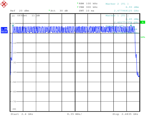
2DH1_Hopping 79
