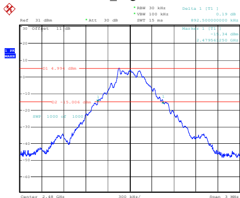
DH1_High 0.893MHz
