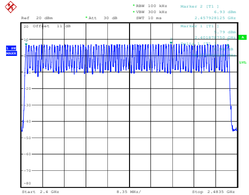
DH1_Hopping 79
