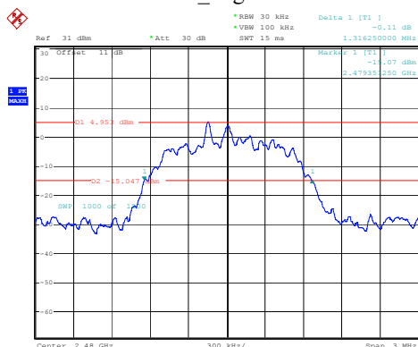
2DH1_High 1.316MHz
