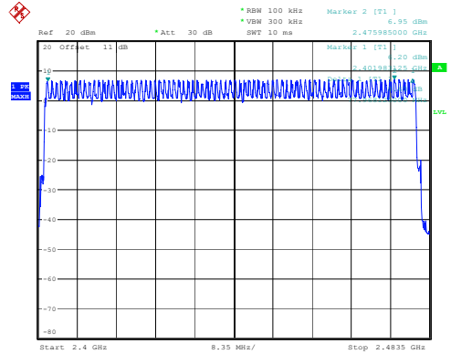
3DH1_Hopping 79
