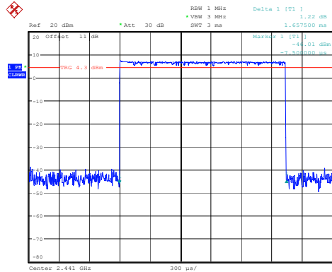
2DH3_Hopping 1.658ms
