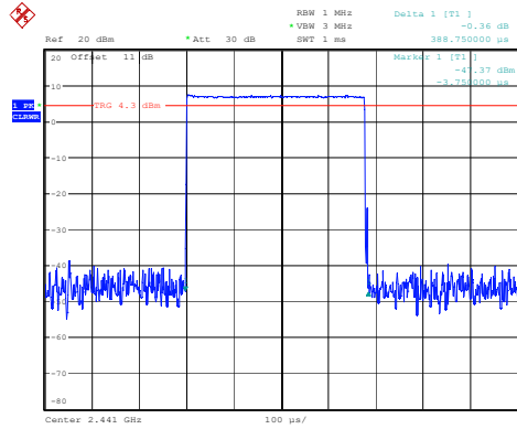
DH1_Hopping 0.389ms
