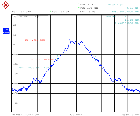
DH1_Middle 0.889MHz
