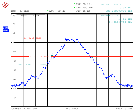
DH1_Low 0.986MHz
