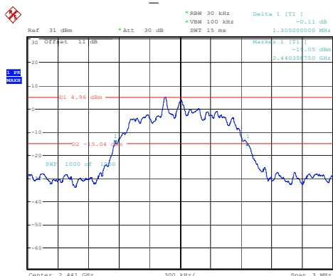
2DH1_Middle 1.305MHz
