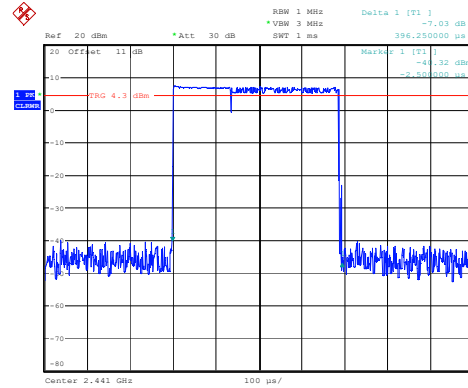
2DH1_Hopping 0.396ms
