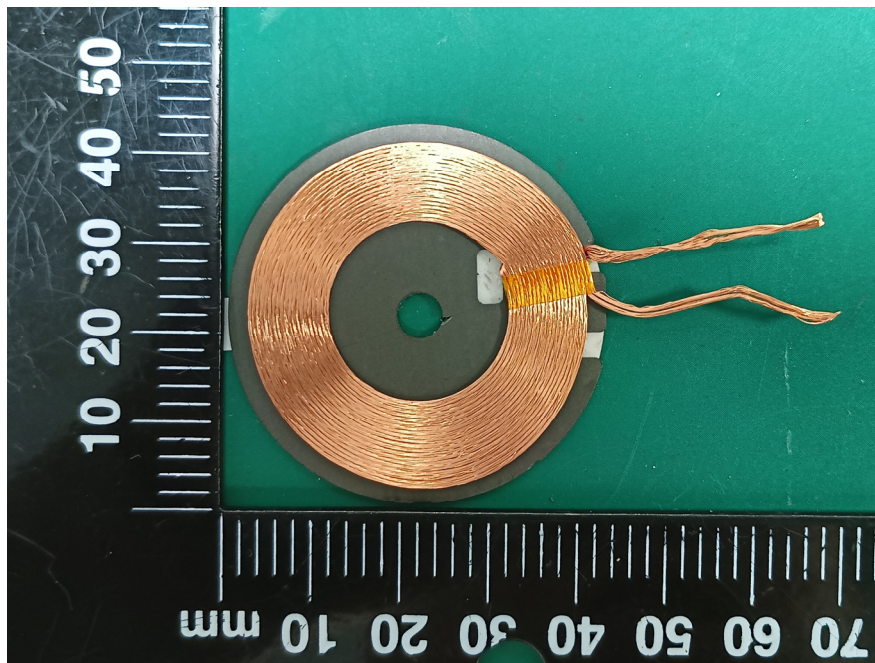
Coil Antenna
