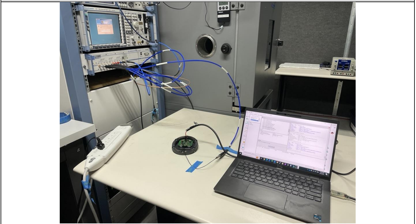
Conducted Power Measurement
