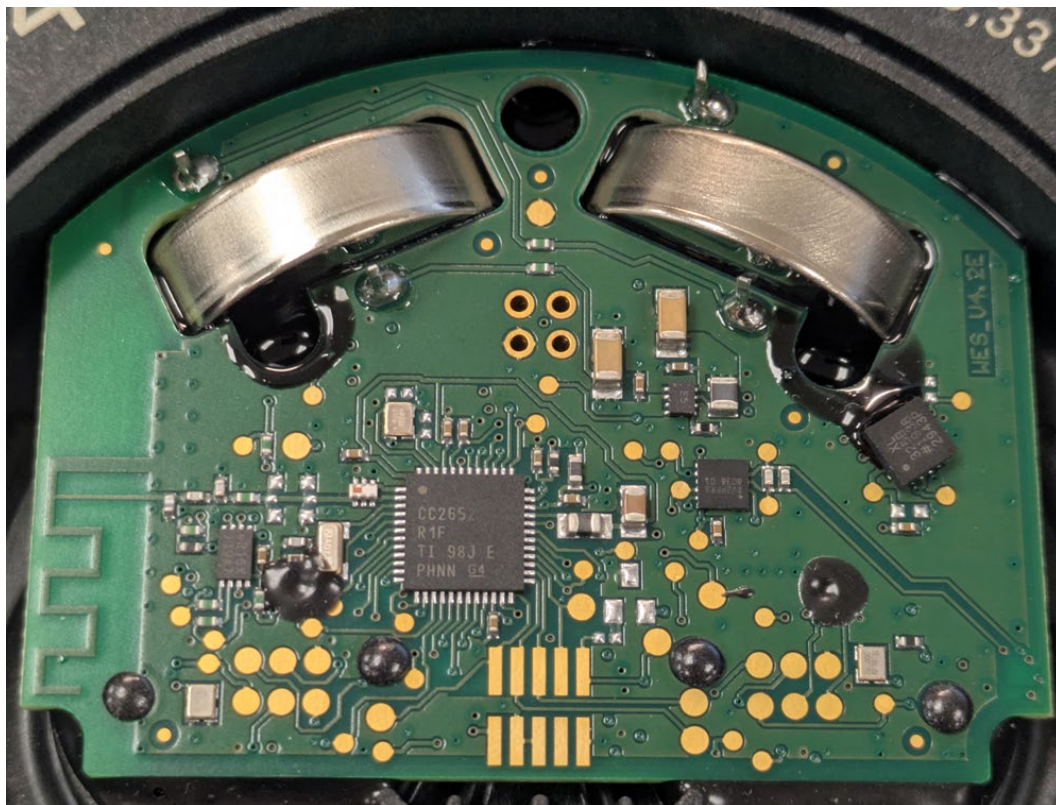
PCB Front
