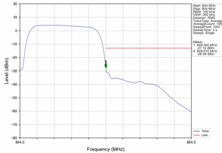
Band5_HSUPA_HCH_846.6MHz_Subtest 1_NTNV
