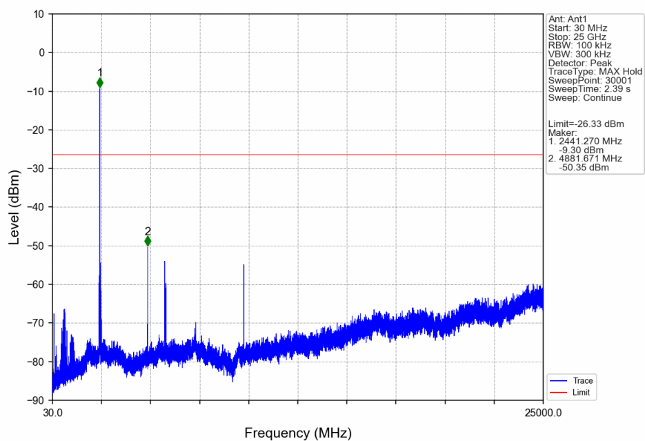
Pi/4DQPSK 2DH5_MCH_2441MHz_Ant1_NTN
