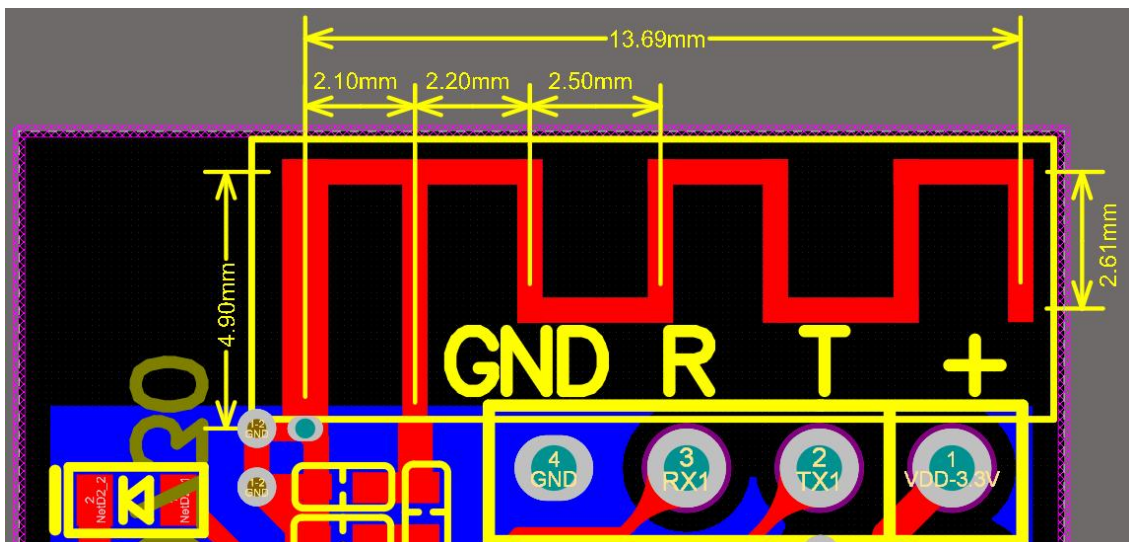
Antenna Photo &amp; Length (mm)
