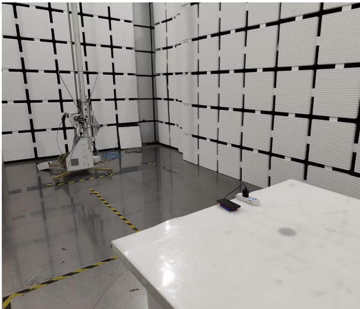
Radiated Emission below 1GHz-AC adapter charge mode
