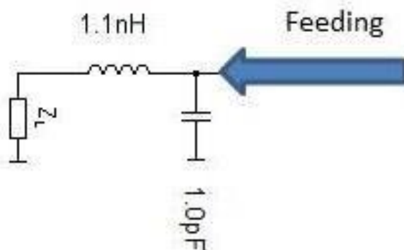
Suggested Matching Circuit
