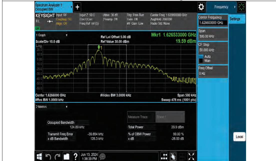
Band255-15kHz-OBW-L-BPSK-1@1
