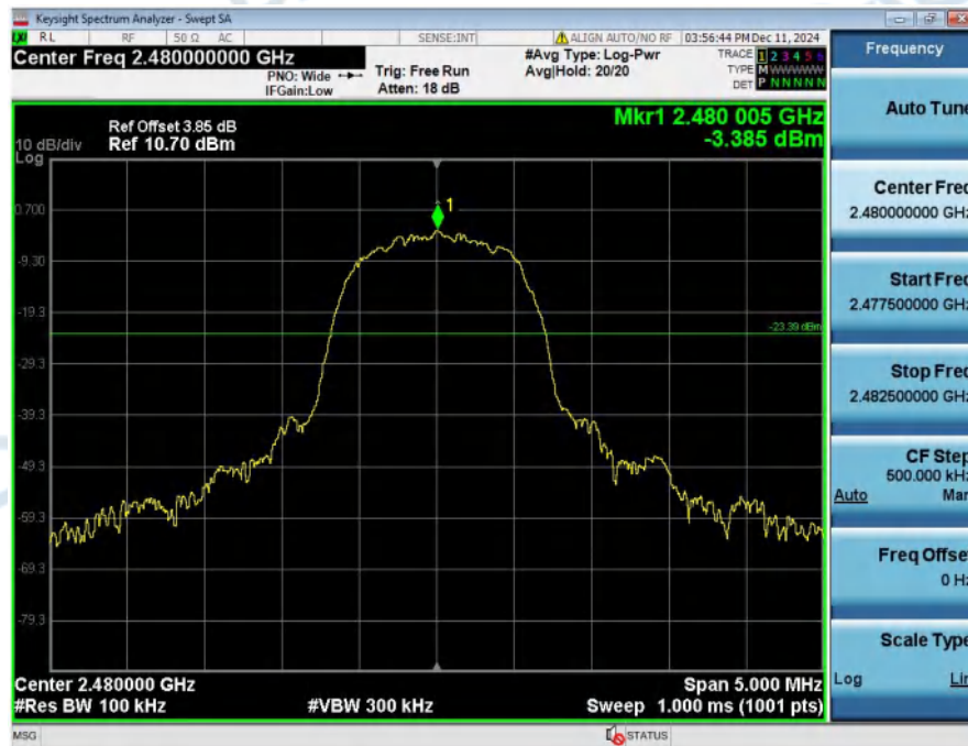
2_Spurious_Emissions_NVNT_ANT1_3-DH5_2480_00
