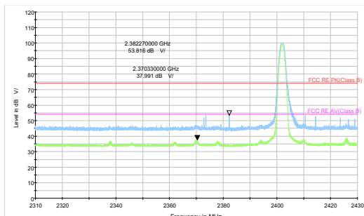
nRF 2.4GHz-Channel 0 Peak+ Average
