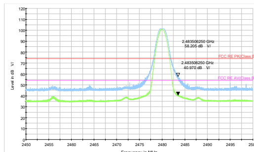
nRF 2.4GHz--Channel 39 Peak+ Average
