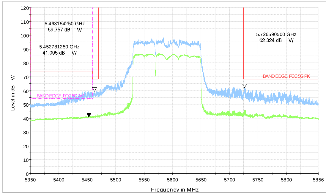
Wi-Fi 5GHz_BE160 996+484Tone HIGH_CH114
