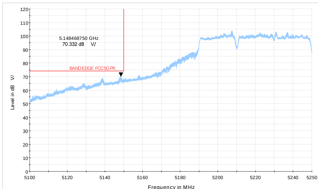
Wi-Fi 5GHz_BE80 484+242Tone HIGH_CH42
