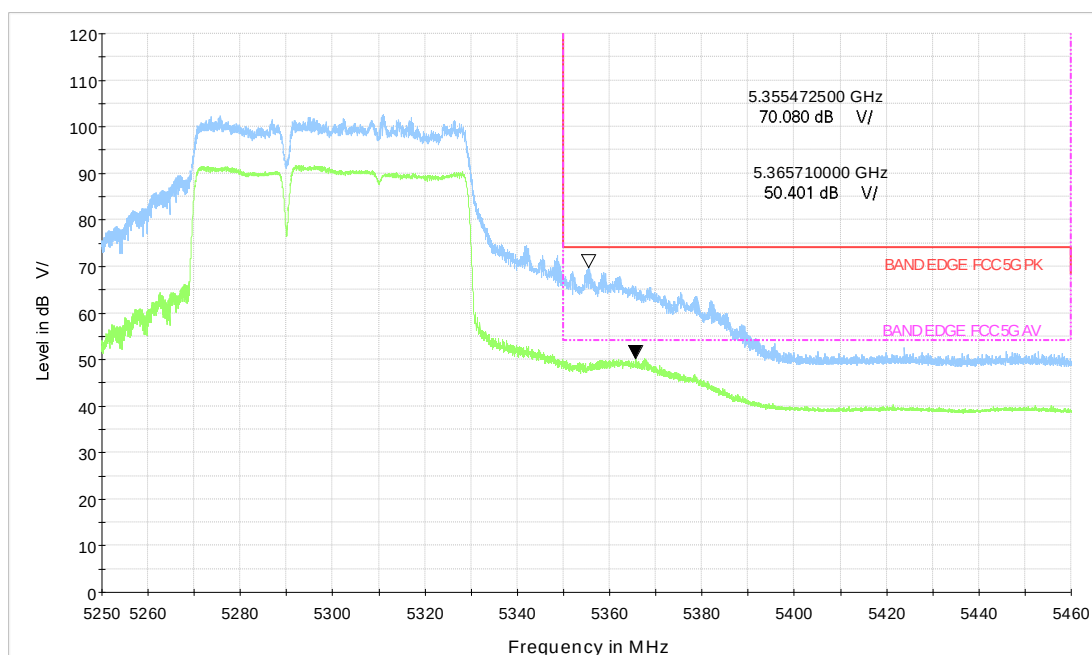
Wi-Fi 5GHz_BE80 484+242Tone HIGH_CH58
