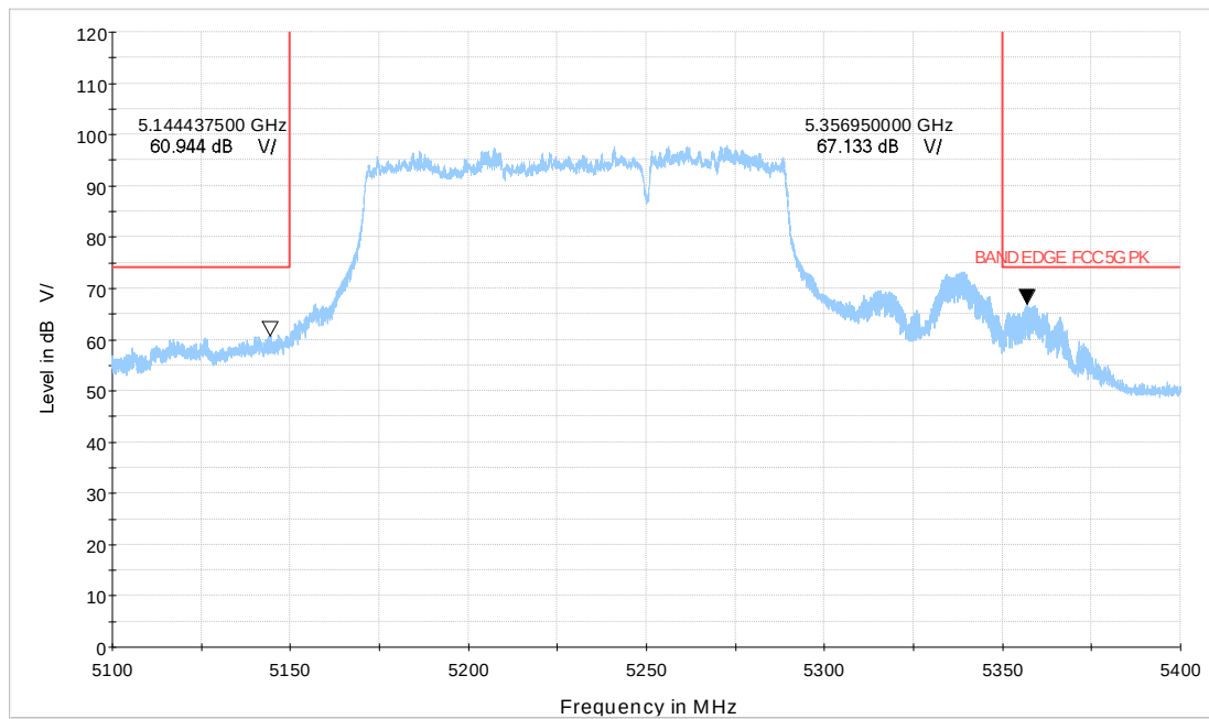
Wi-Fi 5GHz_BE160 996+484Tone LOW_CH50
