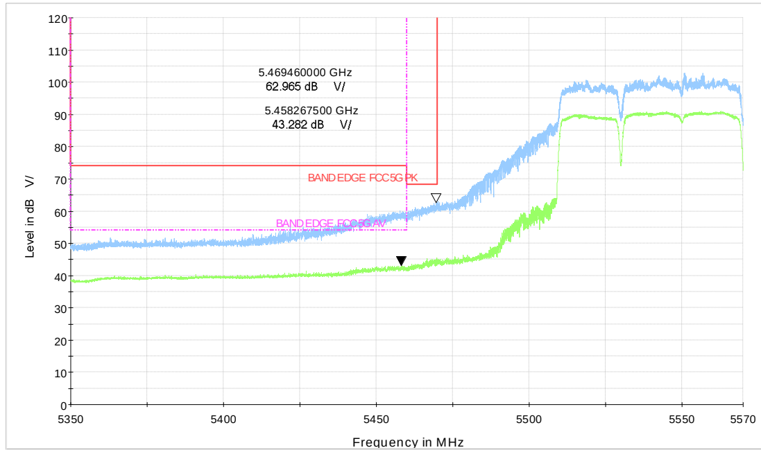
Wi-Fi 5GHz_BE80 484+242Tone HIGH_CH106
