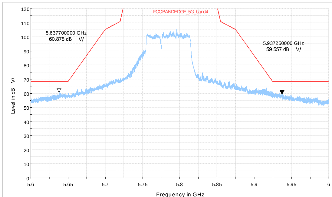
Wi-Fi 5GHz_BE80 484+242Tone HIGH_CH155
