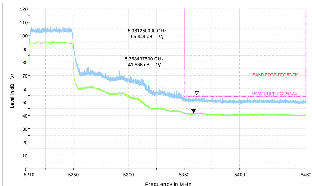
Wi-Fi 5GHz_ax40 CH46
