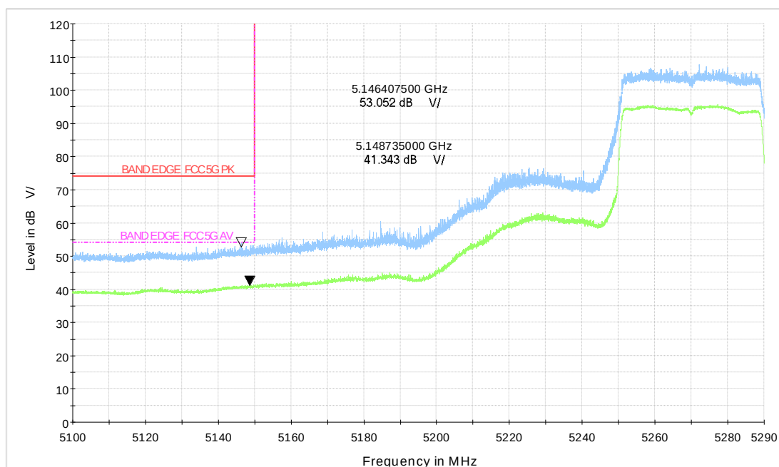
Wi-Fi 5GHz_ax40 CH54
