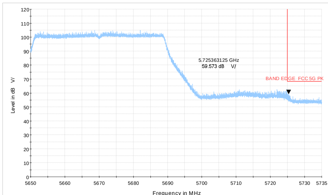
Wi-Fi 5GHz_ax40 CH134
