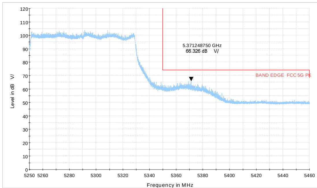
Wi-Fi 5GHz TB_BE80 CH58_996Tone
