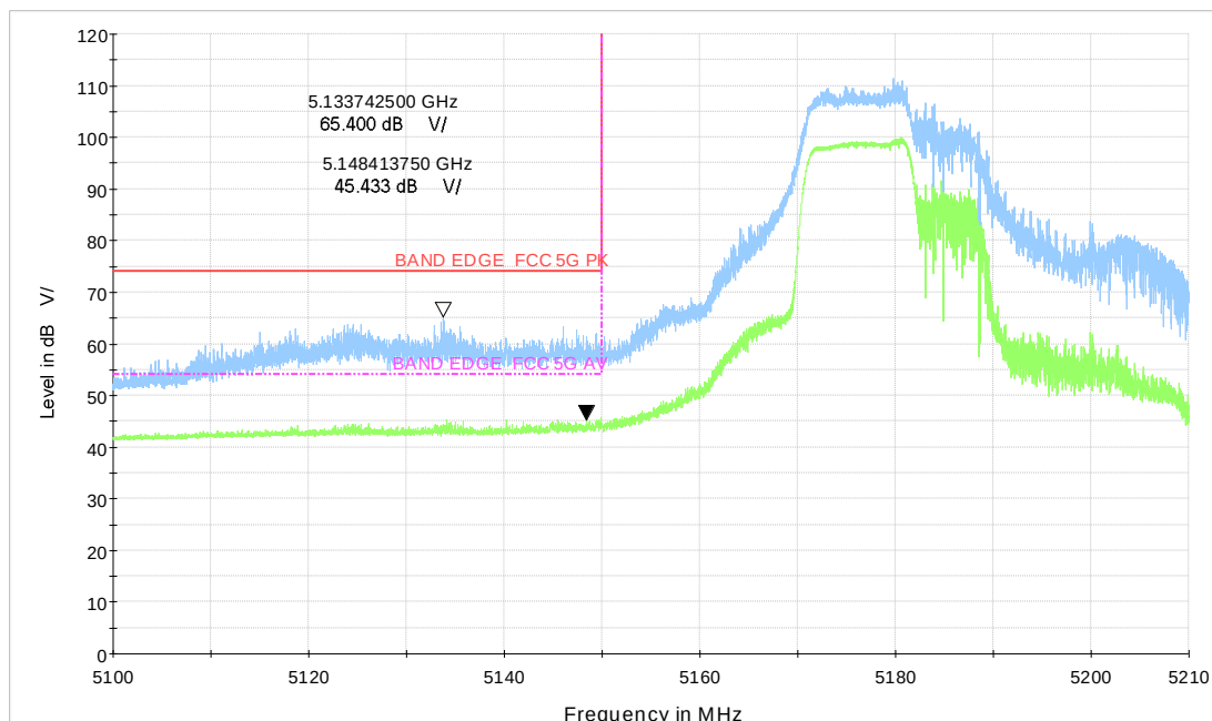
Wi-Fi 5GHz_BE40 106+26Tone LOW_CH38
