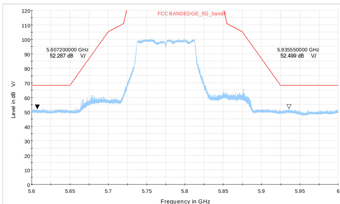
Wi-Fi 5GHz_ac80 CH155
