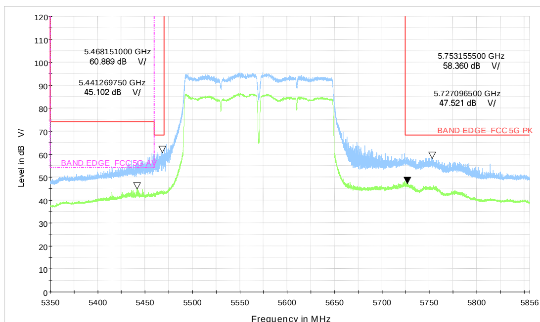
Wi-Fi 5GHz_ac160 CH114
