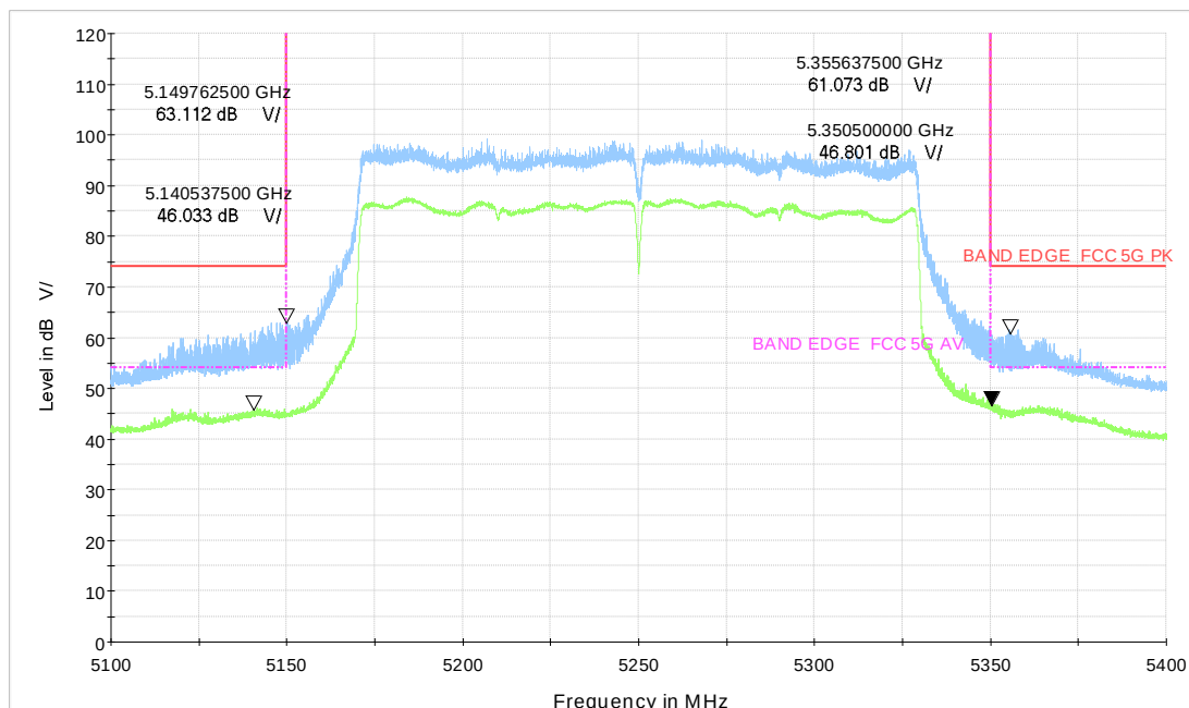
Wi-Fi 5GHz TB_ax160 CH50_996x2Tone
