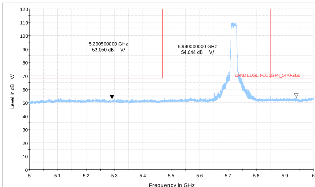
Wi-Fi 5GHz_BE20 CH144
