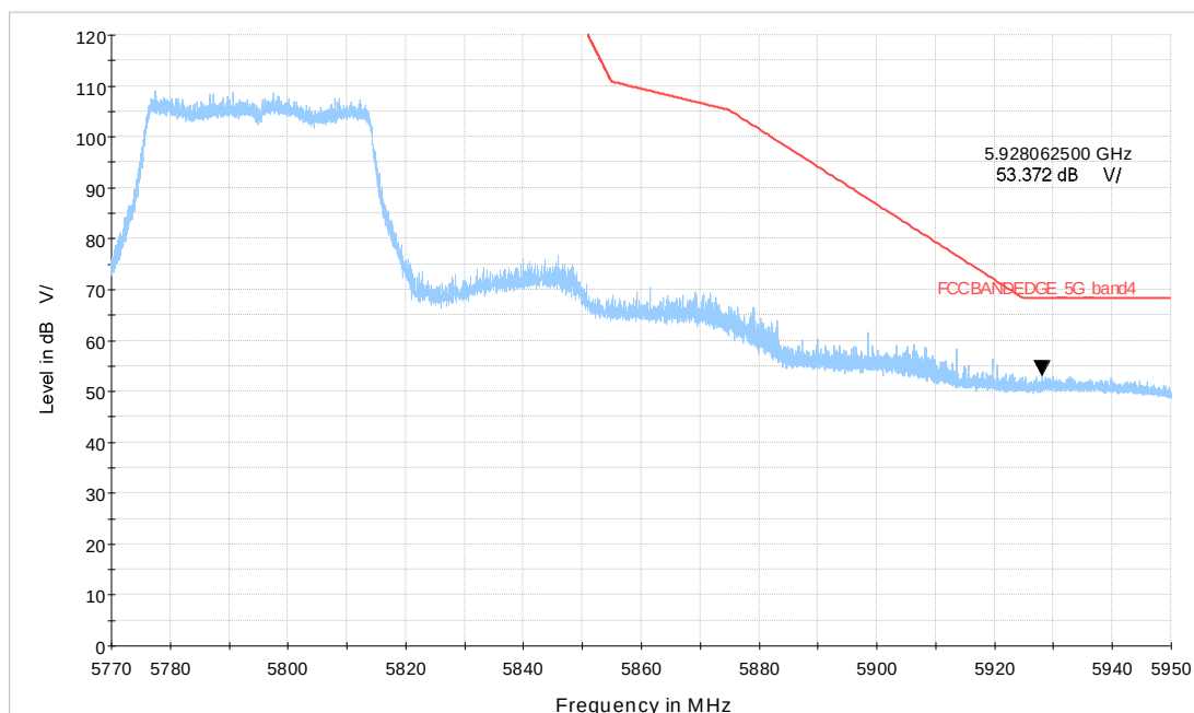
Wi-Fi 5GHz_ax40 CH159
