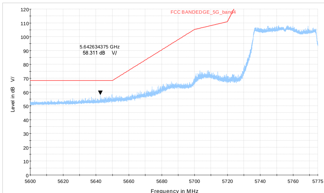
Wi-Fi 5GHz TB_ax40 CH151_484Tone
