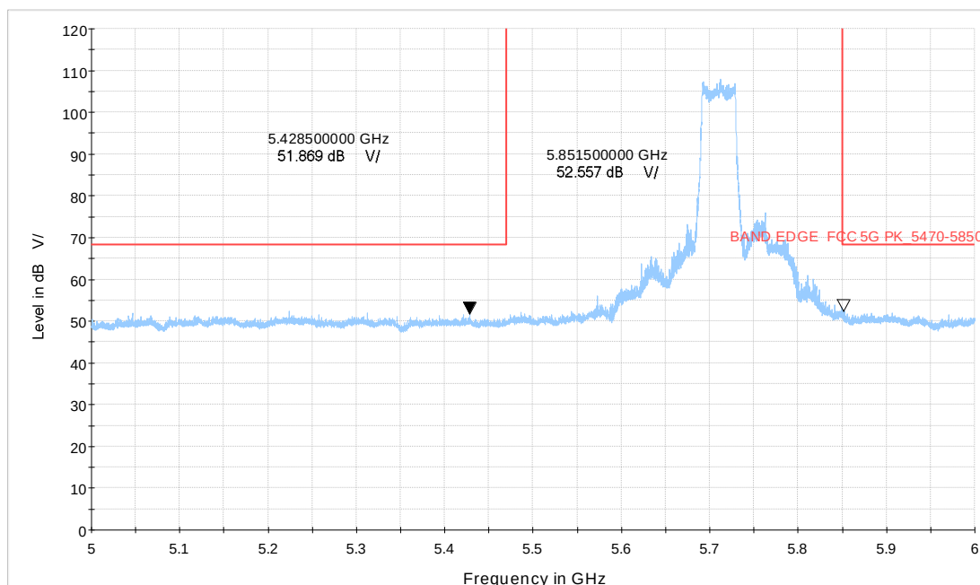
Wi-Fi 5GHz_ax40 CH142
