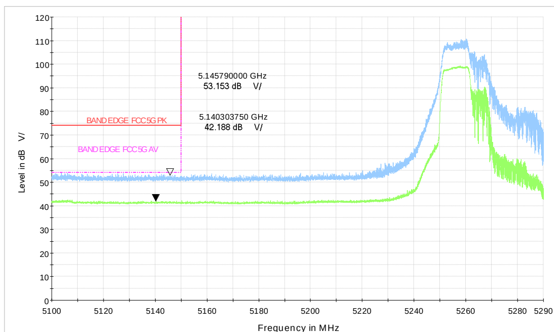
Wi-Fi 5GHz_BE40 106+26Tone LOW_CH54
