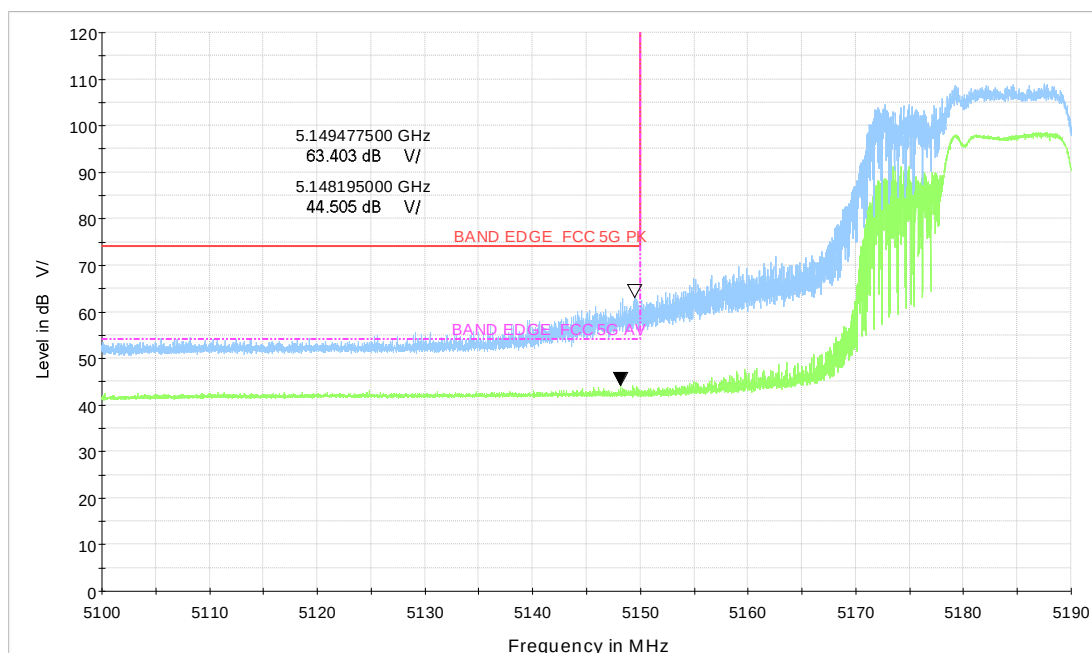
Wi-Fi 5GHz_BE20 106+26Tone HIGH_CH36
