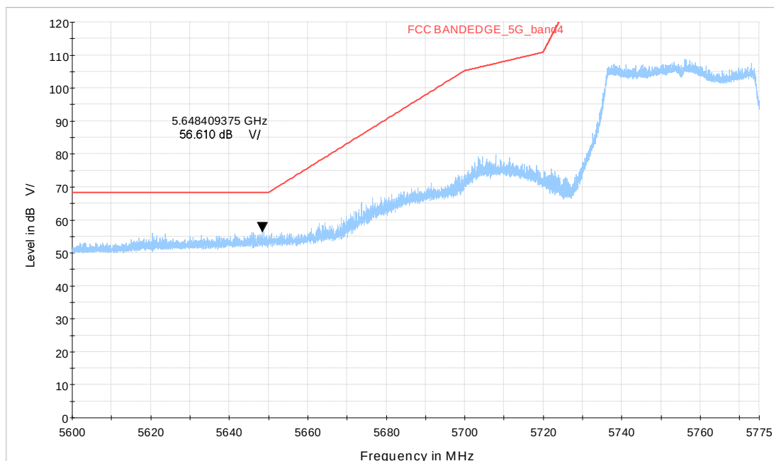
Wi-Fi 5GHz TB_BE40 CH151_484Tone
