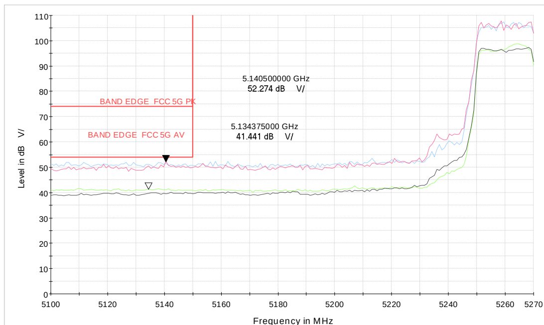
Wi-Fi 5GHz TB_ax20 CH52_242Tone
