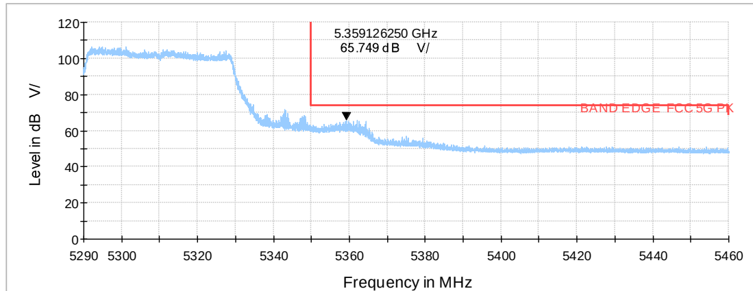
Wi-Fi 5GHz_ax40 CH62
