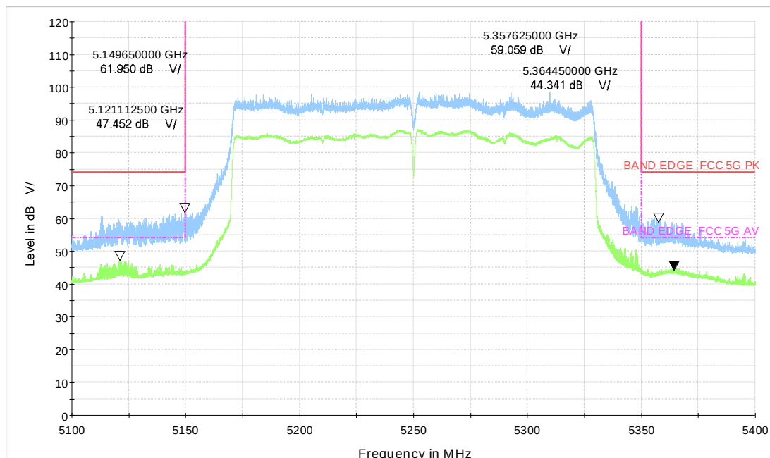
Wi-Fi 5GHz TB_BE160 CH50_996Tx2ONE
