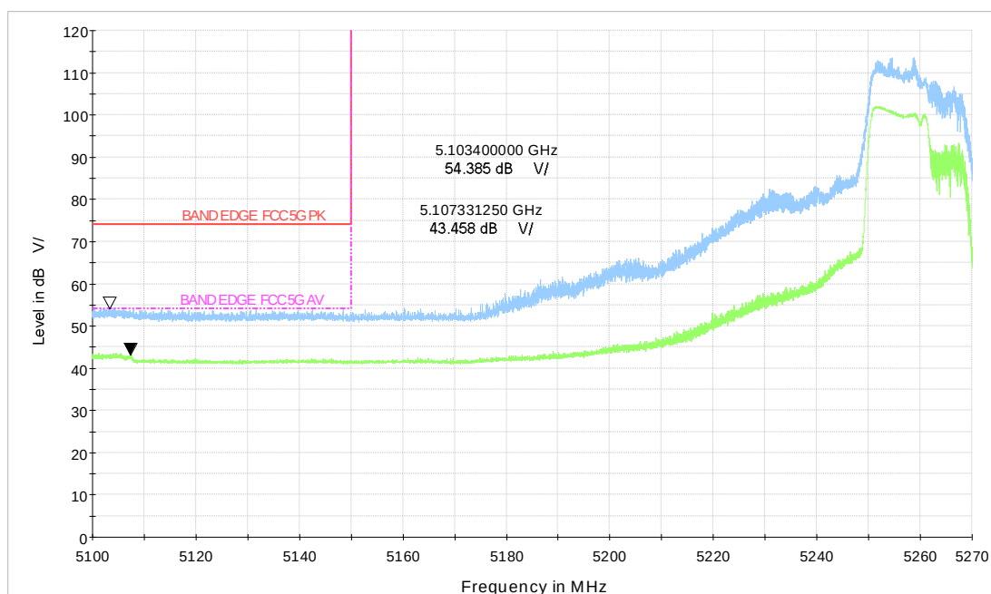
Wi-Fi 5GHz_BE20 106+26Tone LOW_CH52
