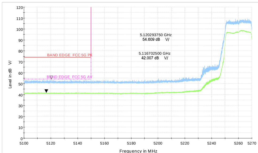
Wi-Fi 5GHz TB_BE20 CH52_242Tone
