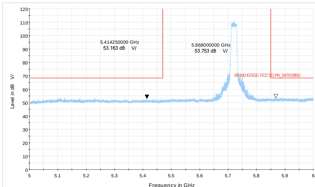
Wi-Fi 5GHz_ax20 CH144
