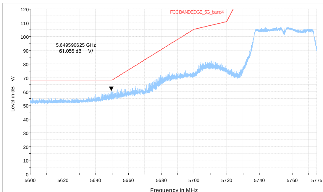
Wi-Fi 5GHz_n40 CH151
