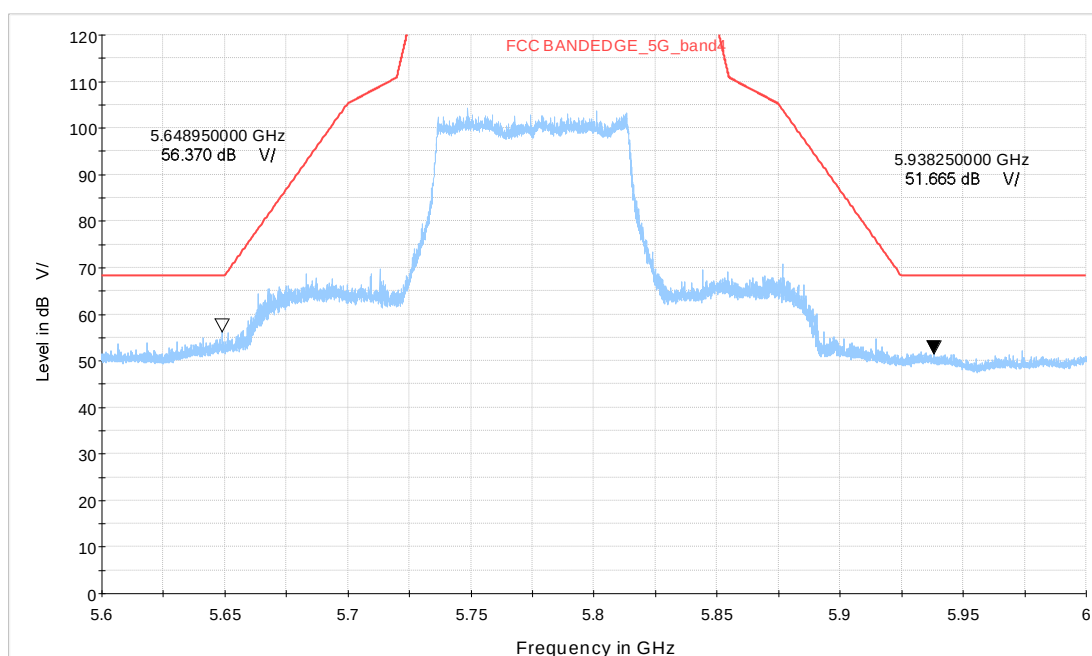
Wi-Fi 5GHz_BE80 CH155
