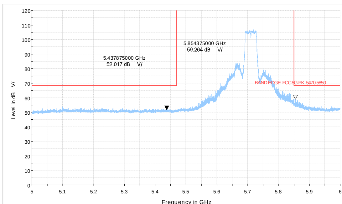
Wi-Fi 5GHz_n40 CH142
