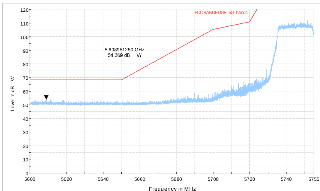
Wi-Fi 5GHz_ax20 CH149
