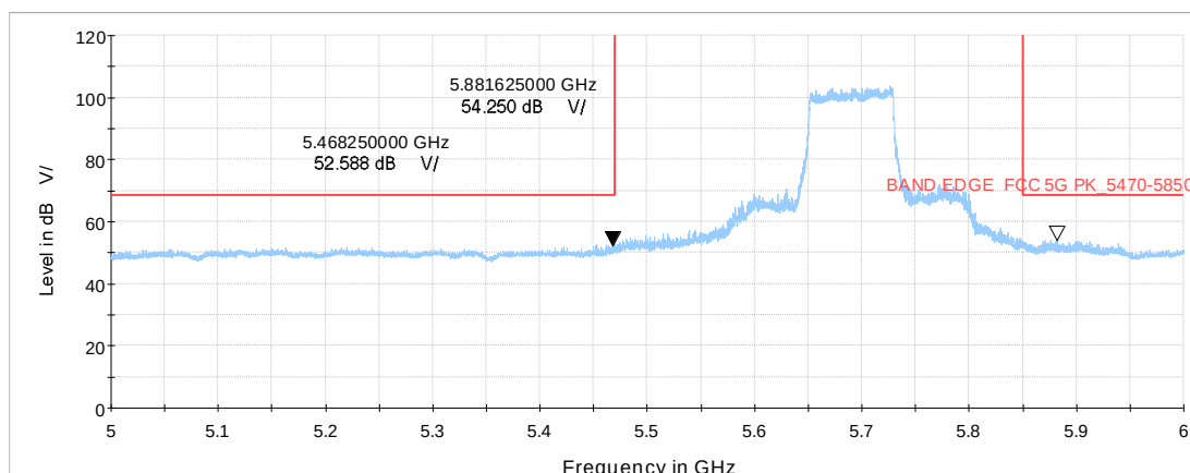
Wi-Fi 5GHz_BE80 CH138
