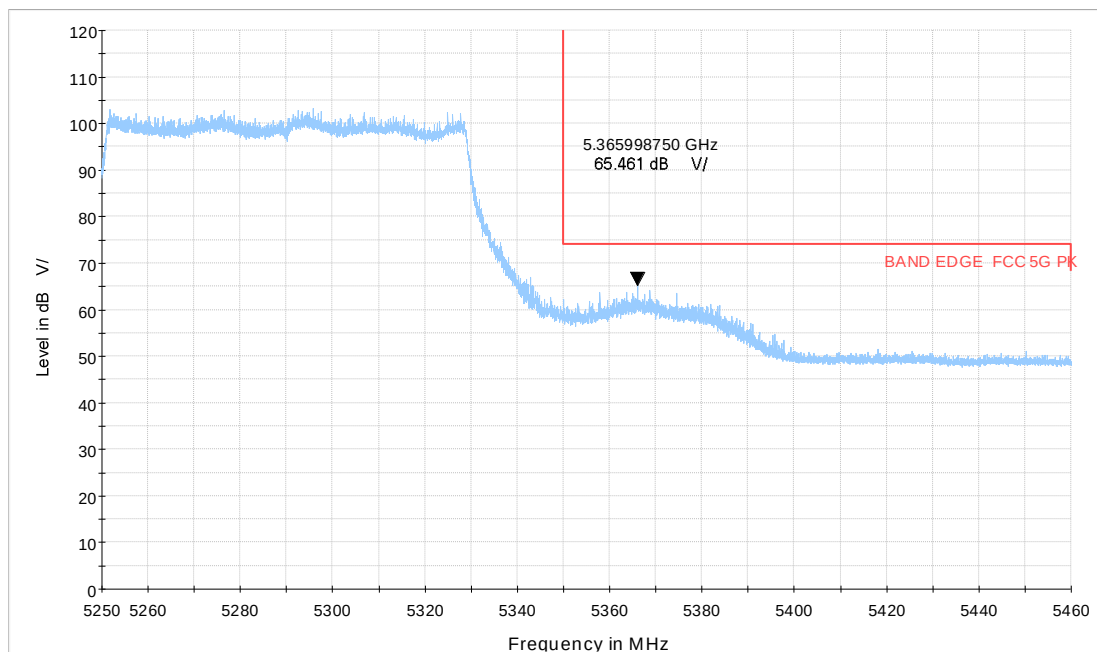
Wi-Fi 5GHz_BE80 CH58
