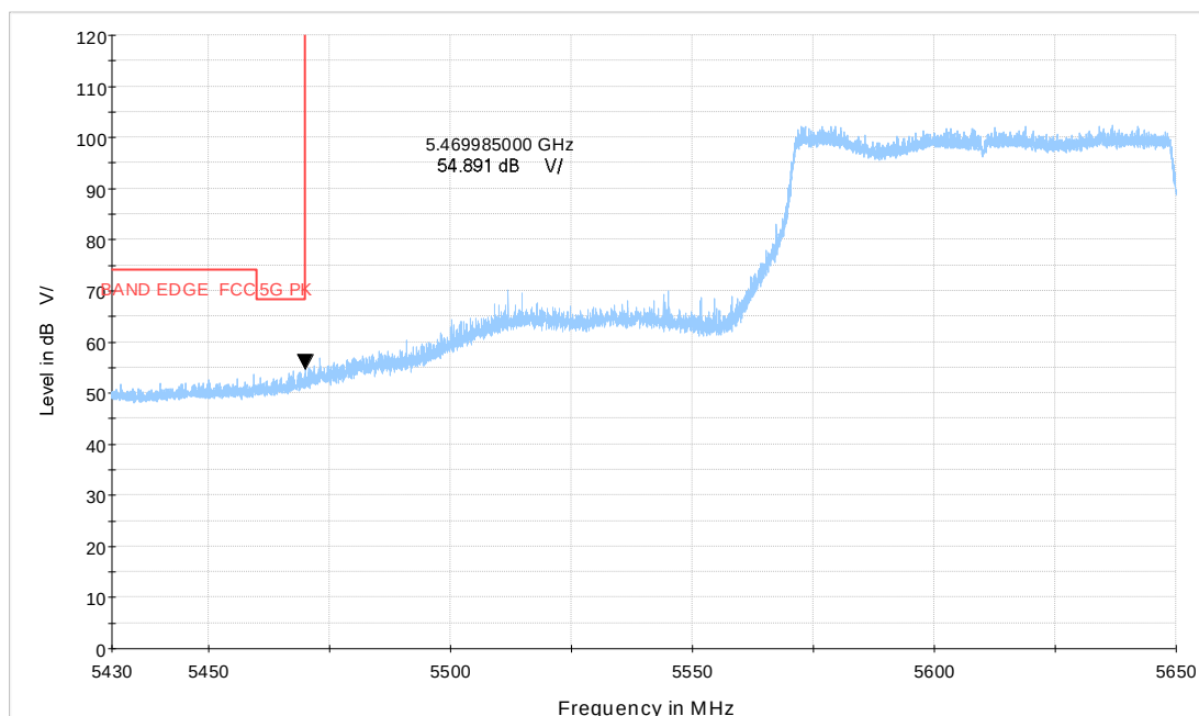
Wi-Fi 5GHz_ax80 CH122
