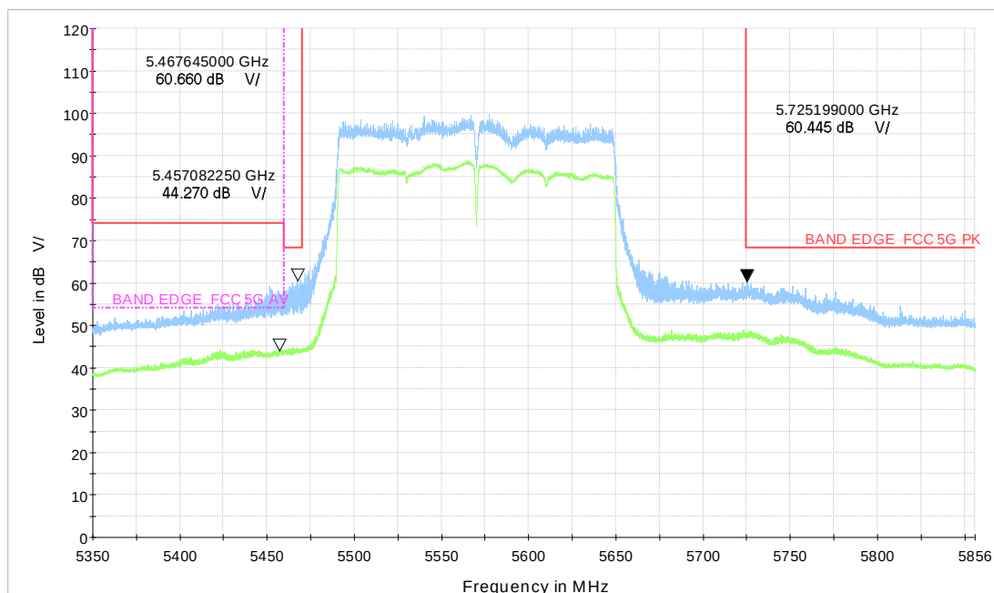
Wi-Fi 5GHz TB_ax160 CH114_996x2Tone
