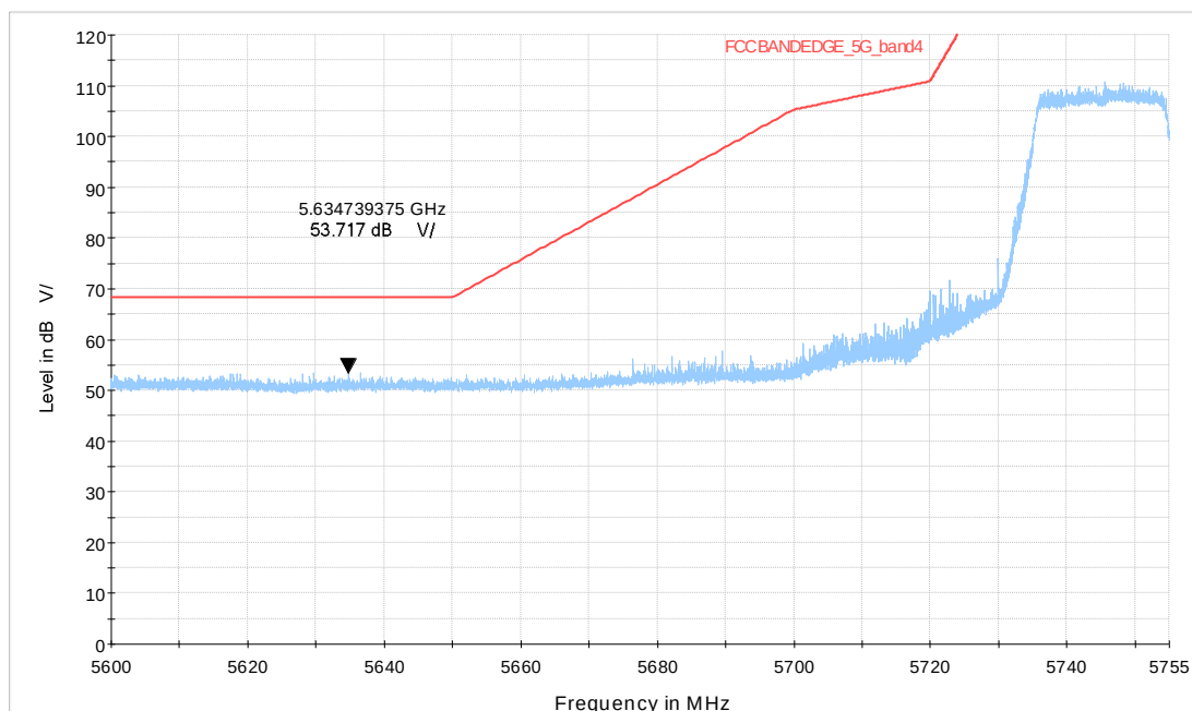
Wi-Fi 5GHz_BE20 CH149
