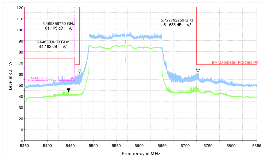
Wi-Fi 5GHz_BE160 CH114
