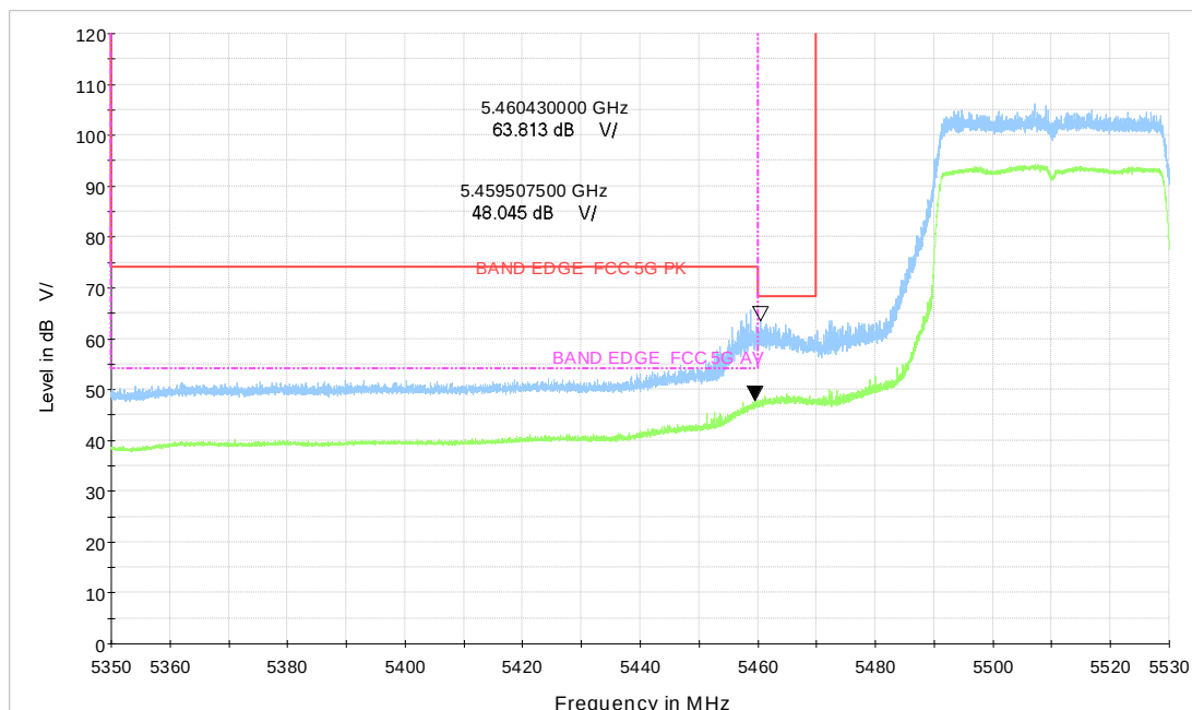
Wi-Fi 5GHz TB_BE40 CH102_484Tone
