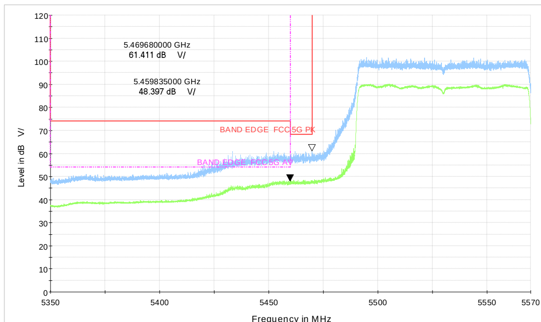
Wi-Fi 5GHz_BE80 CH106
