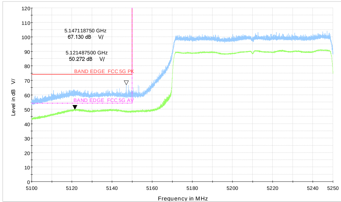
Wi-Fi 5GHz TB_BE80 CH42_996Tone
