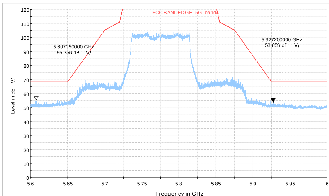
Wi-Fi 5GHz TB_BE80 CH155_996Tone
