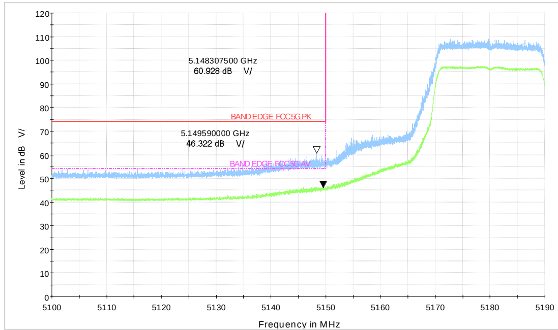
Wi-Fi 5GHz_BE20 CH36
