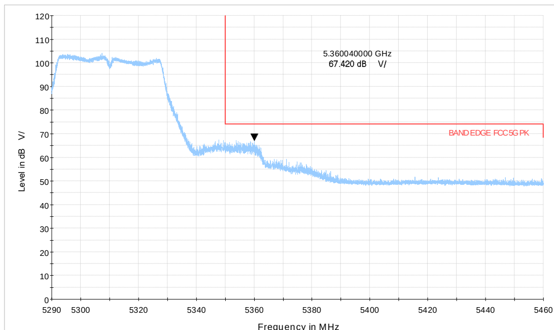
Wi-Fi 5GHz_n40 CH62
