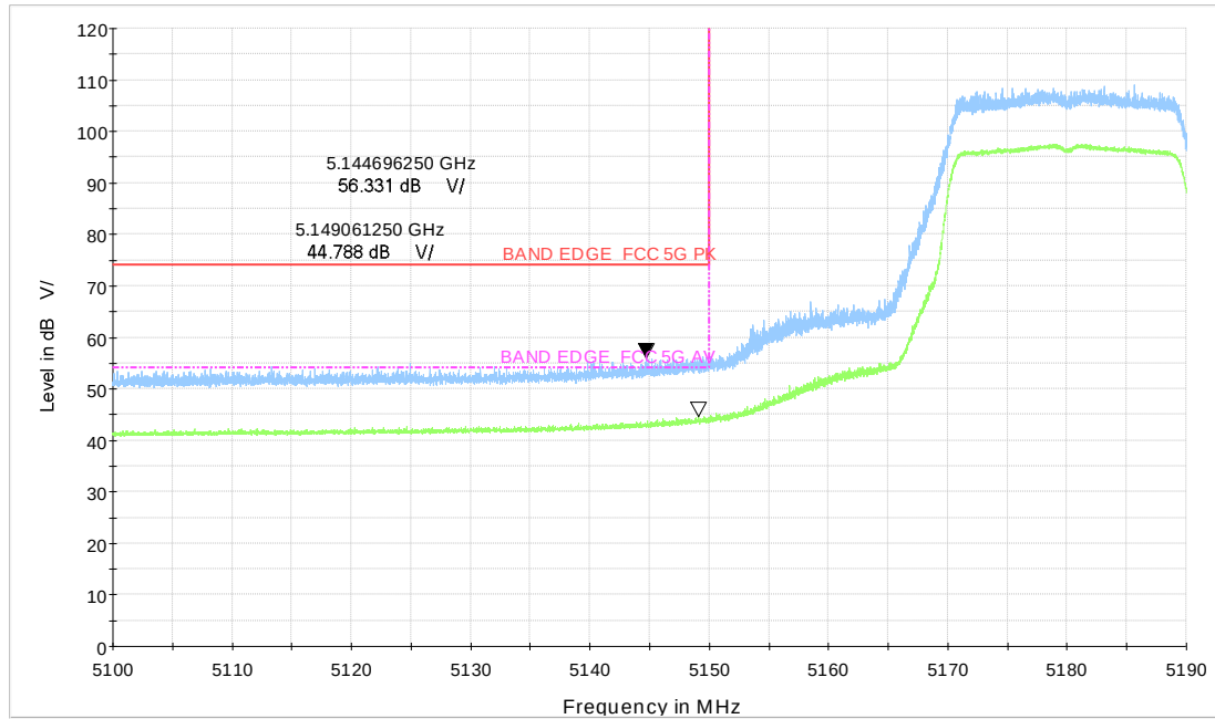
Wi-Fi 5GHz TB_BE20 CH36_242Tone
