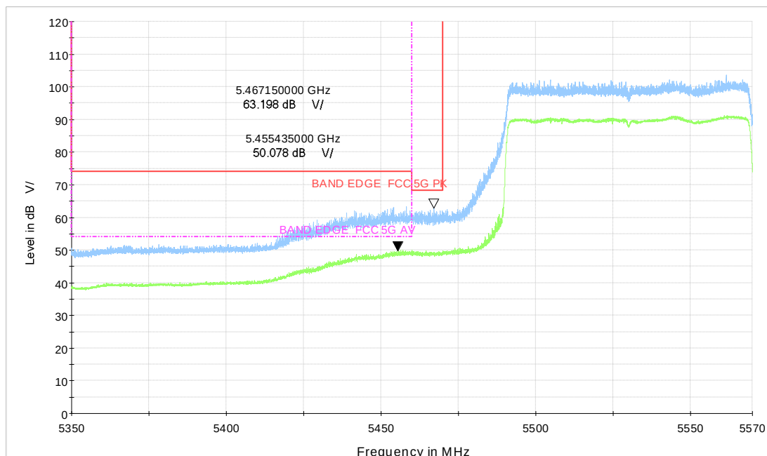
Wi-Fi 5GHz TB_BE80 CH106_996Tone
