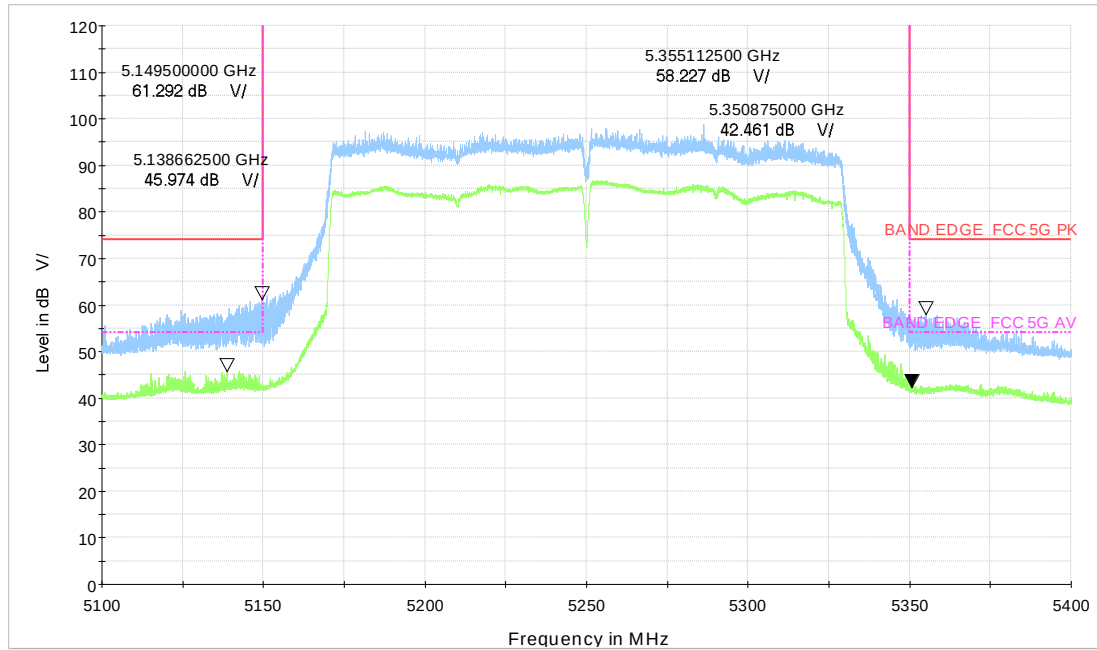
Wi-Fi 5GHz_BE160 CH50
