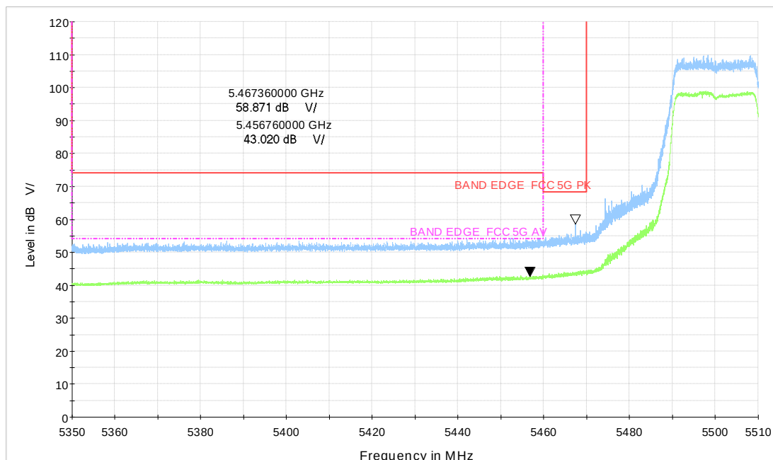
Wi-Fi 5GHz TB_ax20 CH100_242Tone
