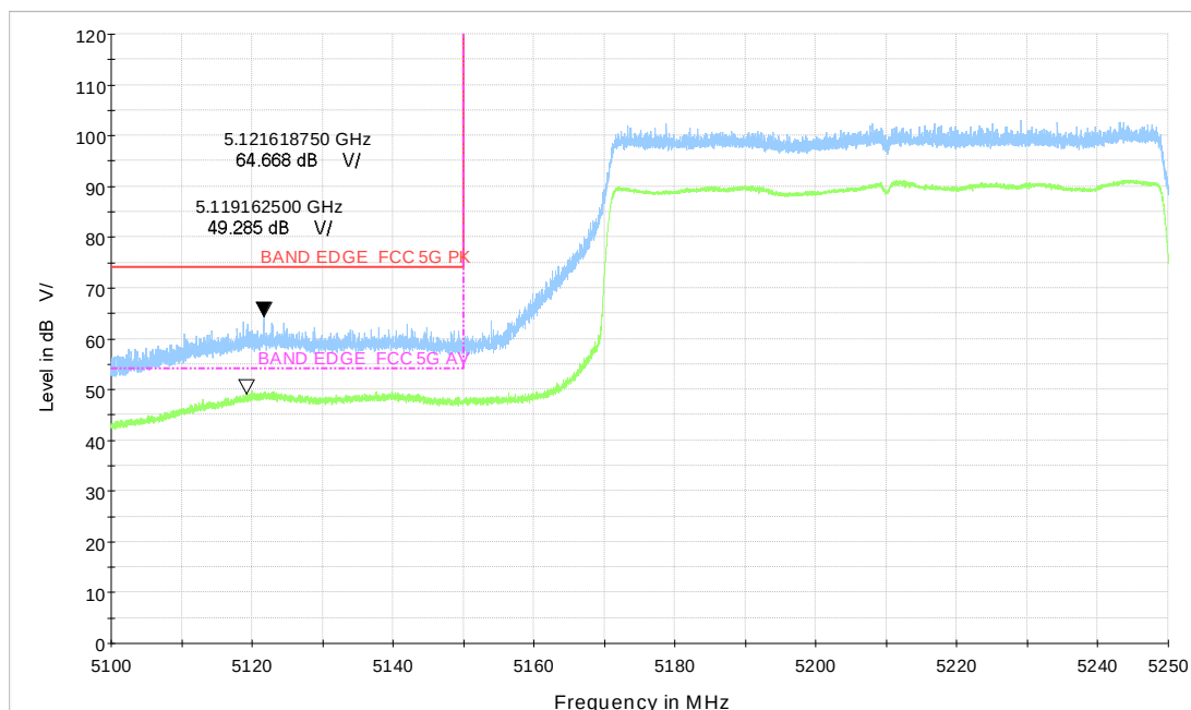
Wi-Fi 5GHz TB_ax80 CH42_996Tone
