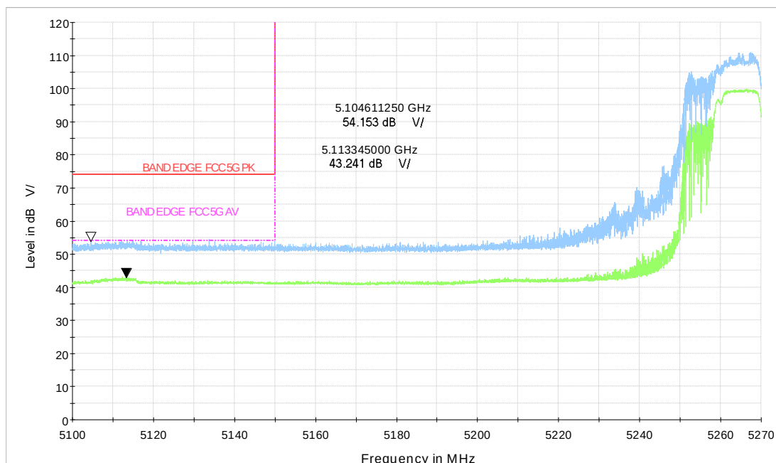
Wi-Fi 5GHz_BE20 106+26Tone HIGH_CH52
