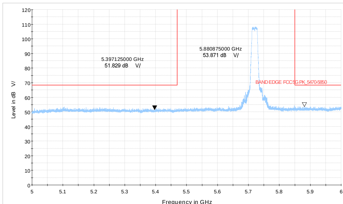
Wi-Fi 5GHz_n20 CH144
