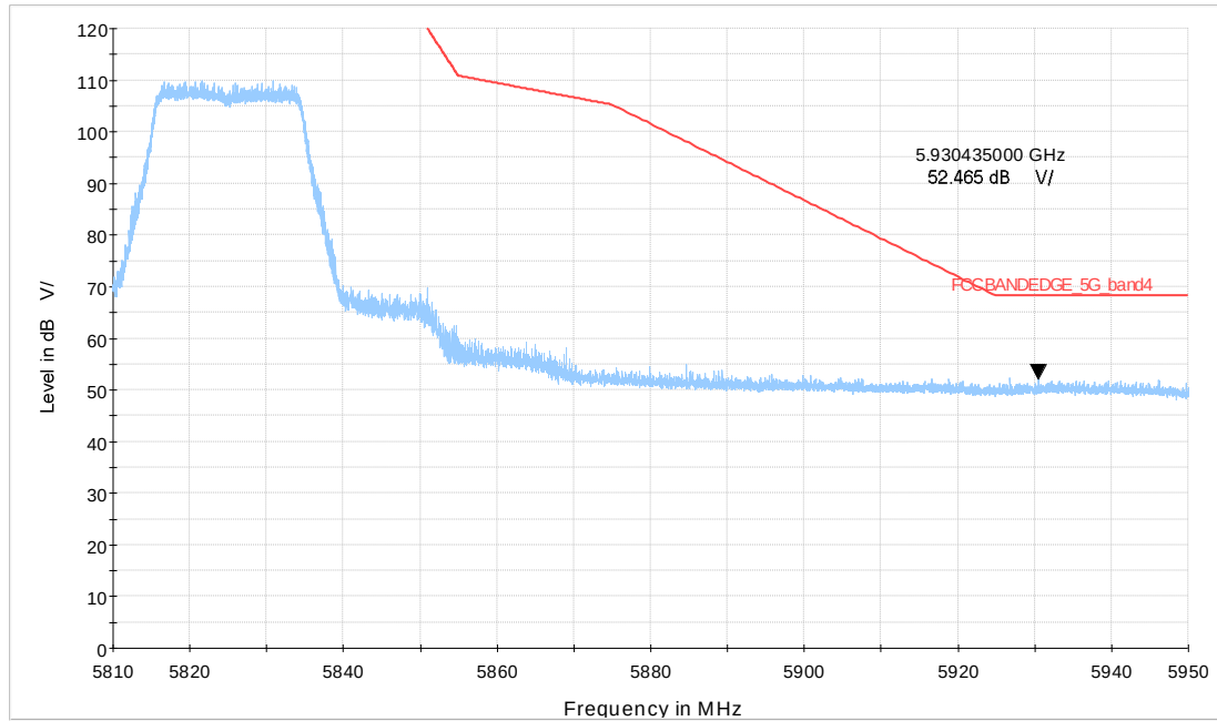
Wi-Fi 5GHz_BE20 CH165
