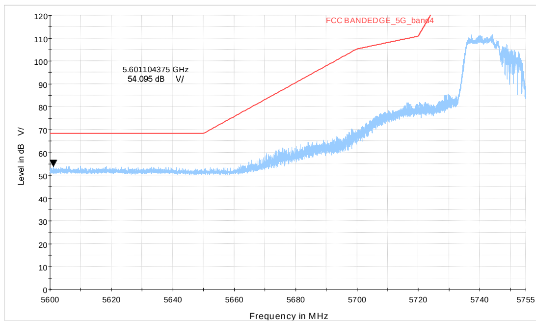
Wi-Fi 5GHz_BE20 106+26Tone LOW_CH149
