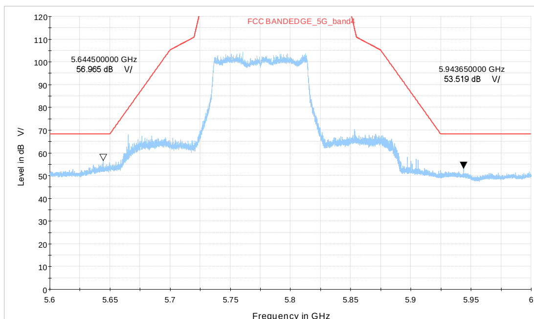
Wi-Fi 5GHz_ax80 CH155
