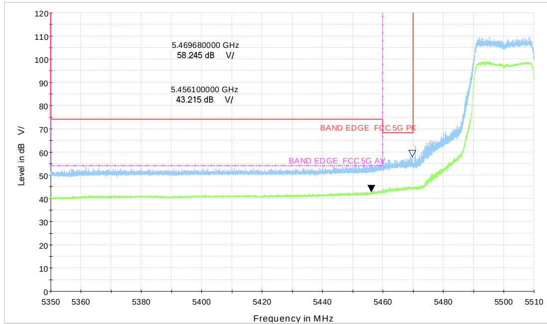
Wi-Fi 5GHz TB_BE20 CH100_242Tone
