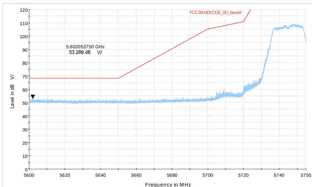
Wi-Fi 5GHz_n20 CH149
