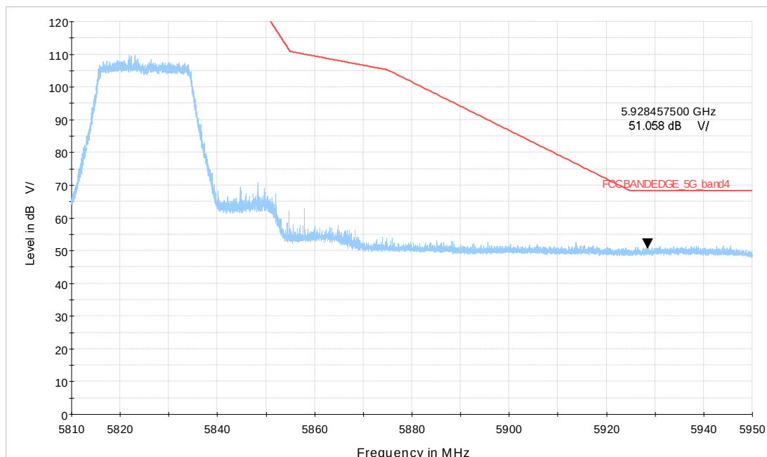
Wi-Fi 5GHz_ax20 CH165
