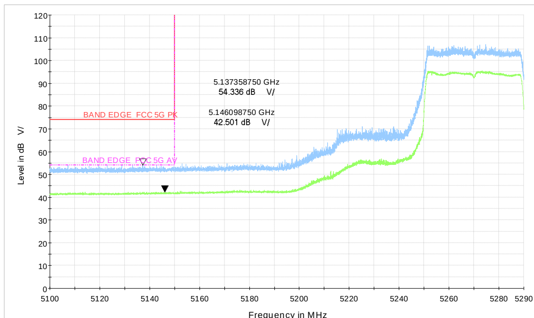
Wi-Fi 5GHz TB_ax40 CH54_484Tone
