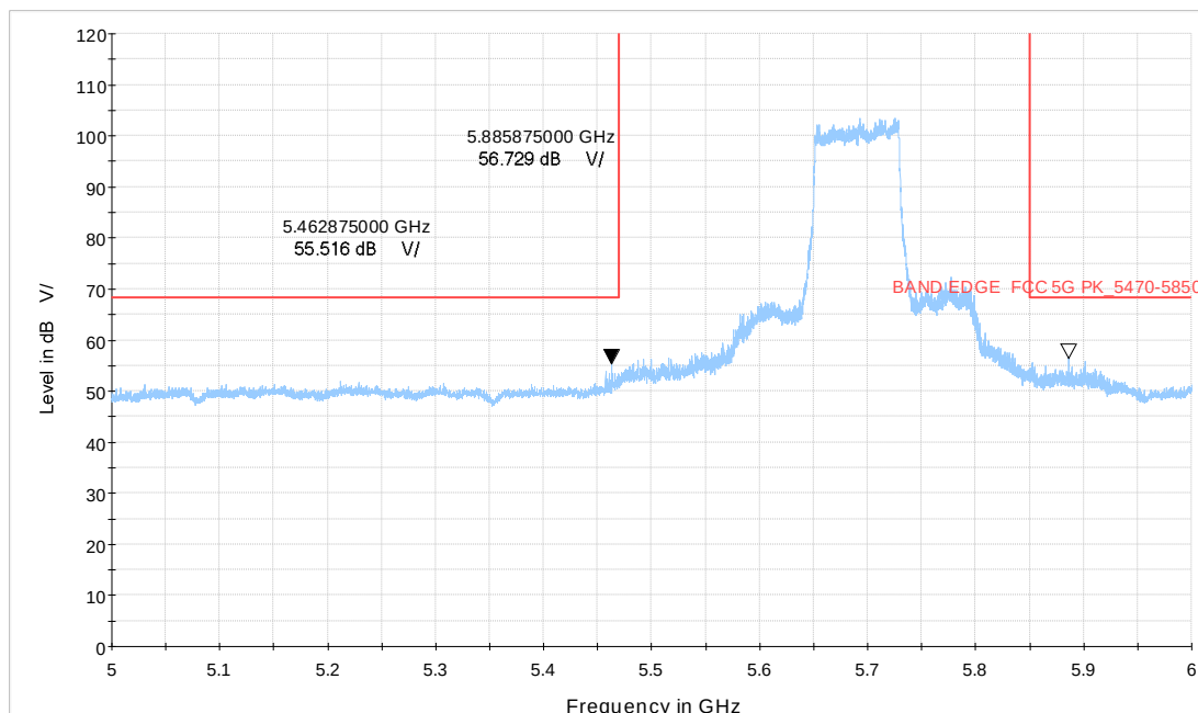
Wi-Fi 5GHz_ax80 CH138
