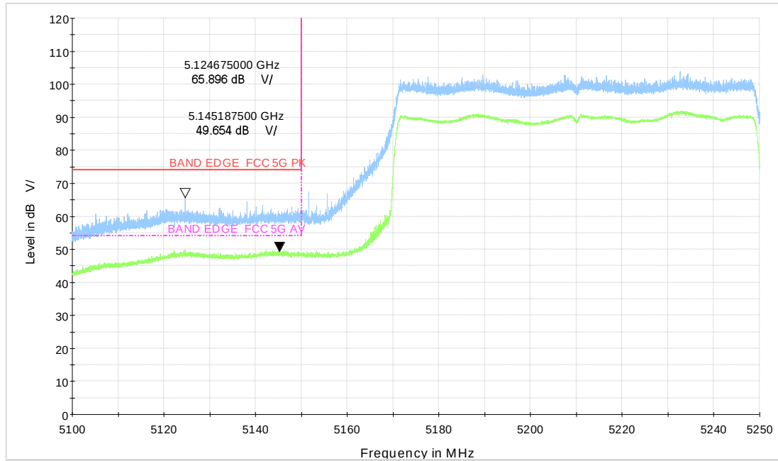
Wi-Fi 5GHz_BE80 CH42
