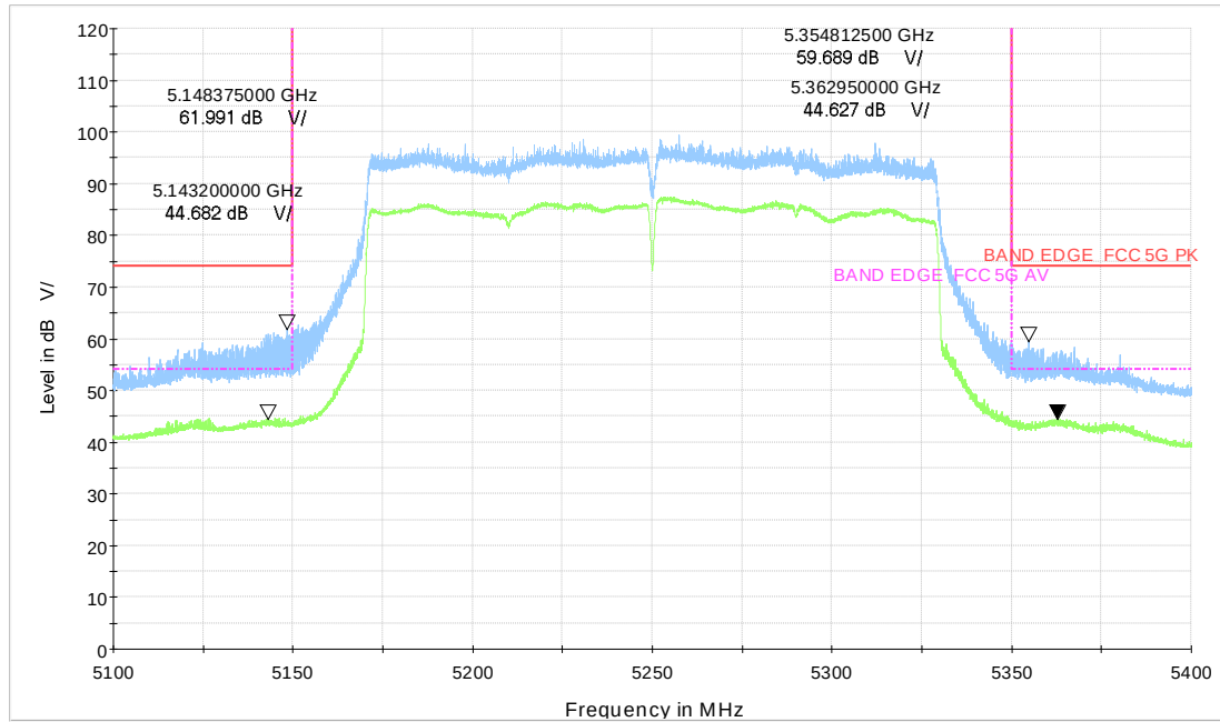
Wi-Fi 5GHz_ax160 CH50
