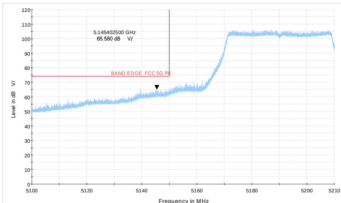
Wi-Fi 5GHz TB_BE40 CH38_484Tone
