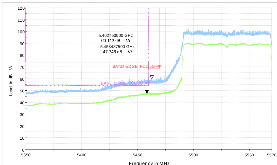
Wi-Fi 5GHz_ax80 CH106
