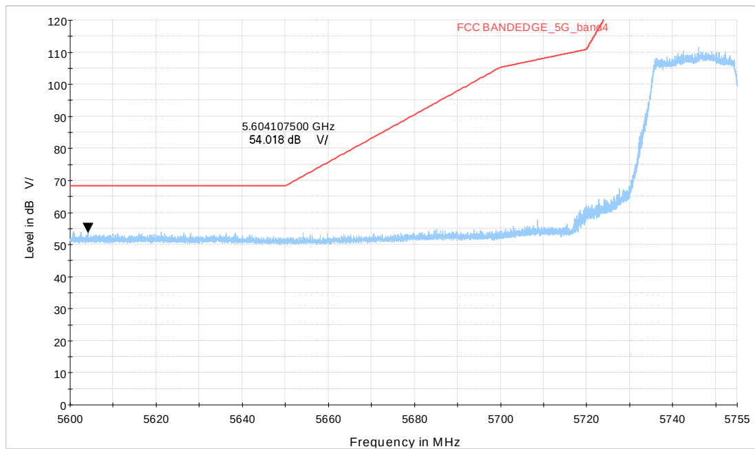
Wi-Fi 5GHz TB_BE20 CH149_242Tone
