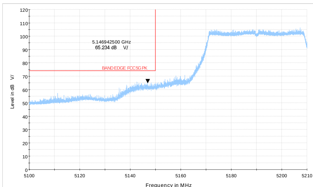
Wi-Fi 5GHz_ax40 CH38
