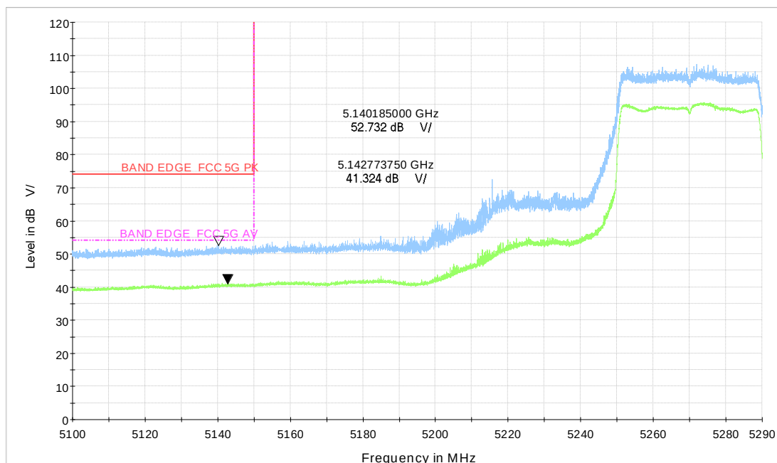
Wi-Fi 5GHz TB_BE40 CH54_484Tone
