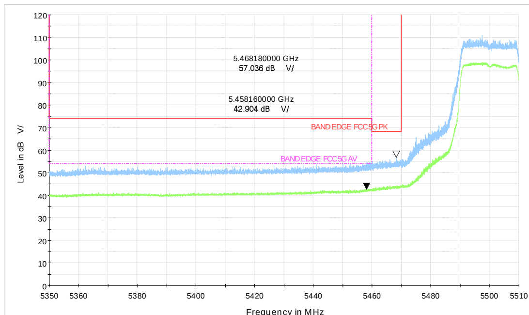
Wi-Fi 5GHz_BE20 CH100
