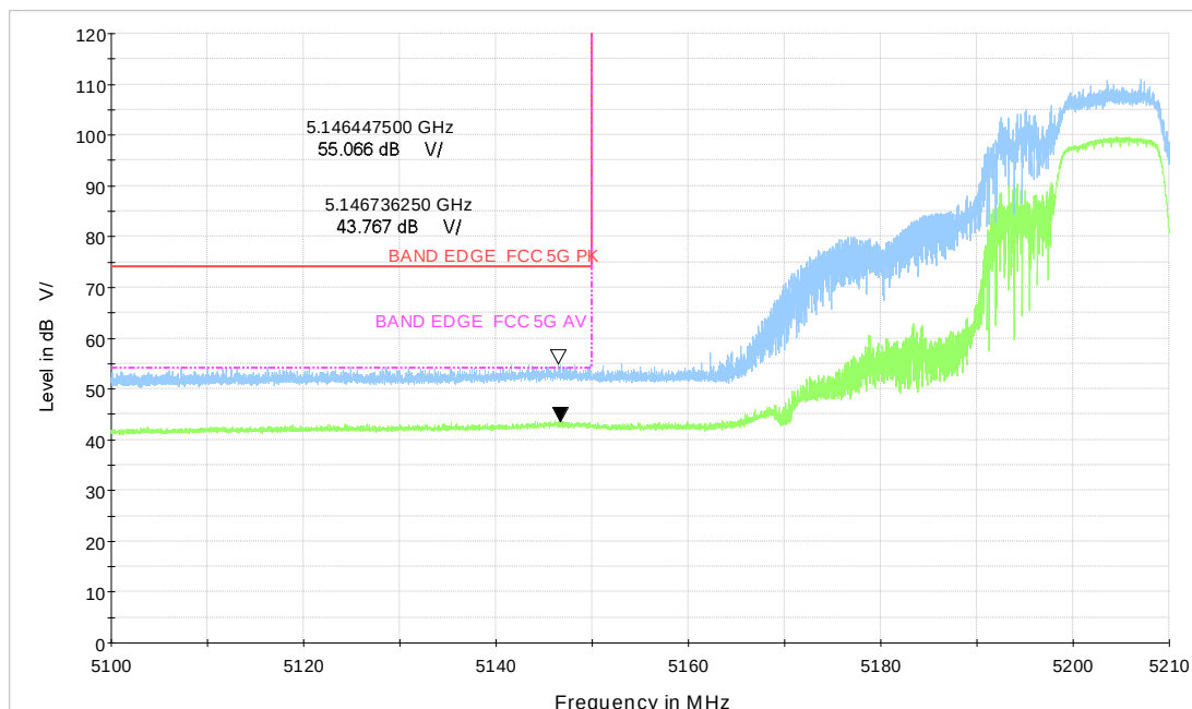
Wi-Fi 5GHz_BE40 106+26Tone HIGH_CH38
