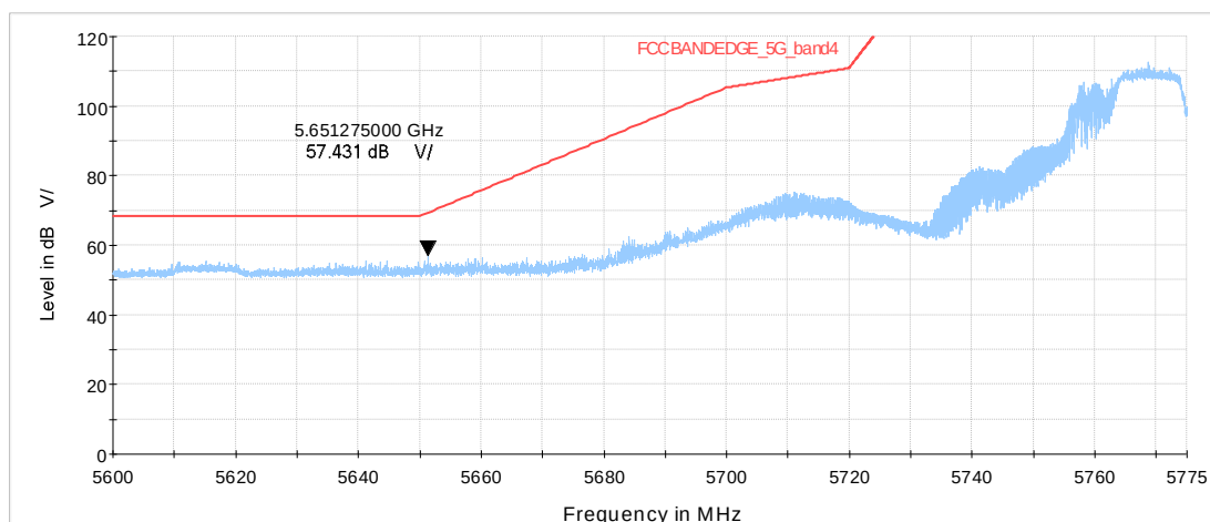
Wi-Fi 5GHz_BE40 106+26Tone HIGH_CH151
