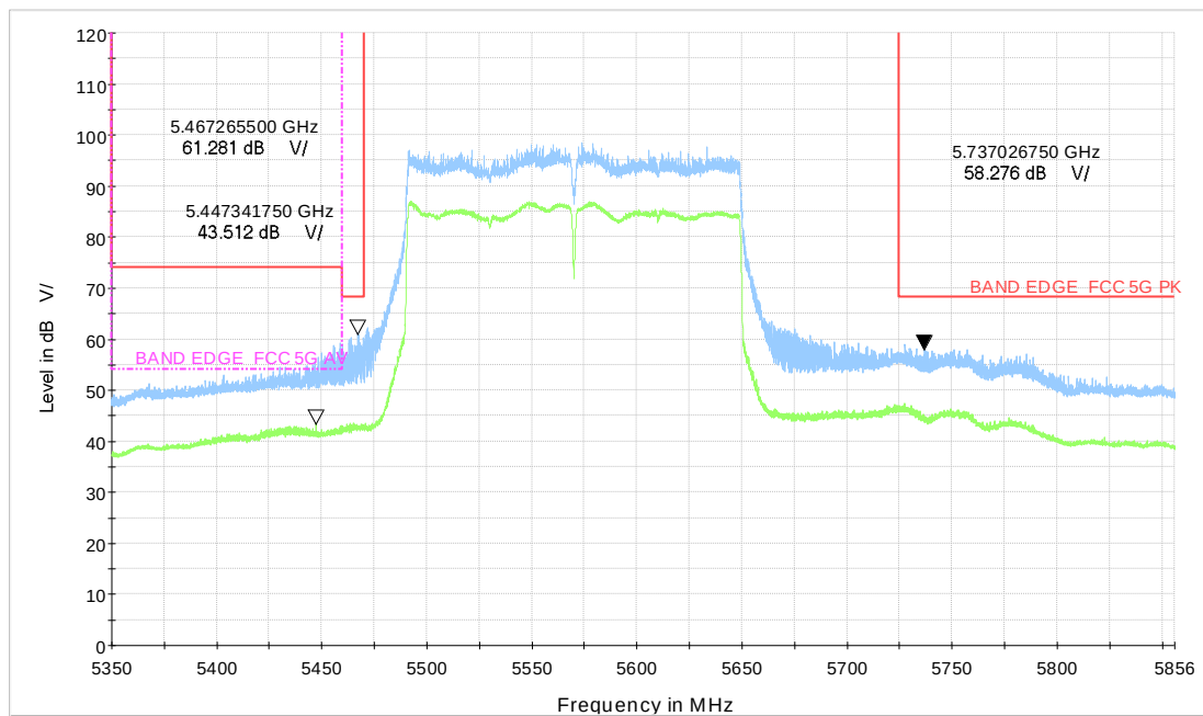
Wi-Fi 5GHz_ax160 CH114
