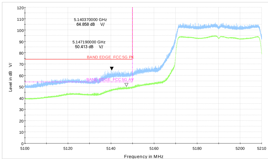
Wi-Fi 5GHz_BE40 CH38
