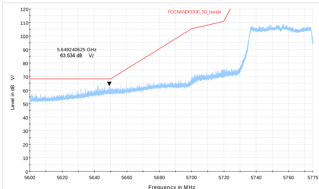
Wi-Fi 5GHz_ax40 CH151
