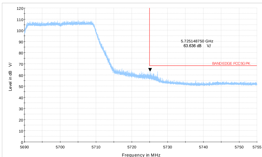
Wi-Fi 5GHz_ax20 CH140
