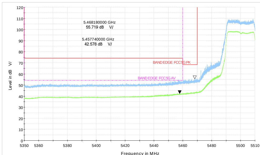
Wi-Fi 5GHz_ax20 CH100
