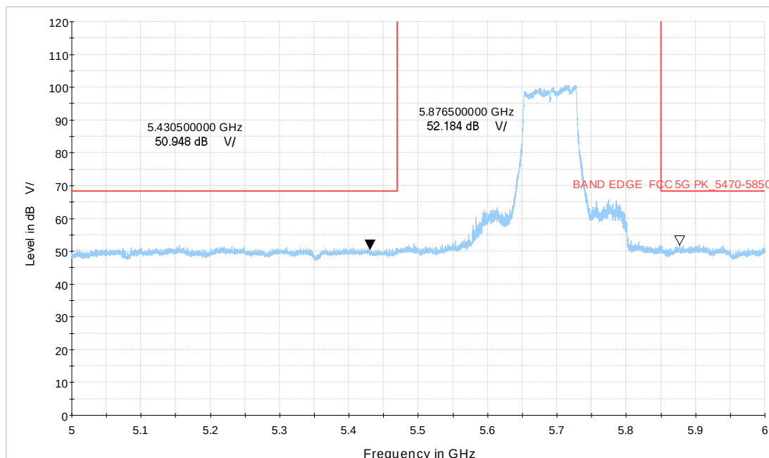
Wi-Fi 5GHz_ac80 CH138
