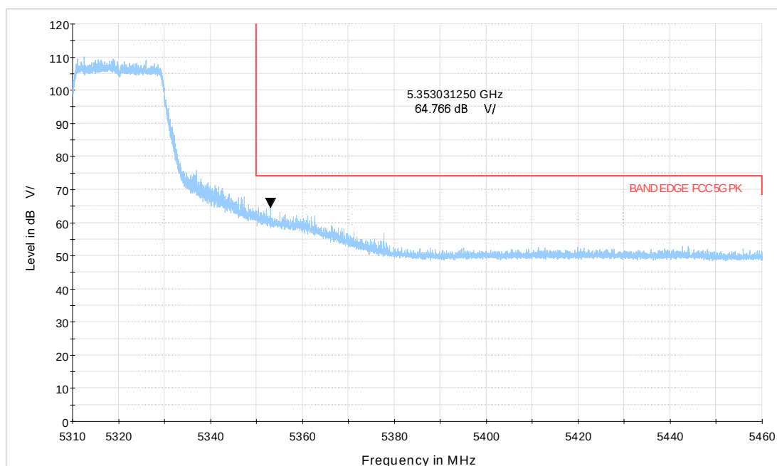
Wi-Fi 5GHz_BE20 CH64
