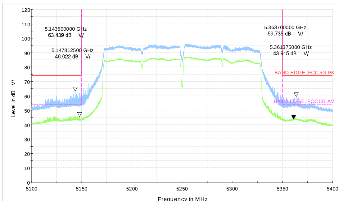
Wi-Fi 5GHz_ac160 CH50
