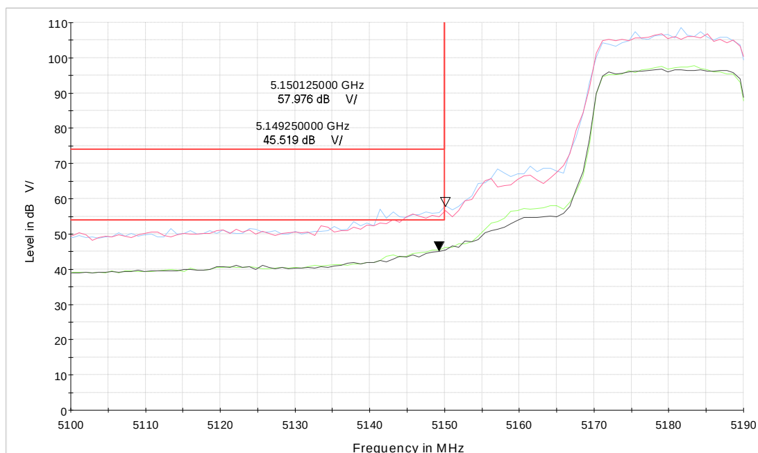
Wi-Fi 5GHz TB_ax20 CH36_242Tone
