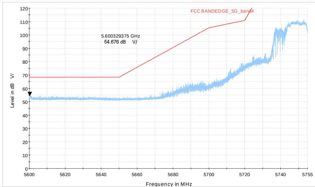
Wi-Fi 5GHz_BE20 106+26Tone HIGH_CH149
