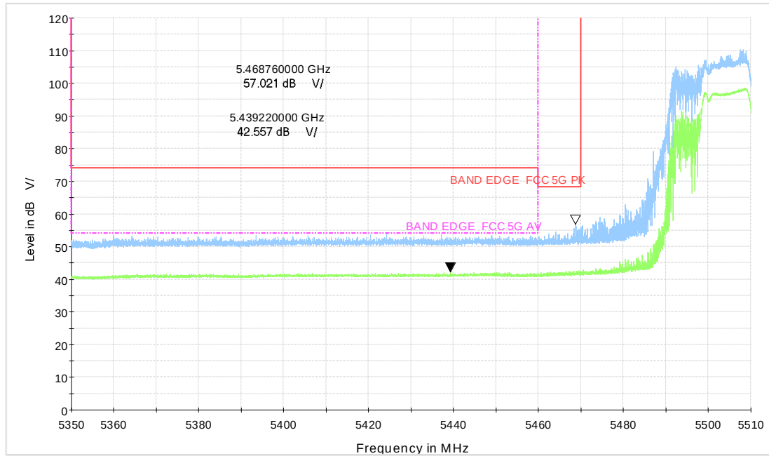
Wi-Fi 5GHz_BE20 106+26Tone HIGH_CH100
