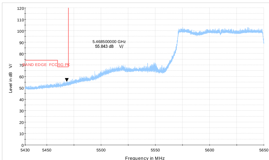
Wi-Fi 5GHz_BE80 CH122
