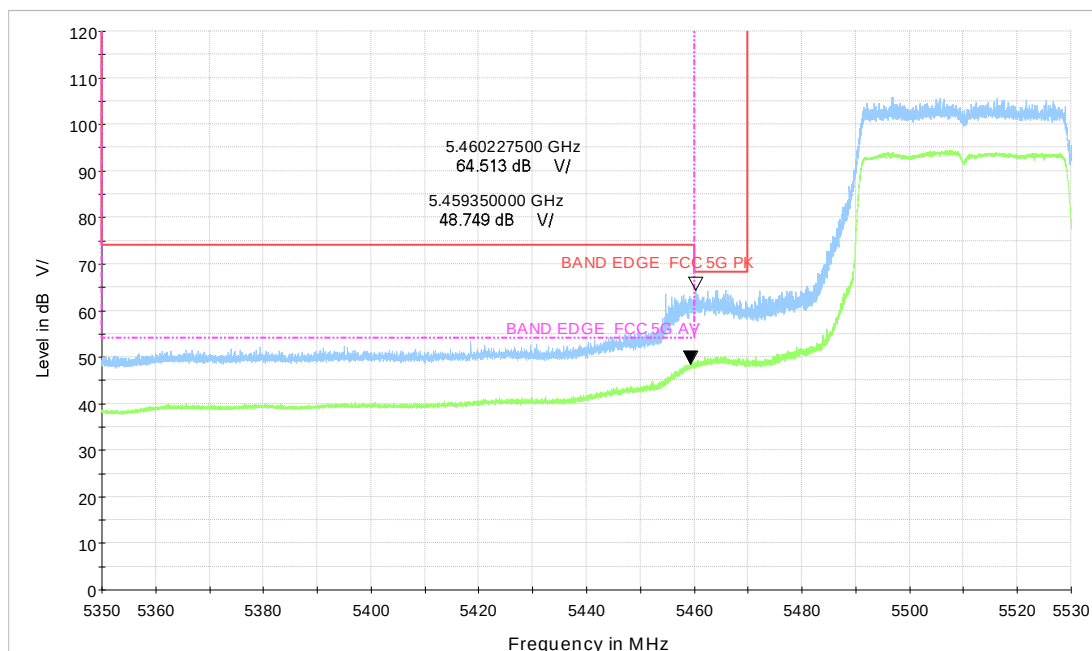
Wi-Fi 5GHz TB_ax40 CH102_484Tone
