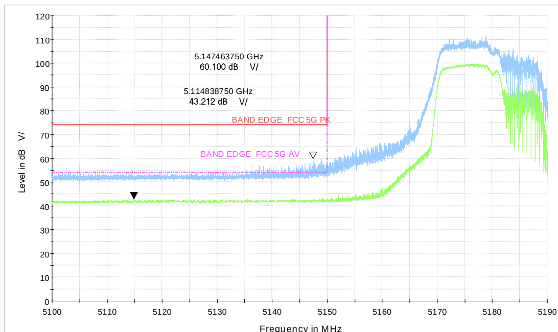
Wi-Fi 5GHz_BE20 106+26Tone LOW_CH36
