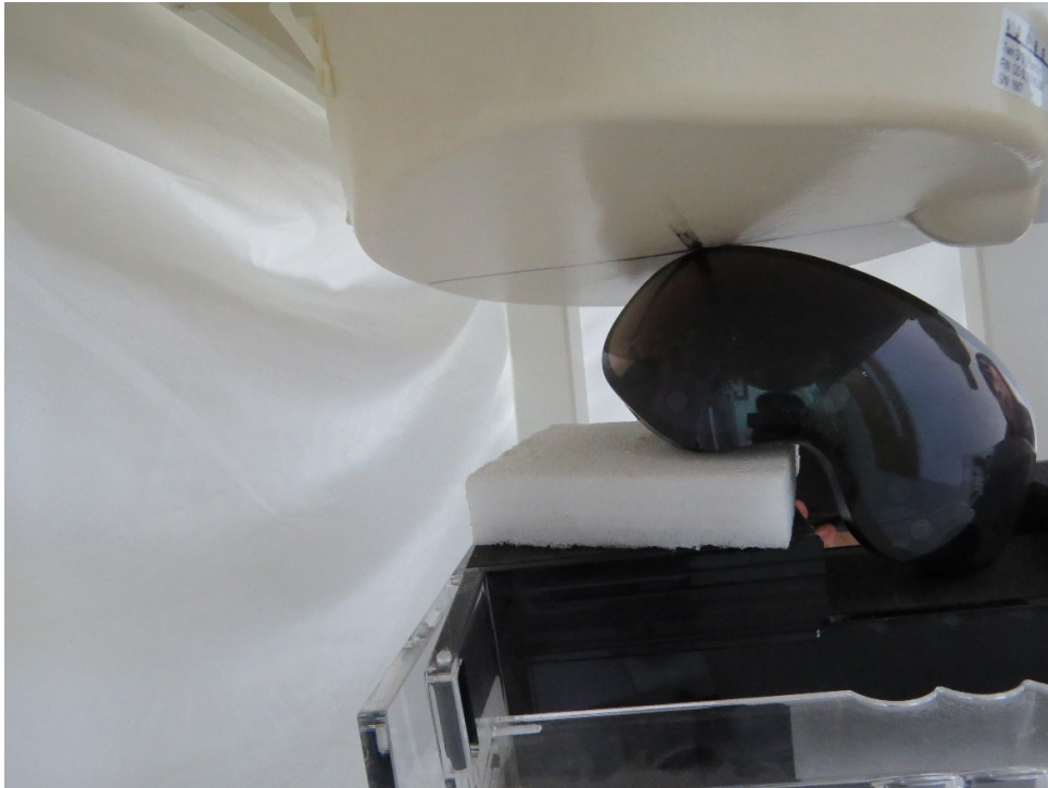
Picture 6: Top Edge1- TS6, the distance from EUT to the bottom of the Phantom is 0mm
