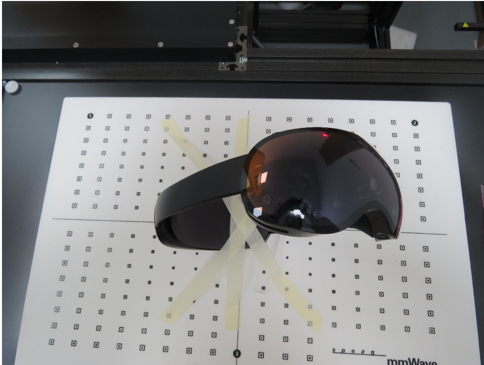
Picture 11: Front Side1-TS8, the distance from EUT to the Probe is 2mm or \lambda/5 mm
