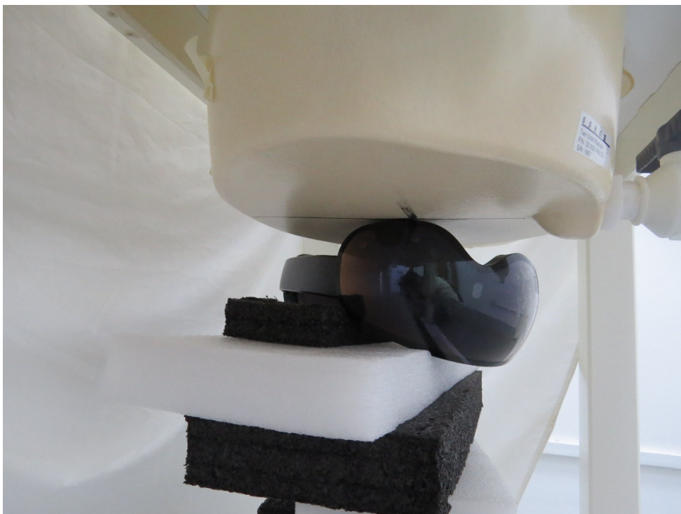
Picture 9: Bottom Edge2- TS2, the distance from EUT to the bottom of the Phantom is 0mm
