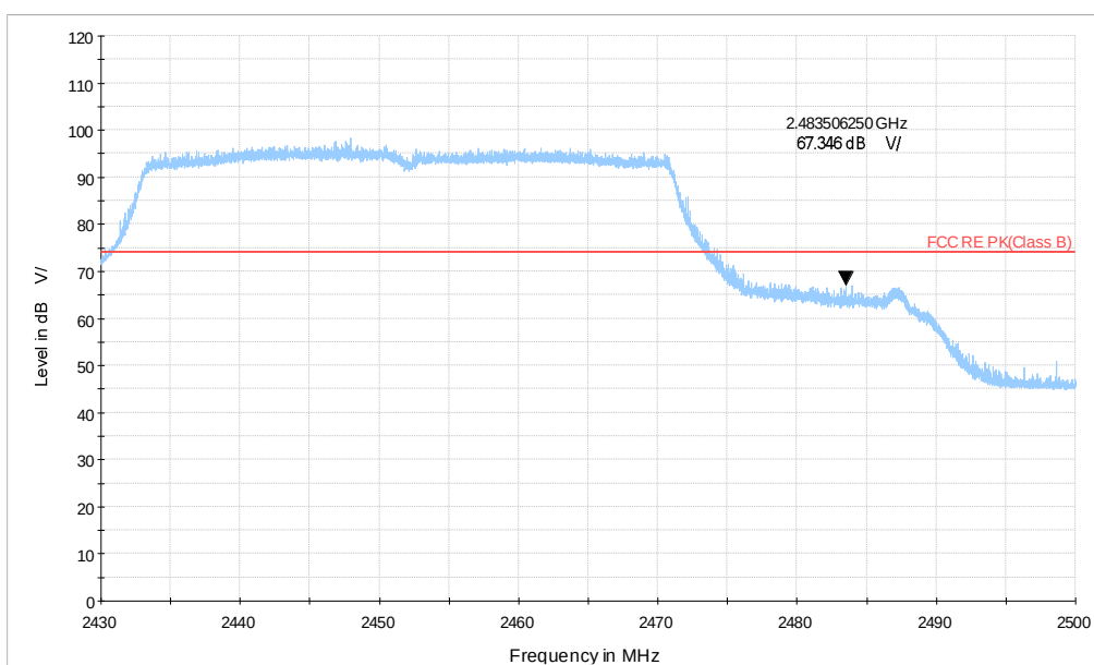
Wi-Fi 2.4G_BE40 CH9_2.43-2.5GHz_MCS13_MIMO_PK
