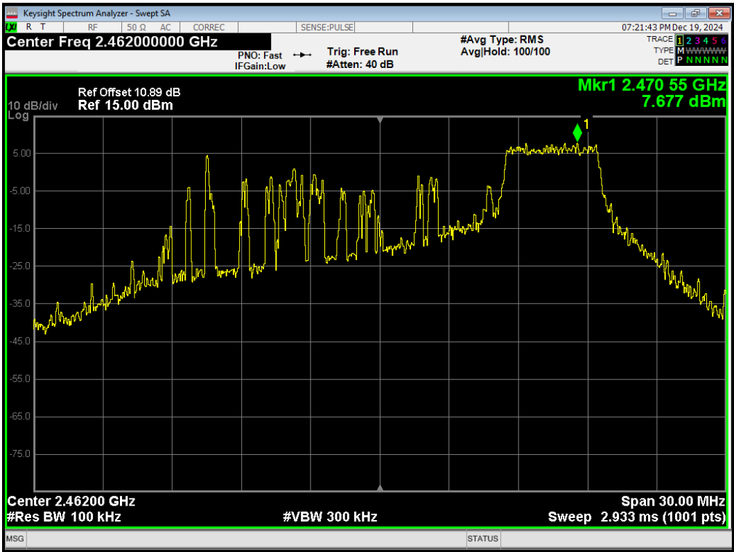
Tx. Spurious 802.11be(20) 52-Tones Index40 2462MHz Emission
