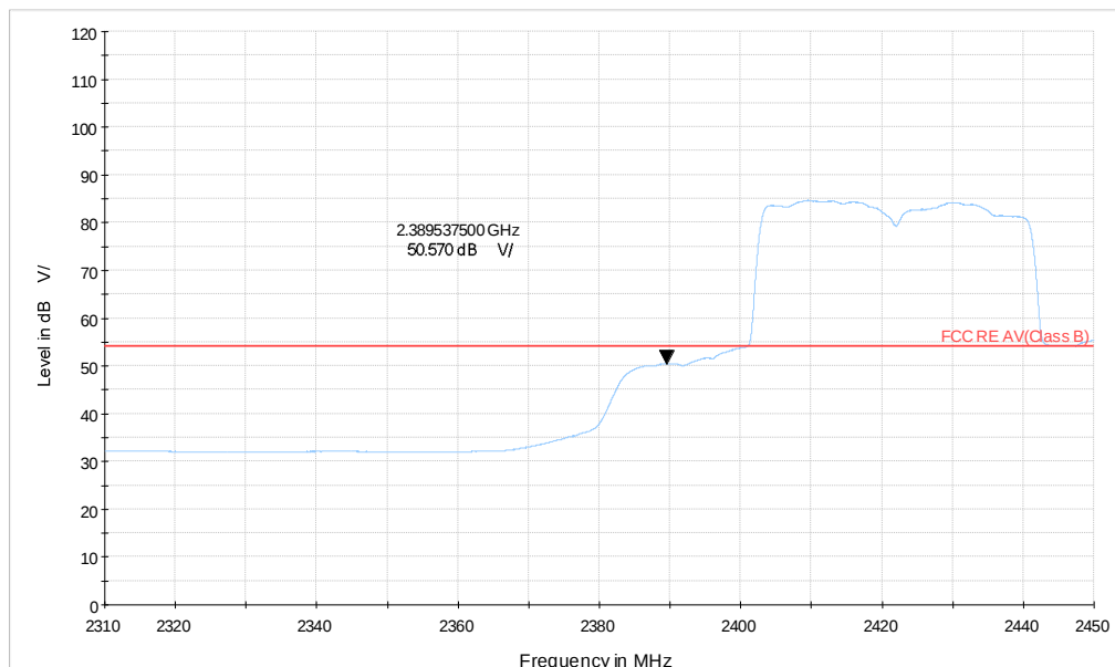
Wi-Fi 2.4G_ax40 CH3_2.31-2.45GHz_MCS13_MIMO_AV
