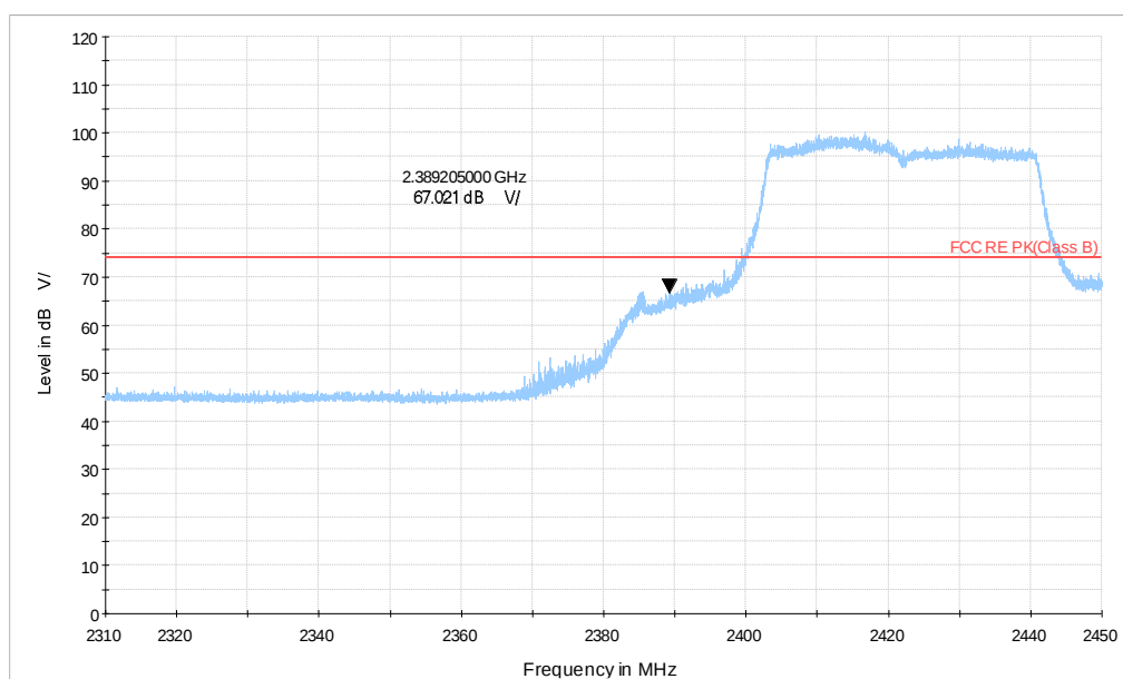
Wi-Fi 2.4G_ax40 CH3_2.31-2.45GHz_MCS13_MIMO_PK
