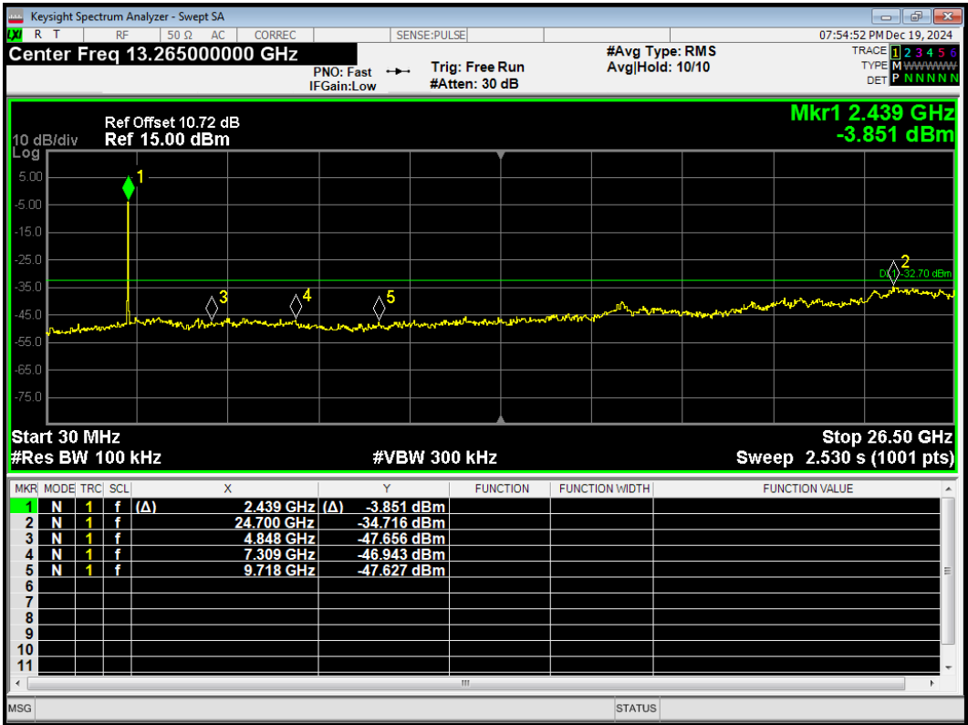
Tx. Spurious 802.11be(20) 106-Tones Index53 2437MHz Ref
