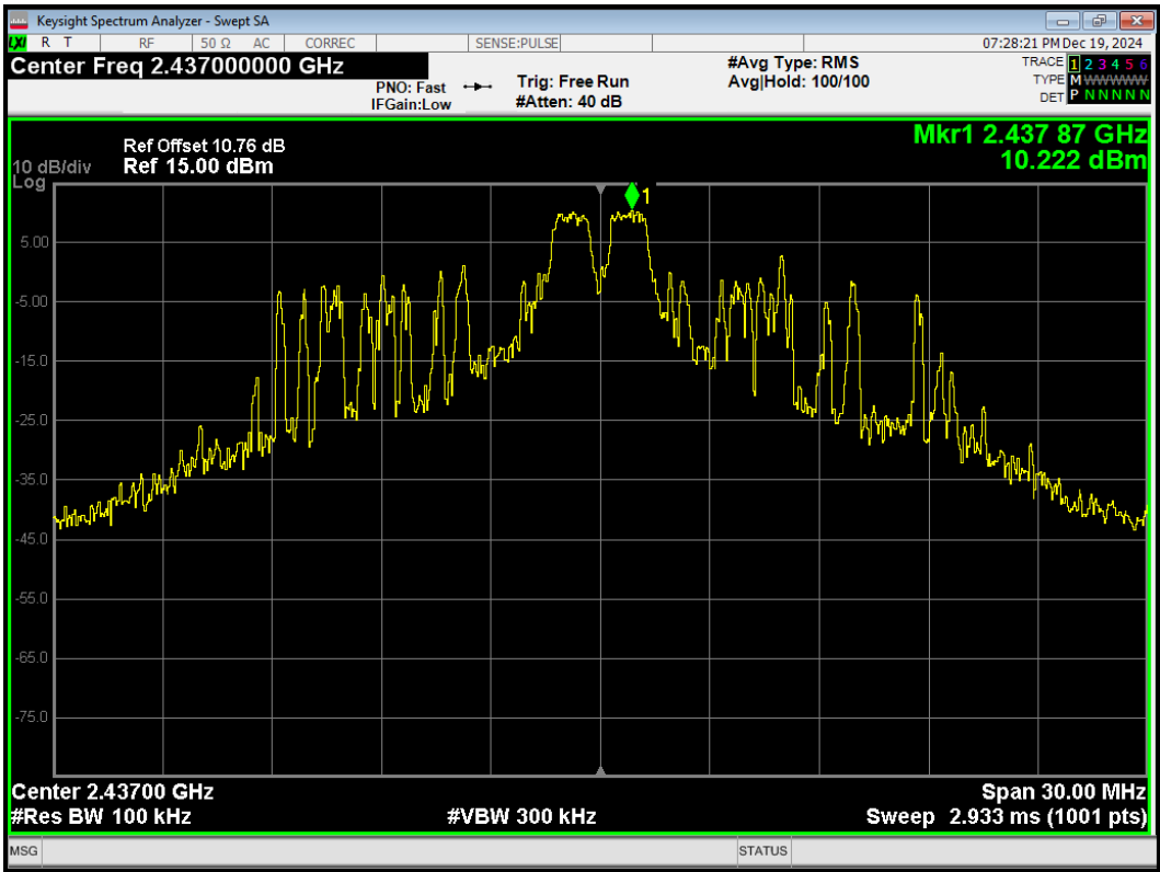
Tx. Spurious 802.11ax(HE20) 26-Tones Index4 2437MHz Emission
