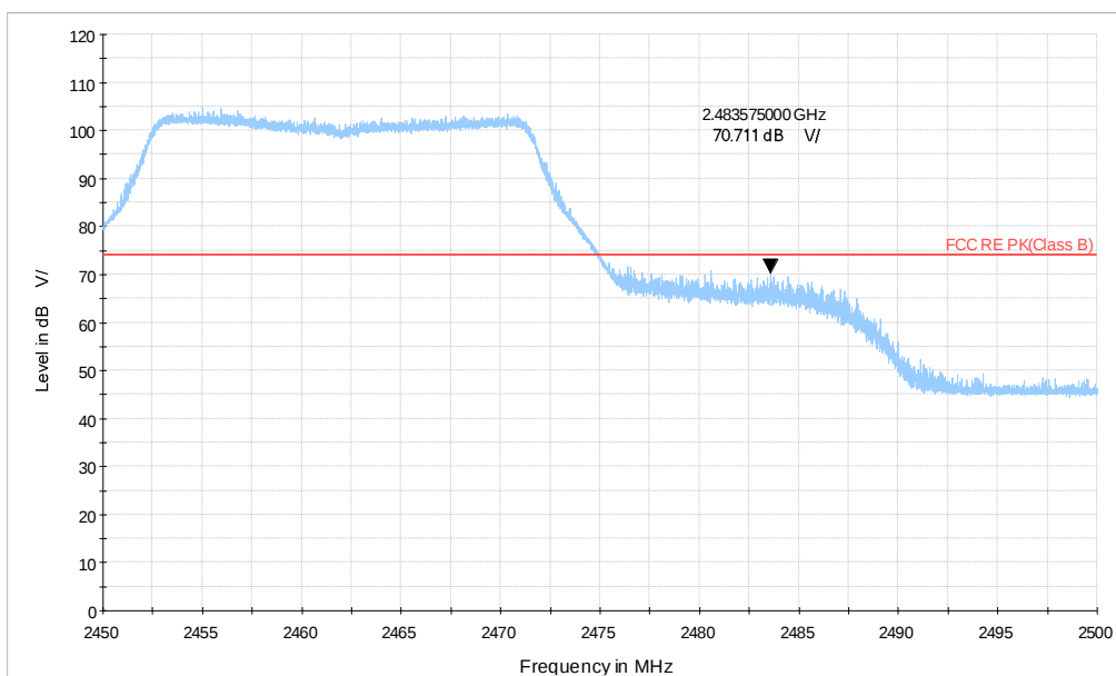
Wi-Fi 2.4G_BE20 CH11_2.45-2.5GHz_MCS13_MIMO_PK
