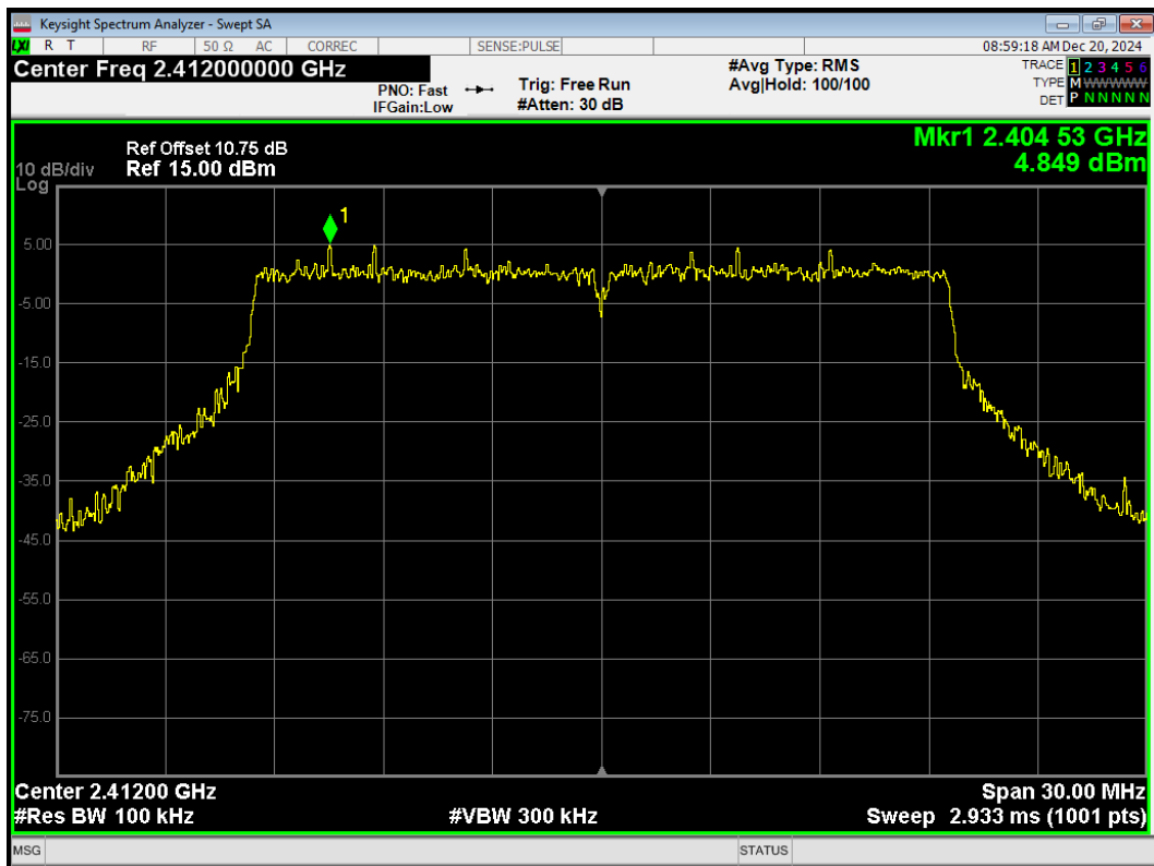
Tx. Spurious 802.11be(20) 242-Tones Index61 2412MHz Emission
