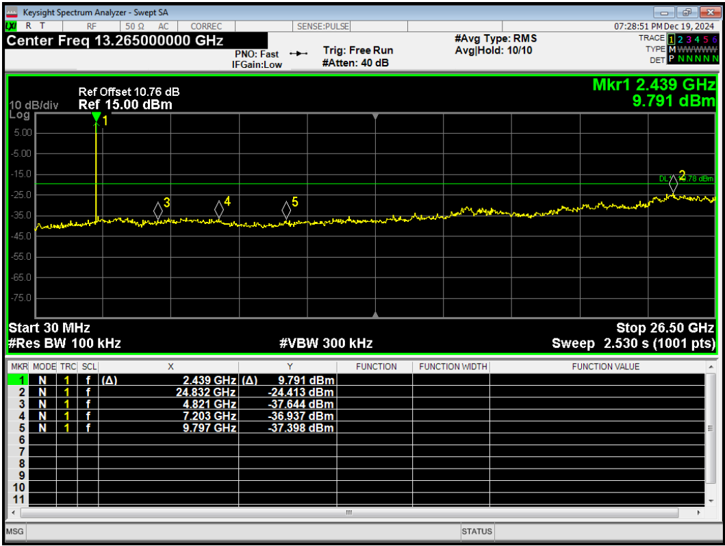
Tx. Spurious 802.11ax(HE40) 26-Tones Index0 2422MHz Ref
