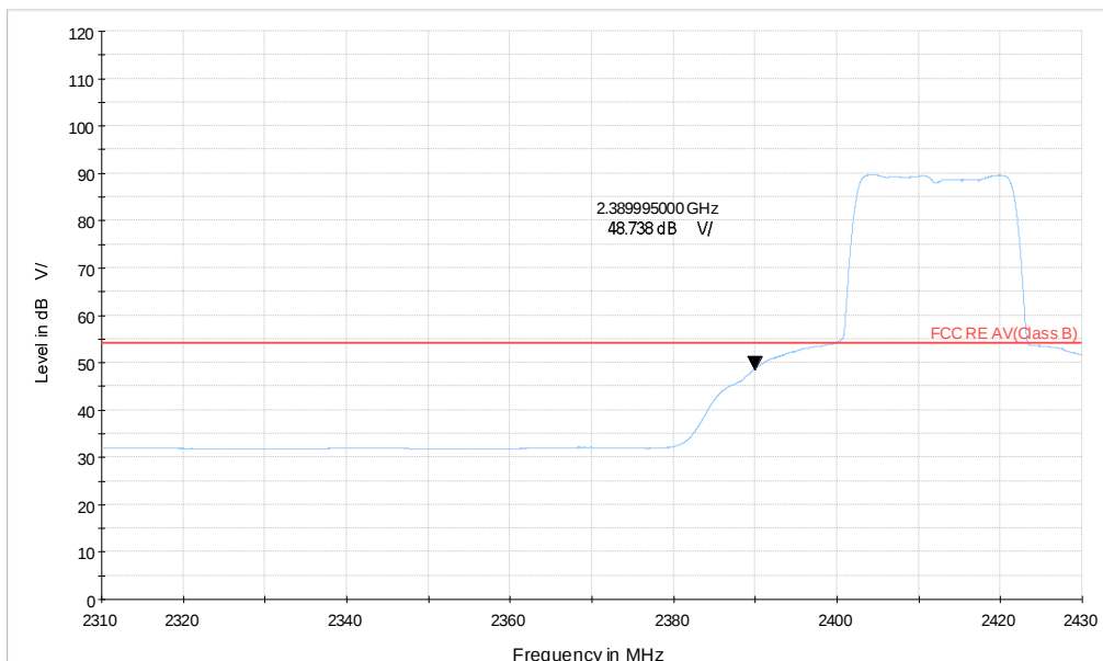
Wi-Fi 2.4G_BE20 CH1_2.31-2.43GHz_MCS13_MIMO_AV
