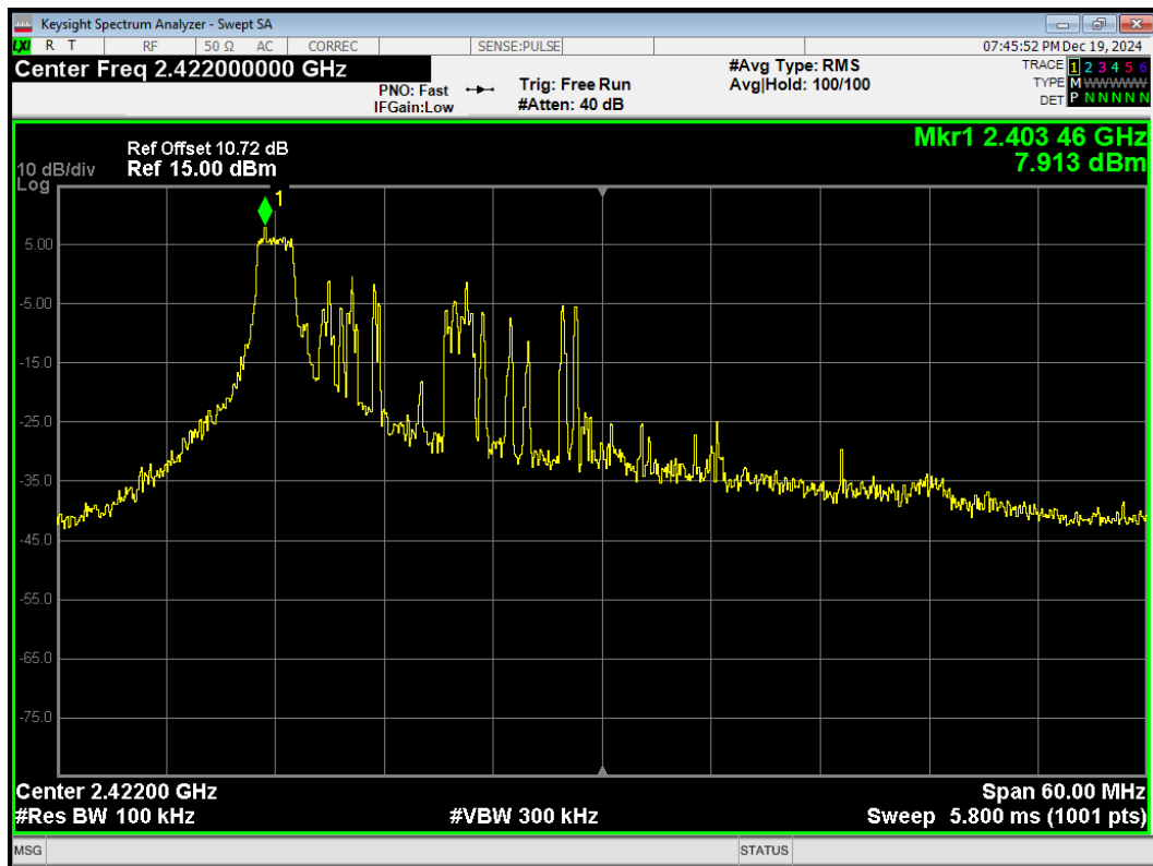
Tx. Spurious 802.11ax(HE40) 26-Tones Index0 2422MHz Emission
