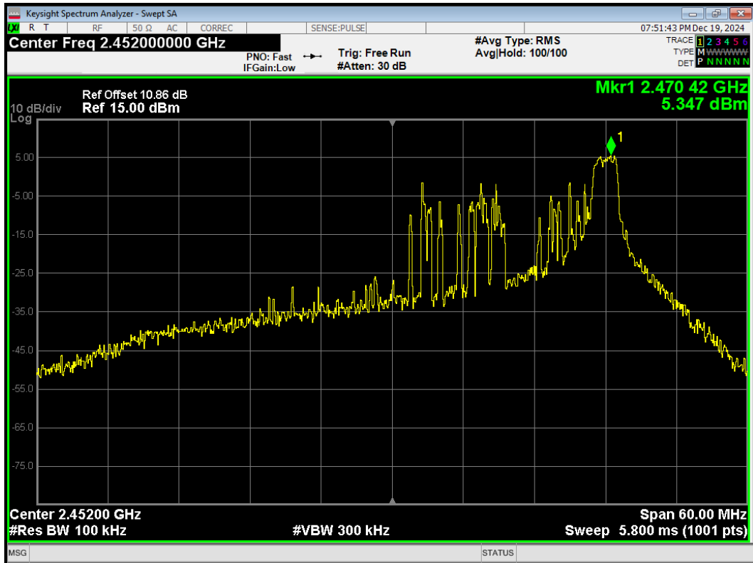
Tx. Spurious 802.11ax(HE40) 26-Tones Index17 2452MHz Emission
