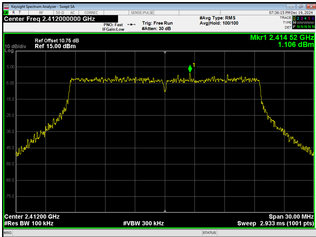
Tx. Spurious 802.11ax(HE20) 242-Tones Index61 2412MHz Emission
