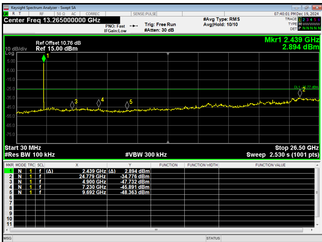
Tx. Spurious 802.11ax(HE20) 242-Tones Index61 2462MHz Ref
