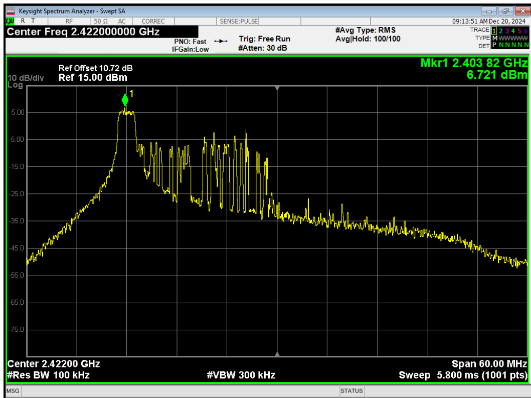
Tx. Spurious 802.11be(40) 26-Tones Index0 2422MHz Emission
