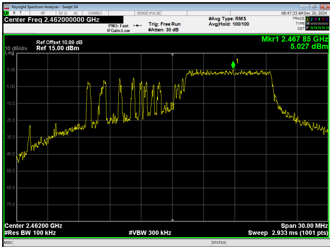
Tx. Spurious 802.11be(20) 106-Tones Index54 2462MHz Emission
