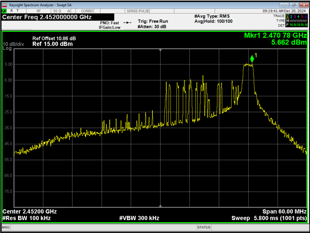
Tx. Spurious 802.11be(40) 26-Tones Index17 2452MHz Emission
