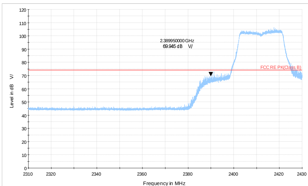
Wi-Fi 2.4G_BE20 CH1_2.31-2.43GHz_MCS13_MIMO_PK
