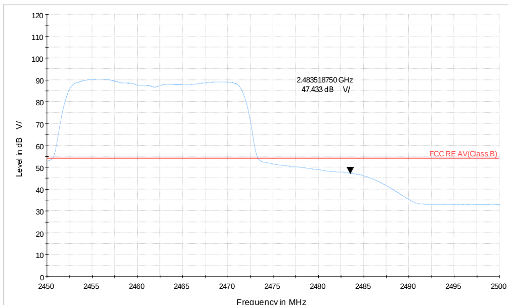
Wi-Fi 2.4G_BE20 CH11_2.45-2.5GHz_MCS13_MIMO_AV
