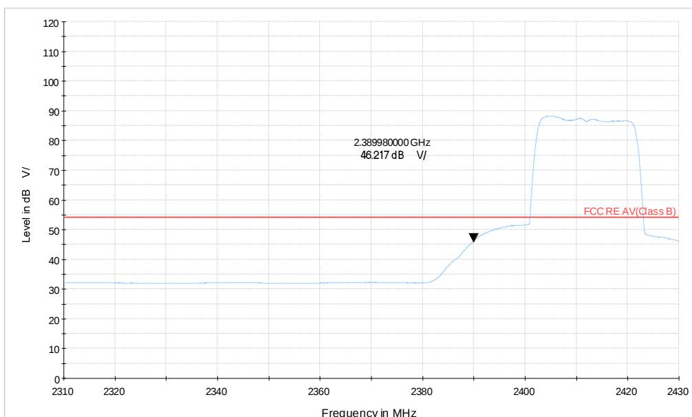
Wi-Fi 2.4G_ax20 CH1_2.31-2.43GHz_MCS13_MIMO_AV
