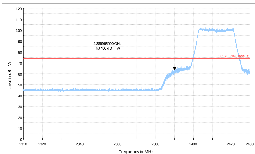
Wi-Fi 2.4G_ax20 CH1_2.31-2.43GHz_MCS13_MIMO_PK
