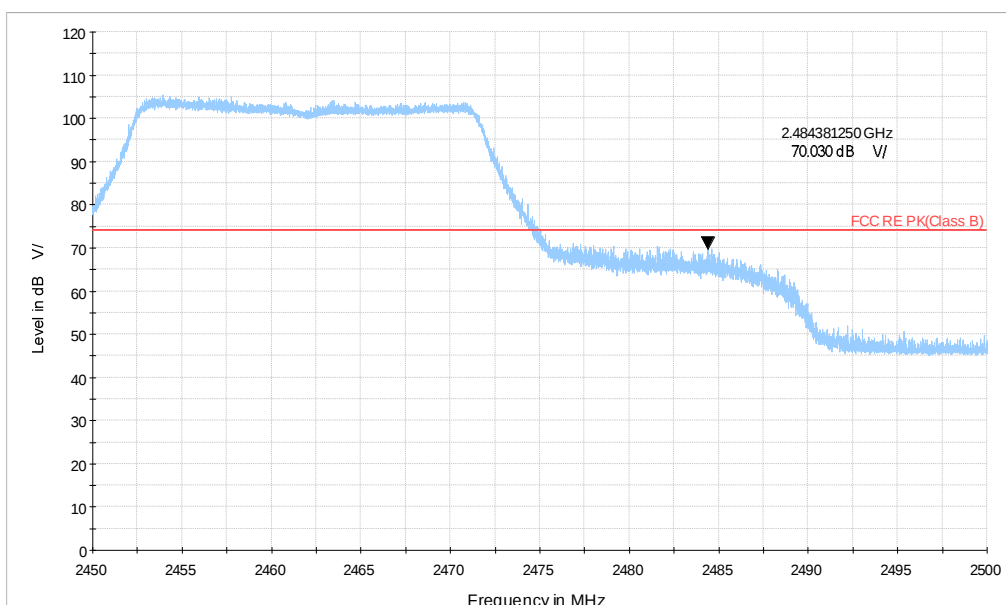
Wi-Fi 2.4G_ax20 CH11_2.45-2.5GHz_MCS13_MIMO_PK
