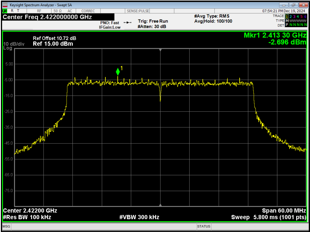
Tx. Spurious 802.11ax(HE40) 484-Tones Index65 2422MHz Emission
