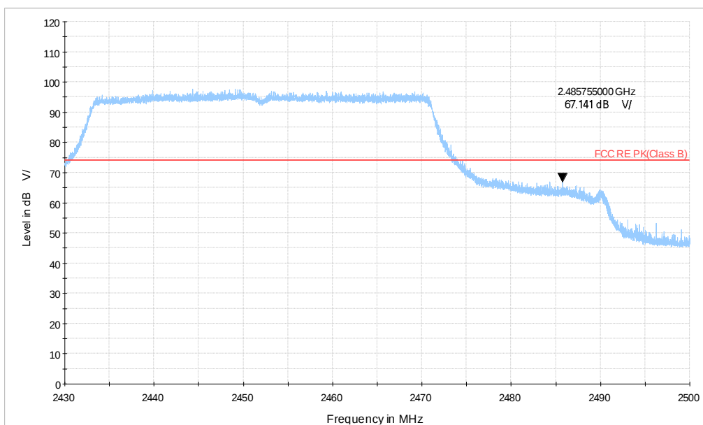
Wi-Fi 2.4G_ax40 CH9_2.43-2.5GHz_MCS13_MIMO_PK
