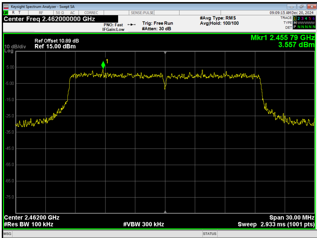
Tx. Spurious 802.11be(20) 242-Tones Index61 2462MHz Emission
