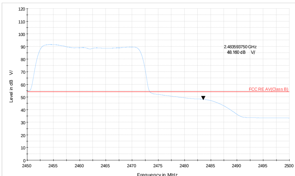
Wi-Fi 2.4G_ax20 CH11_2.45-2.5GHz_MCS13_MIMO_AV
