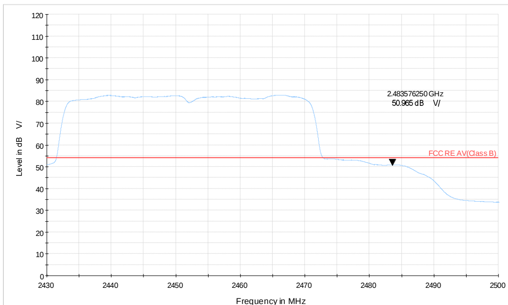
Wi-Fi 2.4G_ax40 CH9_2.43-2.5GHz_MCS13_MIMO_AV
