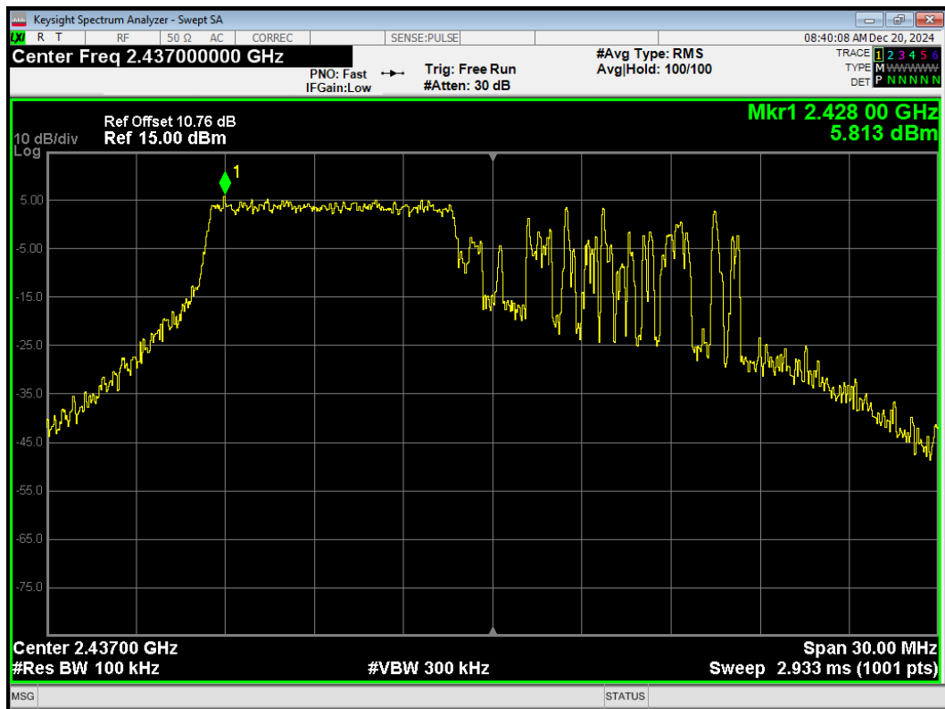
Tx. Spurious 802.11be(20) 106-Tones Index53 2437MHz Emission
