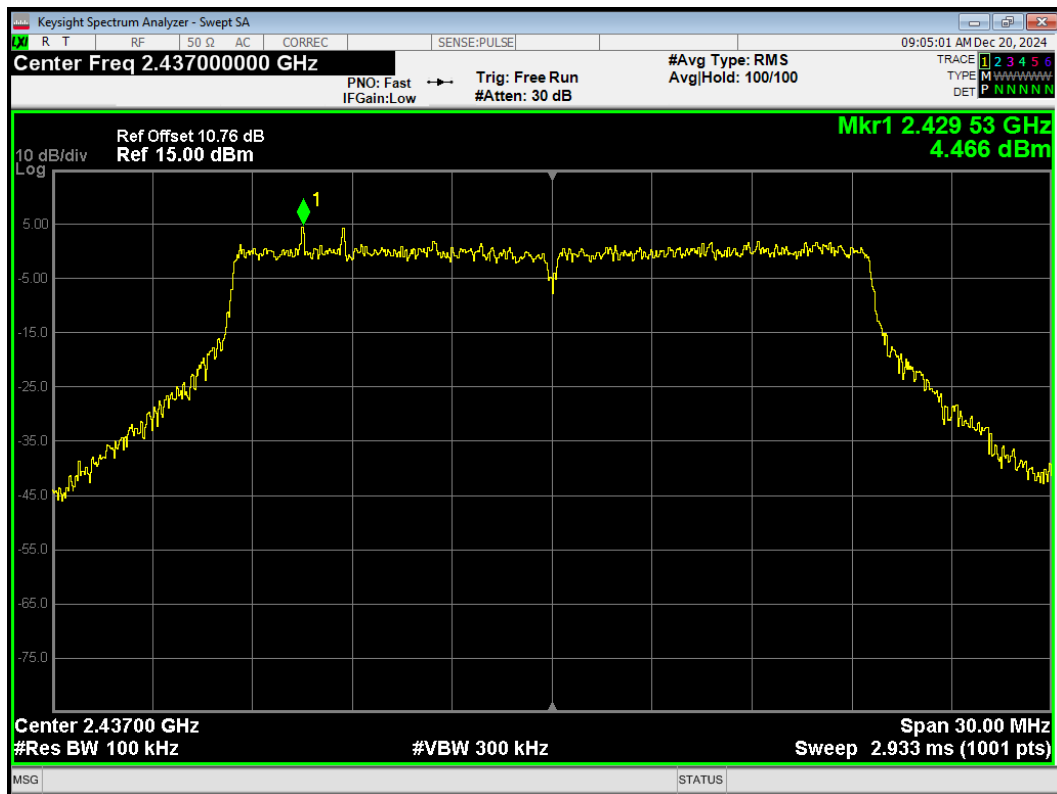
Tx. Spurious 802.11be(20) 242-Tones Index61 2437MHz Emission
