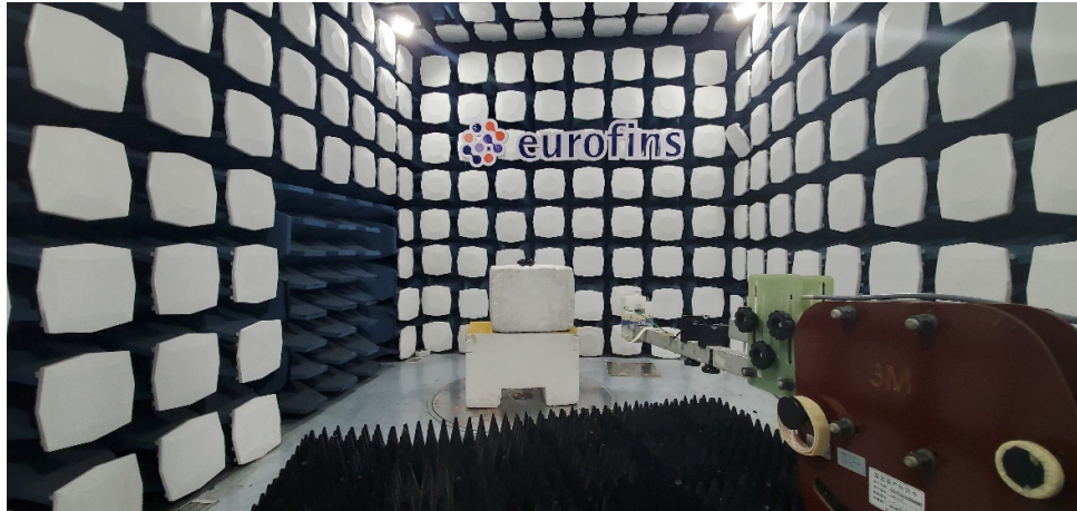
Picture 1 Radiated Emission Test Setup
