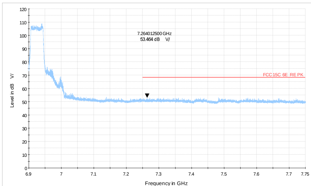
484TONE_802.11ax40 CH195_6.9-7.75GHz_MCS0_MIMO
