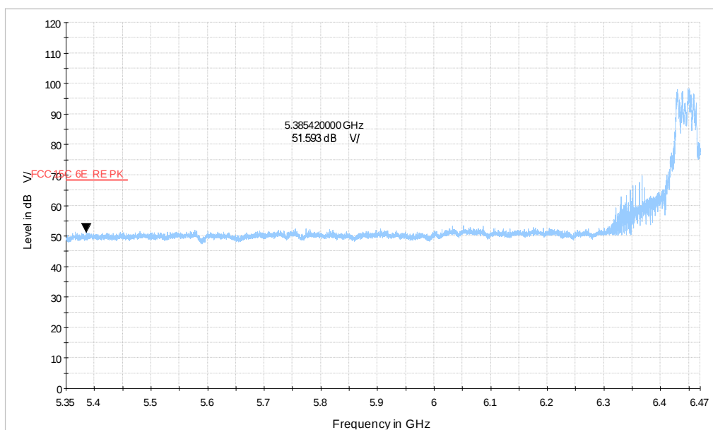
484TONE_802.11be40 CH99_5.35-6.47GHz_MCS0_MIMO
