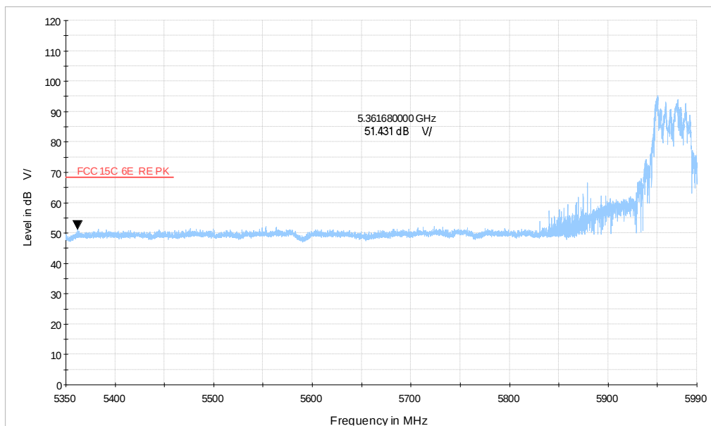
484TONE_802.11be40 CH3_5.35-5.99GHz_MCS0_MIMO
