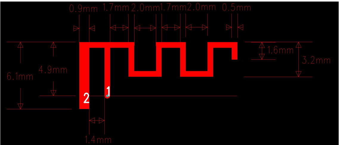
Antenna Dimensions
