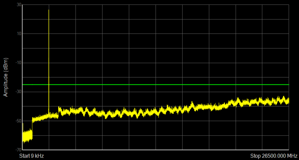
Band41 16QAM BW=10MHz Channel=41140 RB Size=1 Position=#0
