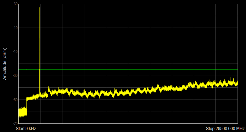
Band41 16QAM BW=10MHz Channel=40640 RB Size=1 Position=#0
