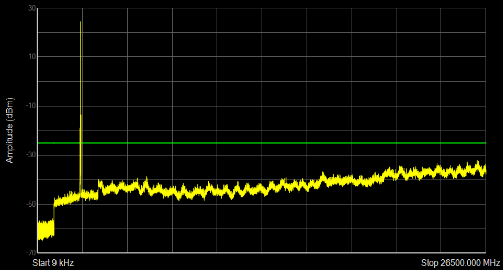
Band41 QPSK BW=20MHz Channel=40190 RB Size=1 Position=#0
