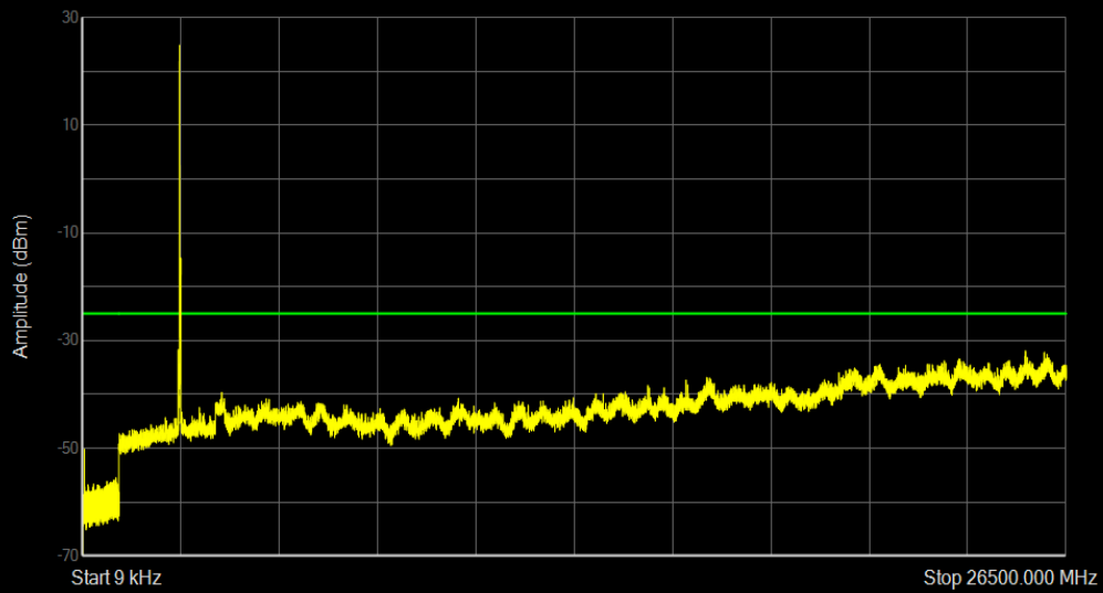
Band41 QPSK BW=20MHz Channel=41090 RB Size=1 Position=#0
