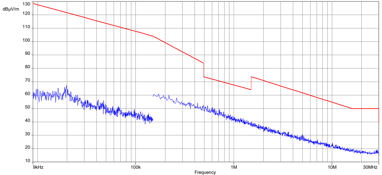
Plot 1: 9 kHz to 30 MHz FCC
