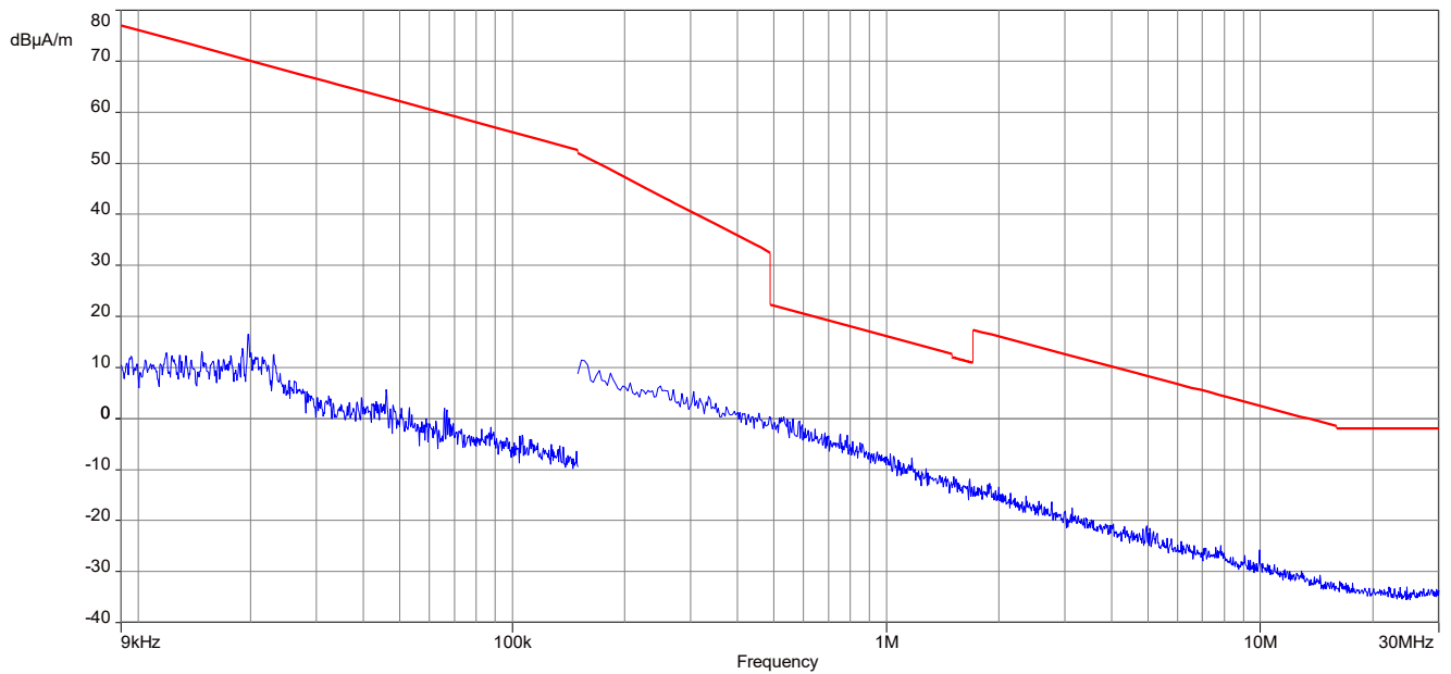
Plot 2: 9 kHz to 30 MHz IC
