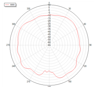
Phi=90 freq=5850MHz
