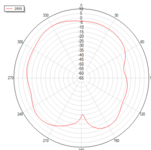
Phi=90 freq=2500MHz
