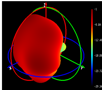
Phi=0 freq=2500MHz
