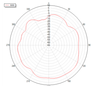
Theta=90 freq=5850MHz
