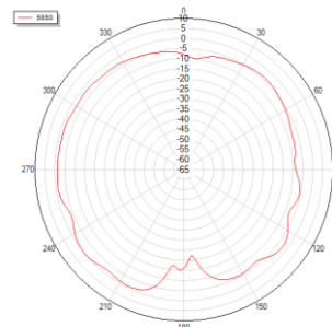
Phi=0 freq=5850MHz
