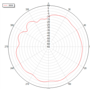
Theta=90 freq=5500MHz
