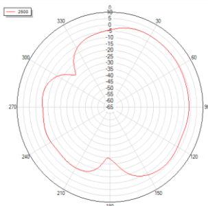
Phi=0 freq=2500MHz
