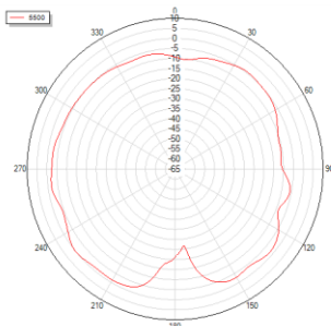
Phi=0 freq=5500MHz
