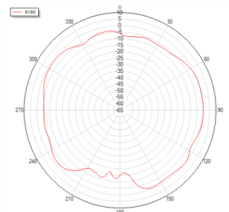
Phi=90 freq=5150MHz
