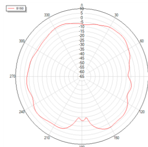
Phi=0 freq=5150MHz
