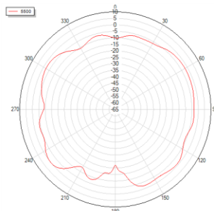
Phi=90 freq=5500MHz
