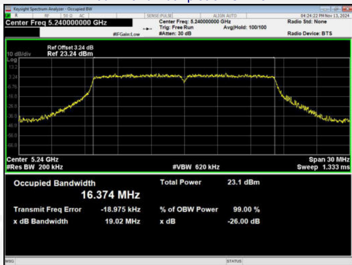
26dB Bandwidth plot on CH 48
