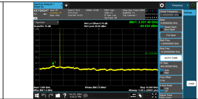
Band41(2555-2655)-15MHz-QPSK-40215-1RB#0-20000-27000-PASS
