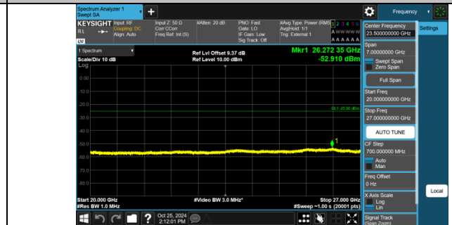
Band41(2555-2655)-10MHz-QPSK-40190-1RB#0-1000-10000-PASS
