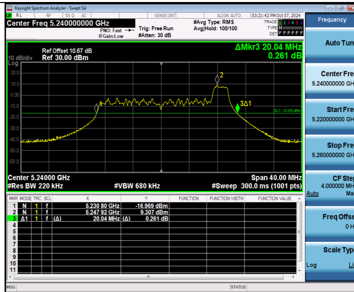
11AX20MIMO Ant W0 5240 52Tone RU40
