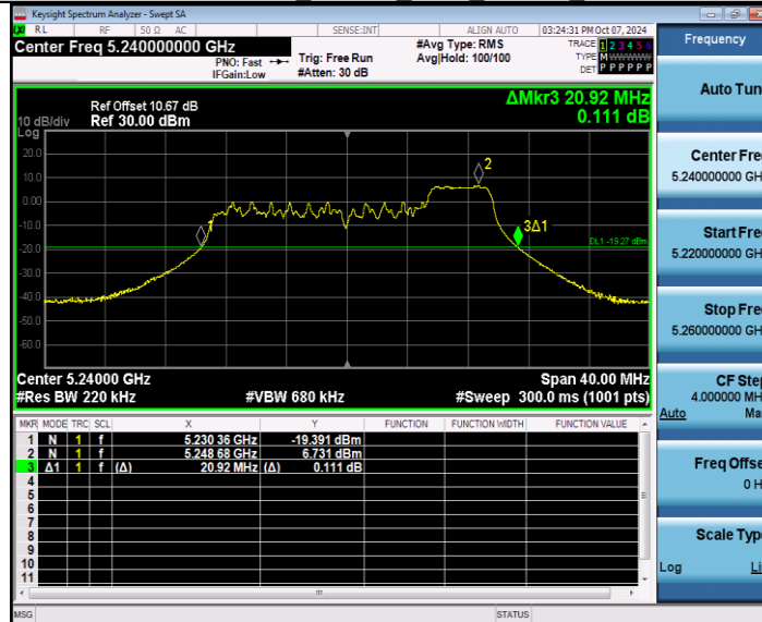
11AX20MIMO Ant W0 5240 106Tone RU54
