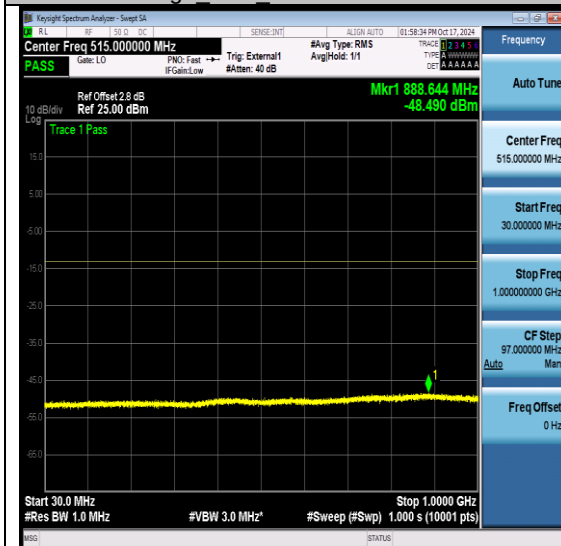
NTNV-N77-3700-3980-PC3-30-60-H-DFT-QPSK-Edge_1RB_Left-Ant1-PASS
