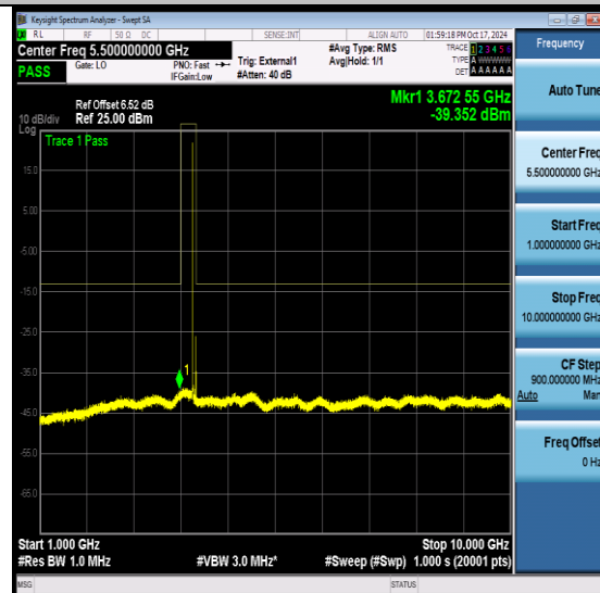
NTNV-N77-3700-3980-PC3-30-60-H-DFT-QPSK-Edge_1RB_Left-Ant1-PASS
