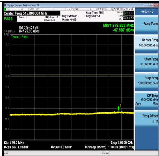
NTNV-N77-3700-3980-PC3-30-10-M-DFT-Q PSK-Edge_1RB Left-Ant1-PASS
