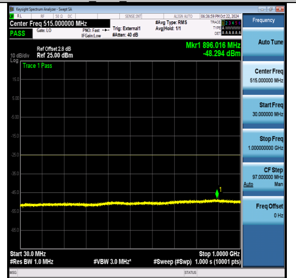
NTNV-N41-2545-2655-PC3-30-60-M-DFT-QPSK-Edge_1RB Left-Ant1-PASS
