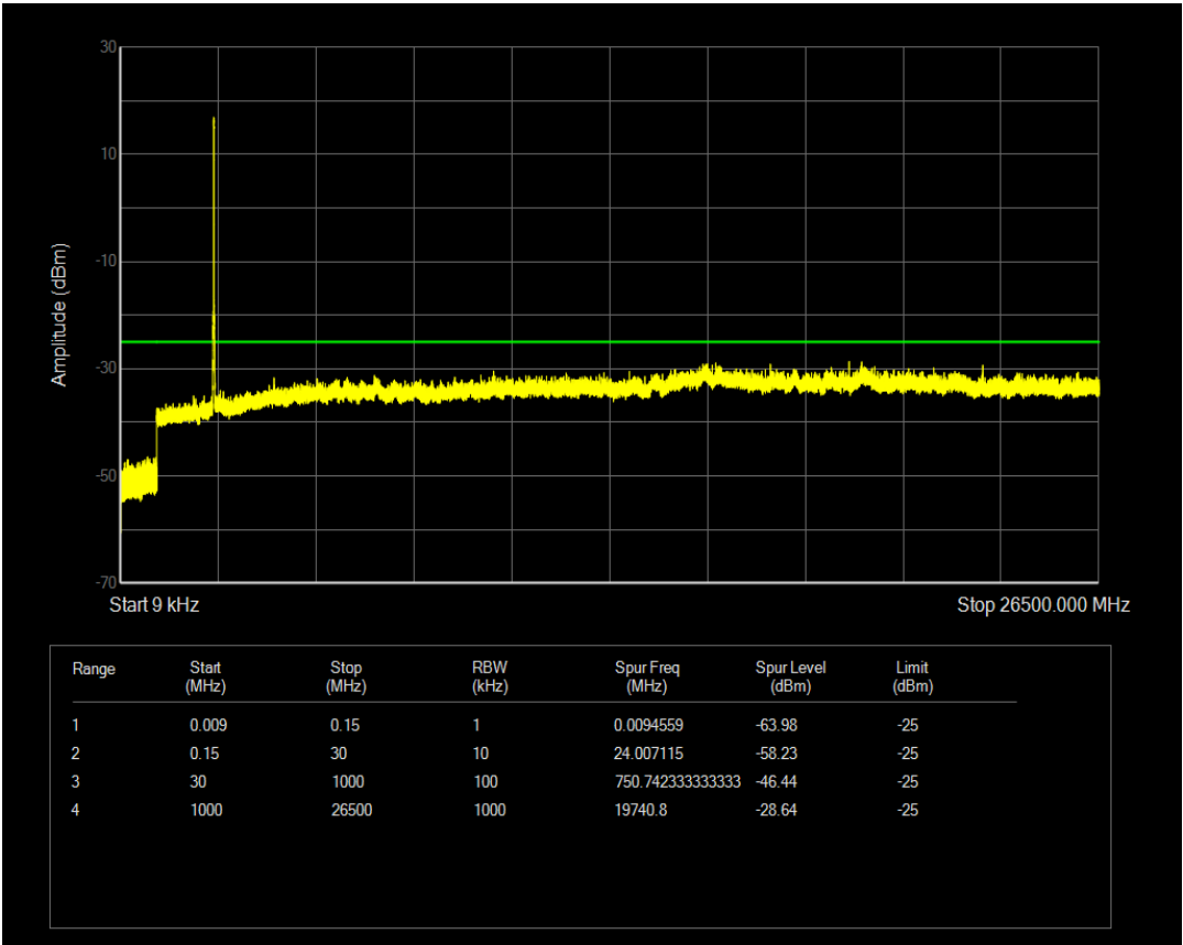
Band41(2535-2675) QPSK BW=15MHz Channel=40740 RB Size=75 Position=#0
