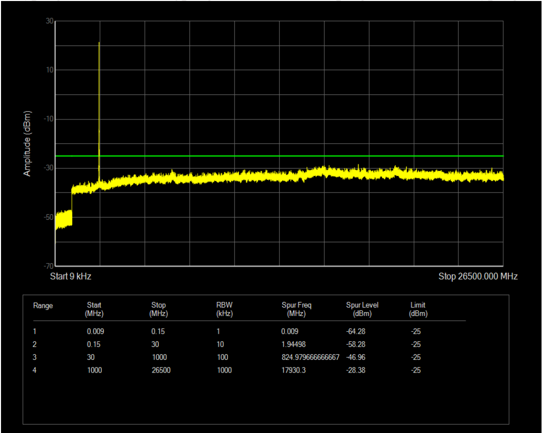
Band41(2535-2675) QPSK BW=5MHz Channel=40740 RB Size=25 Position=#0
