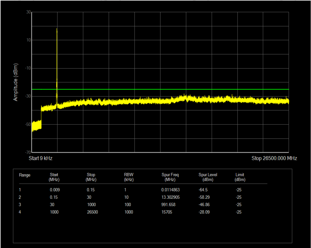
Band41(2535-2675) QPSK BW=20MHz Channel=40740 RB Size=100 Position=#0
