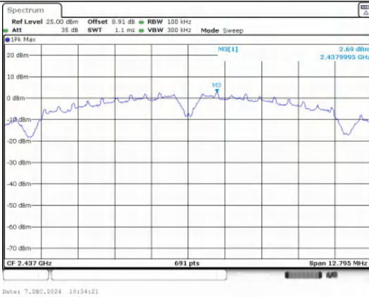
In-Band Reference Level IEEE 802.11b_Channel 6_20MHz_Antenna 1
