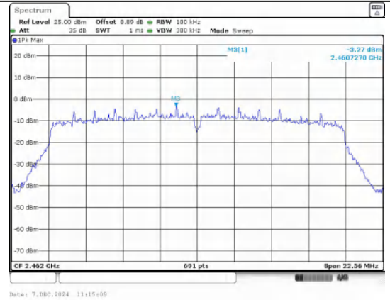
In-Band Reference Level IEEE 802.11n_Channel 11_20MHz_Antenna 1
