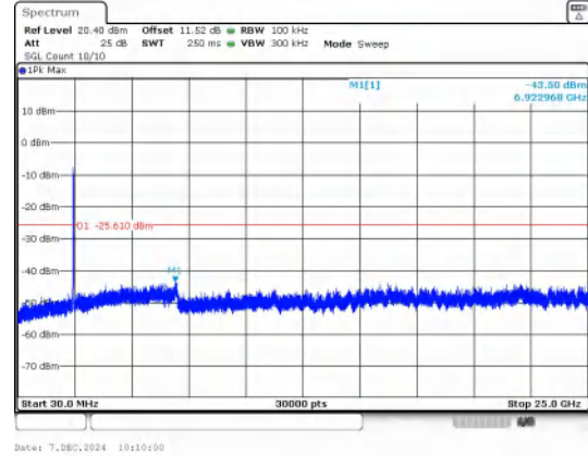
30.0 MHz - 25000.0 MHz IEEE 802.11n_Channel 6_40MHz_Antenna 0
