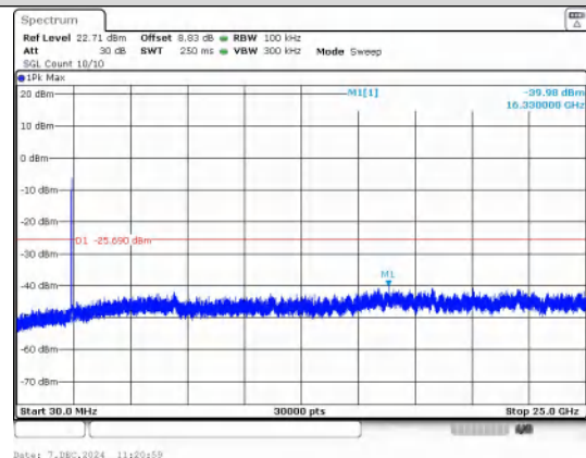
30.0 MHz - 25000.0 MHz IEEE 802.11n_Channel 3_40MHz_Antenna 1
