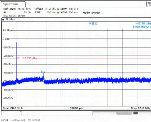
30.0 MHz - 25000.0 MHz IEEE 802.11n_Channel 11_20MHz_Antenna 0
