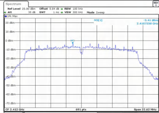
In-Band Reference Level IEEE 802.11g_Channel 1_20MHz_Antenna 1
