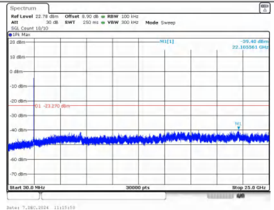
30.0 MHz - 25000.0 MHz IEEE 802.11n_Channel 11_20MHz_Antenna 1
