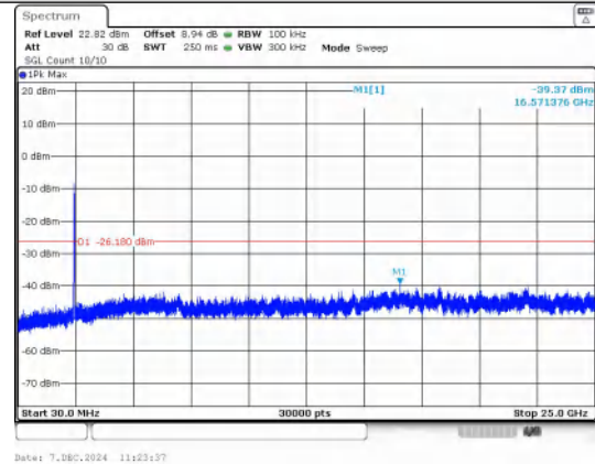
30.0 MHz - 25000.0 MHz IEEE 802.11n_Channel 6_40MHz_Antenna 1
