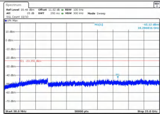
30.0 MHz - 25000.0 MHz IEEE 802.11g_Channel 1_20MHz_Antenna 1
