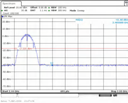
Out Of Band Emission IEEE 802.11b_Channel 11_20MHz_Antenna 1
