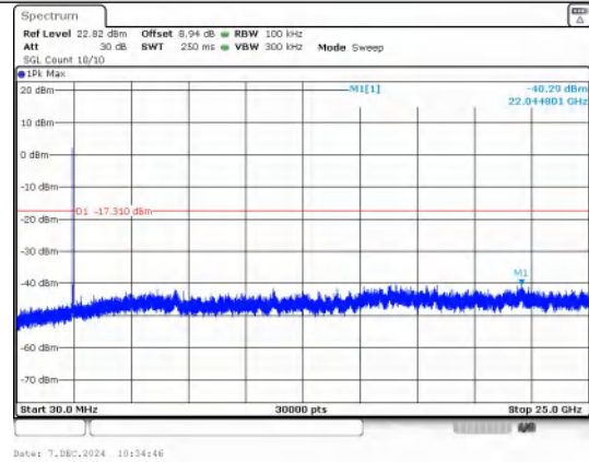
30.0 MHz - 25000.0 MHz IEEE 802.11b_Channel 6_20MHz_Antenna 1
