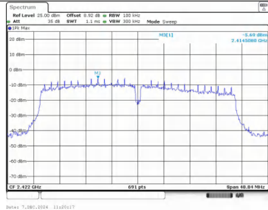
In-Band Reference Level IEEE 802.11n_Channel 3_40MHz_Antenna 1
