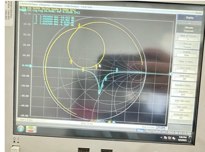
Tigao PCB ANT Matching Result
