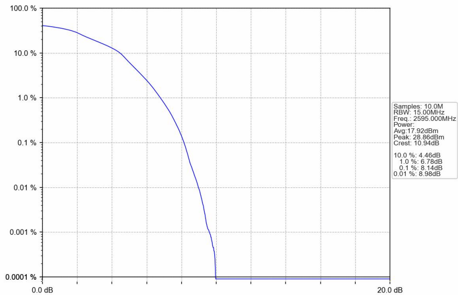
Band38_15MHz_16QAM_MCH_2595MHz_RB_75_0_NTNV
