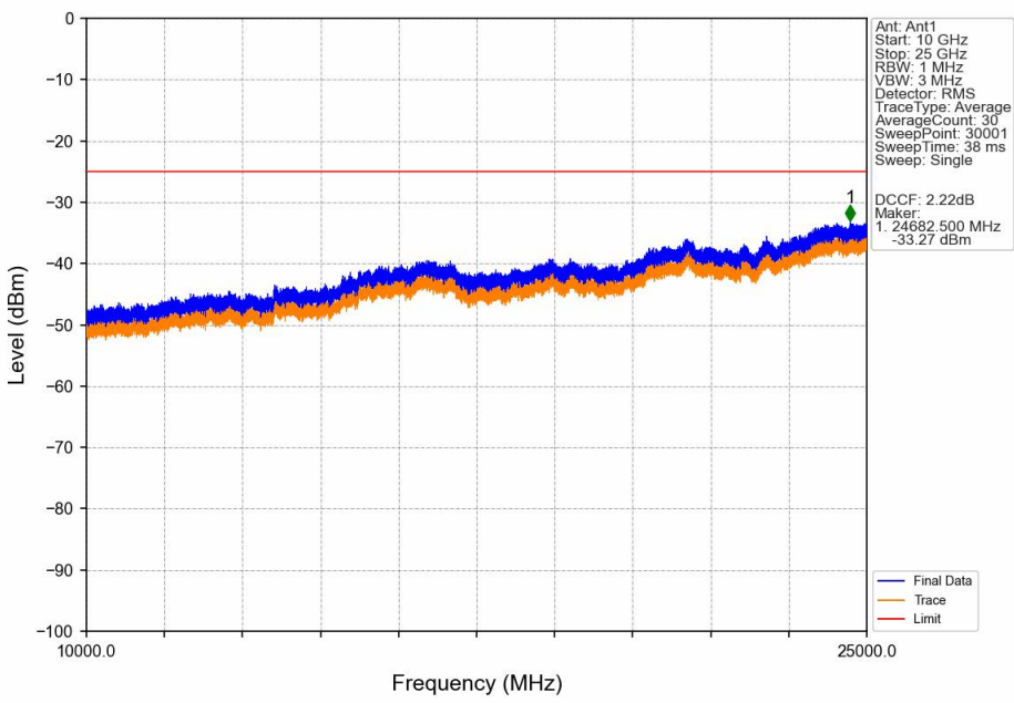
Band38_5MHz_16QAM_LCH_2572.5MHz_RB_1_0_NTNV
