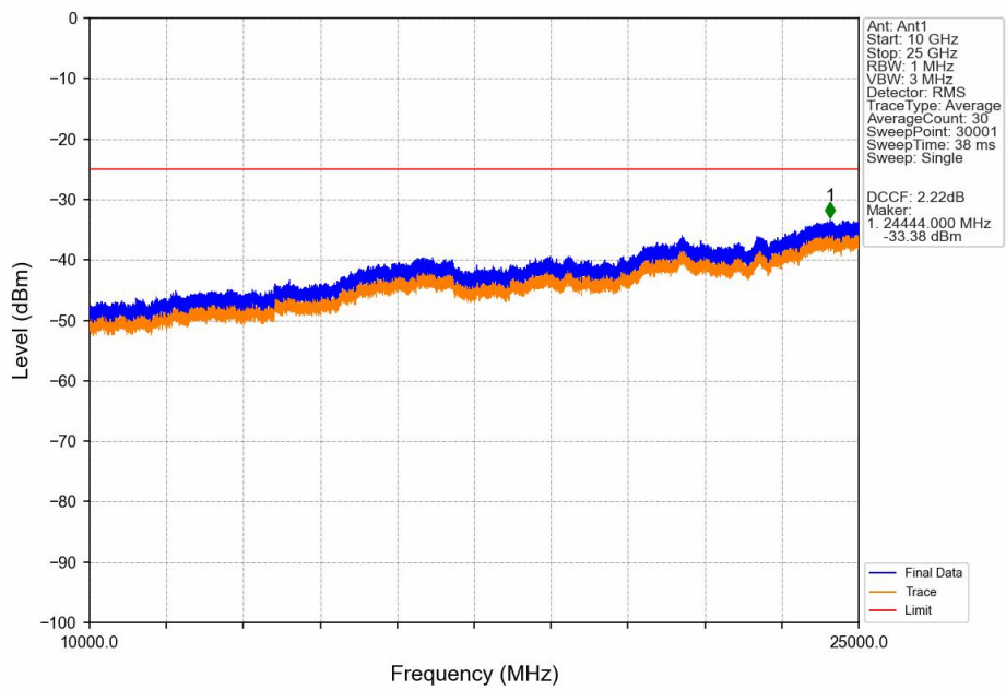
Band38_10MHz_16QAM_MCH_2595MHz_RB_1_0_NTNV
