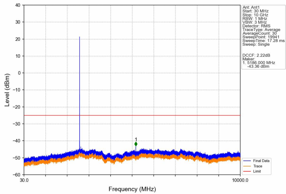
Band38_5MHz_16QAM_MCH_2595MHz_RB_1_0_NTNV
