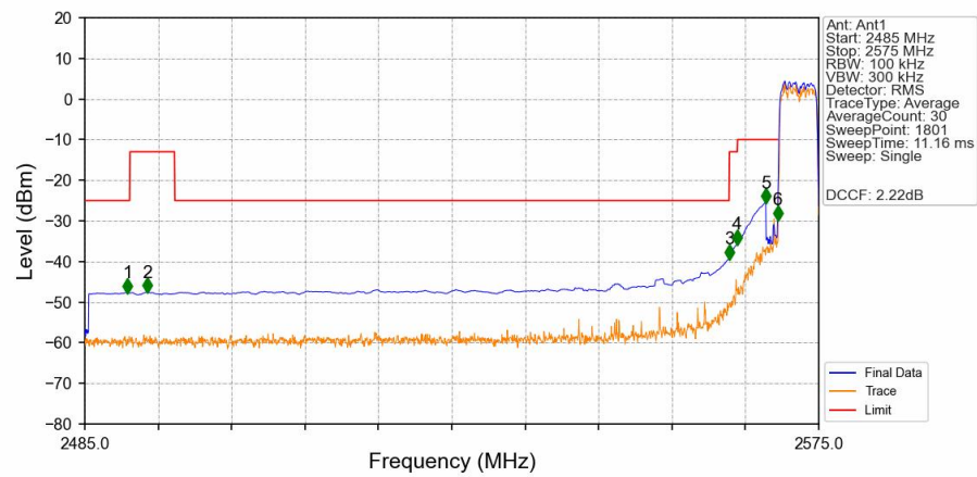
Band38_5MHz_16QAM_LCH_2572.5MHz_RB_25_0_NTNV
