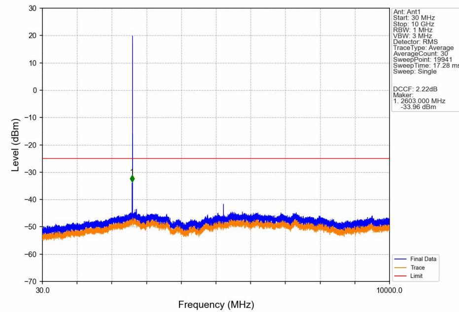
Band38_5MHz_16QAM_HCH_2617.5MHz_RB_1_0_NTNV
