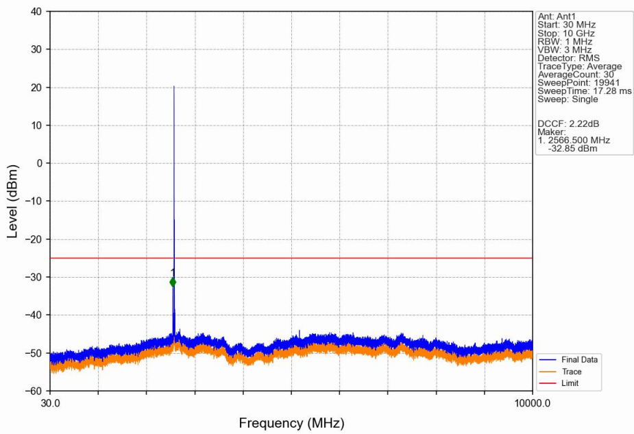
Band38_10MHz_16QAM_MCH_2595MHz_RB_1_0_NTNV
