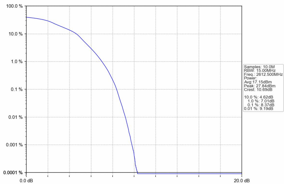
Band38_15MHz_16QAM_HCH_2612.5MHz_RB_75_0_NTNV
